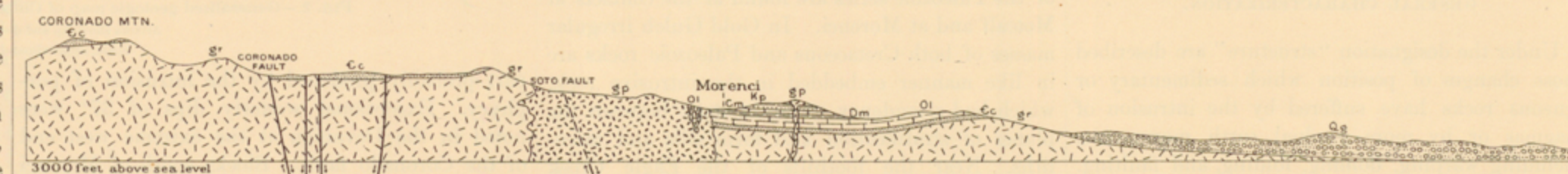
FIG. 3.—Cross section along line E-E on areal geology map.
