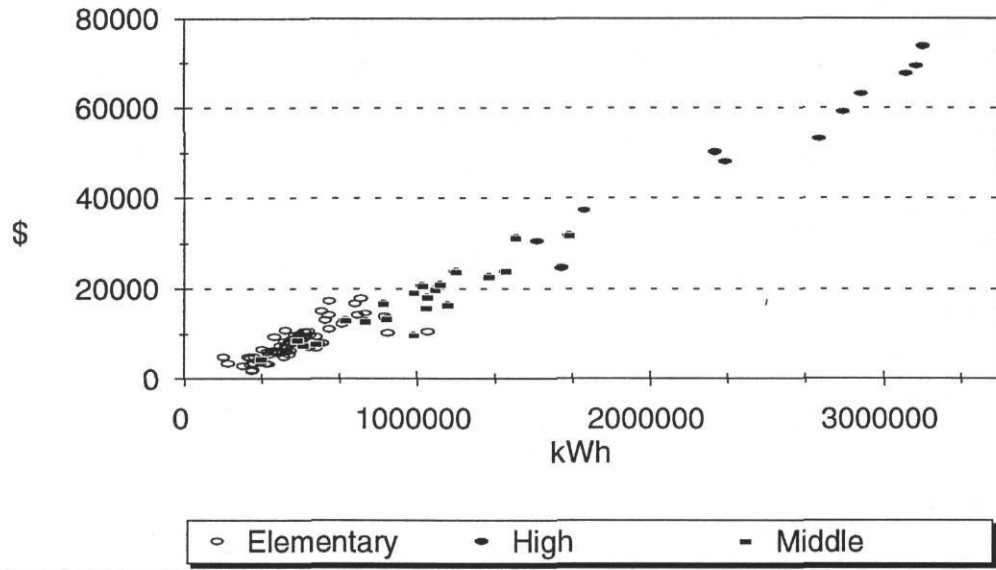
Figure 3a: The Potential Savings vs the Annual Consumption for 104 Schools
