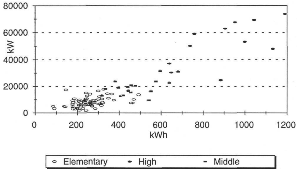
Figure 3b: The Potential Savings vs the Annual Peak Demand for 104 Schools
