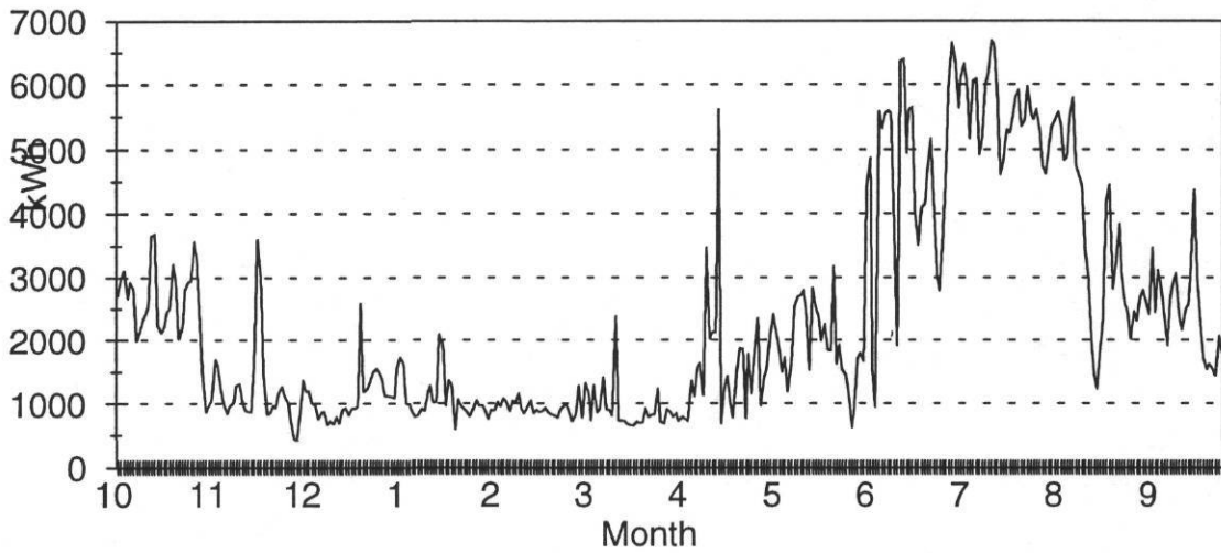
Figure A-3: The Maximum Daily Potential Electricity Savings Patterns at Dunbar Middle School
