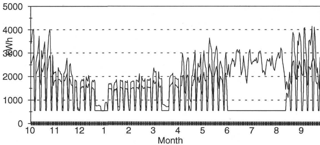
Figure A-2: The Measured and Efficient Daily Electricity Consumption Patterns at Sims Elementary School (The Top Line is the Measured Consumption, and the Lower Line is the Efficient Pattern)
