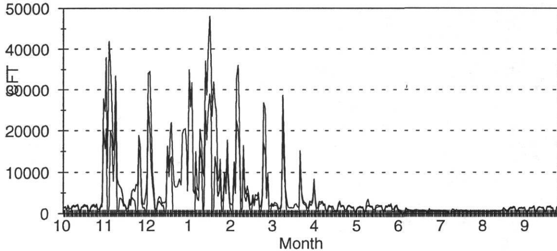
Figure A-5: The Measured and Efficient Daily Gas Consumption at Dunbar Middle School (The Top Line is the Measured Consumption and the Lower Line is the Efficient Consumption Pattern)
