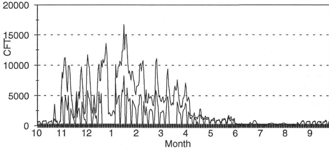
Figure A-6: The Measured and Efficient Daily Gas Consumption at Sims Elementary School (The Top Line is the Measured Consumption and the Lower Line is the Efficient Consumption Pattern)
