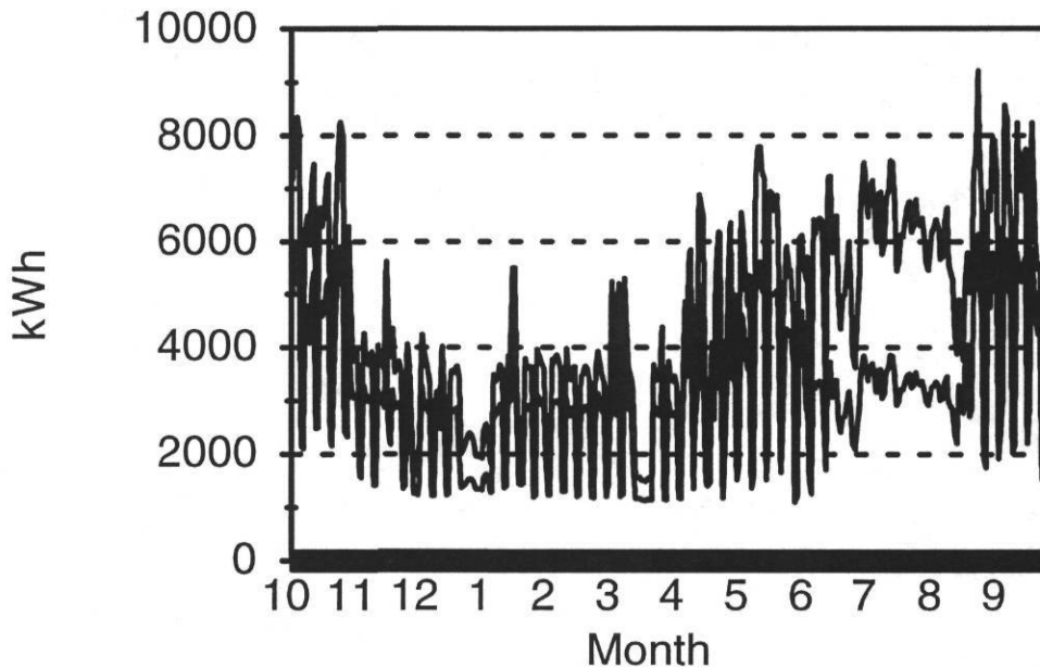
Figure 9: The Optimized and Measured Daily Electricity Consumption at Dunbar Middle School
