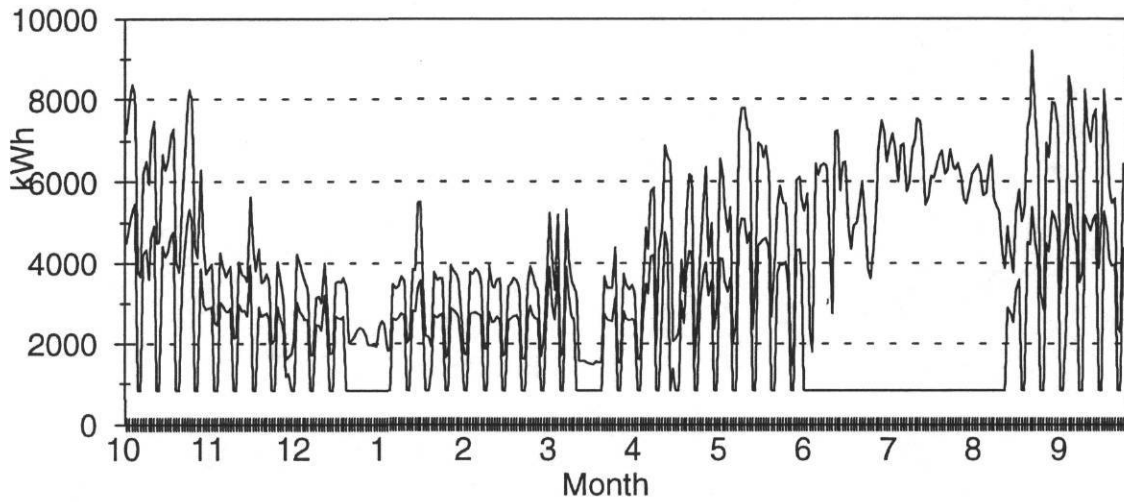
Figure A-1: The Measured and Efficient Daily Electricity Consumption Patterns at Dunbar Middle School (The Top Line is the Measured Consumption, and the Lower Line is the Efficient Pattern)
