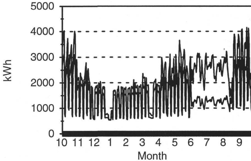
Figure 9: The Optimized and Measured Daily Electricity Consumption at Sims Elementary School
