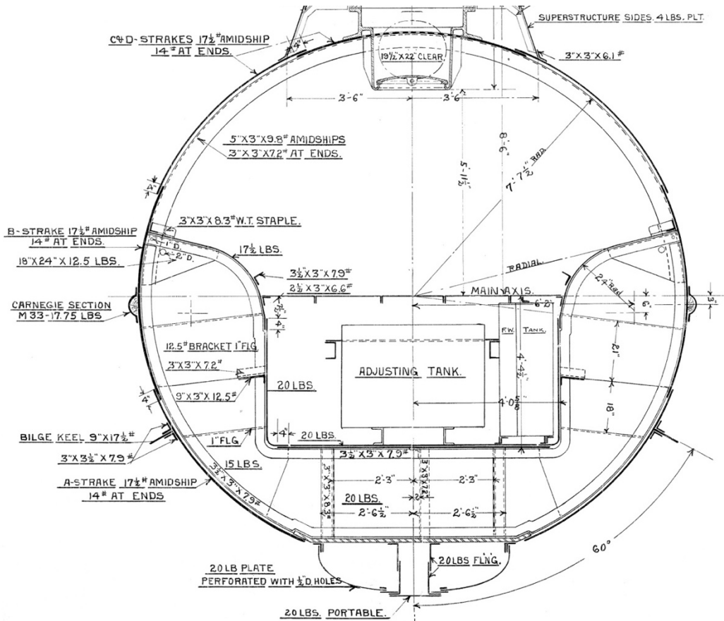
Figure 56. H-1 midships section.
