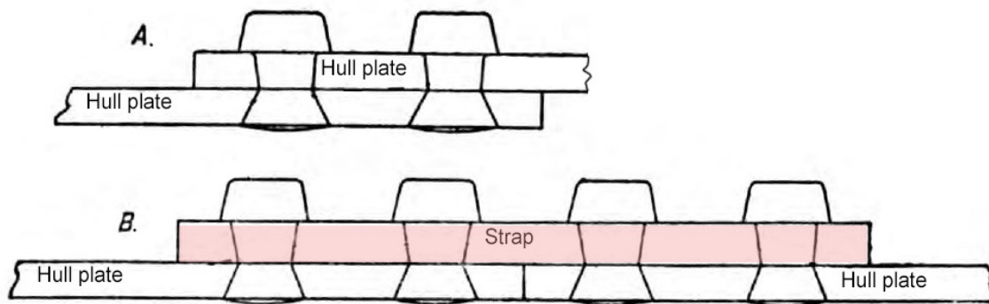
Figure 57. Butt lap and butt strap connections.
