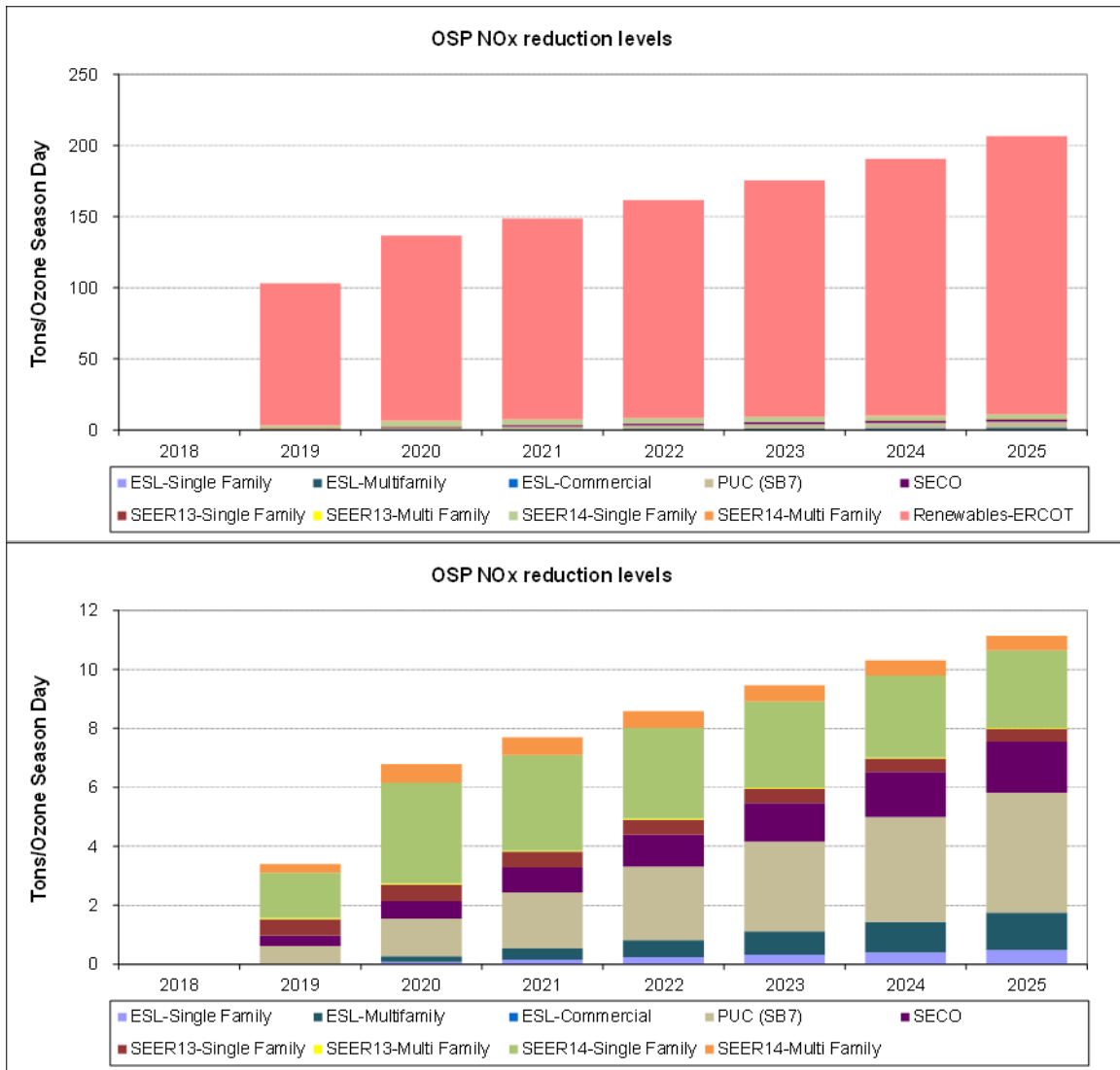
Figure 17: Integrated OSP NOx Emissions Reduction Projections from 2018 to 2025 (Base Year 2018). (Upper plot) all programs, (lower plot) all programs except Renewables.
