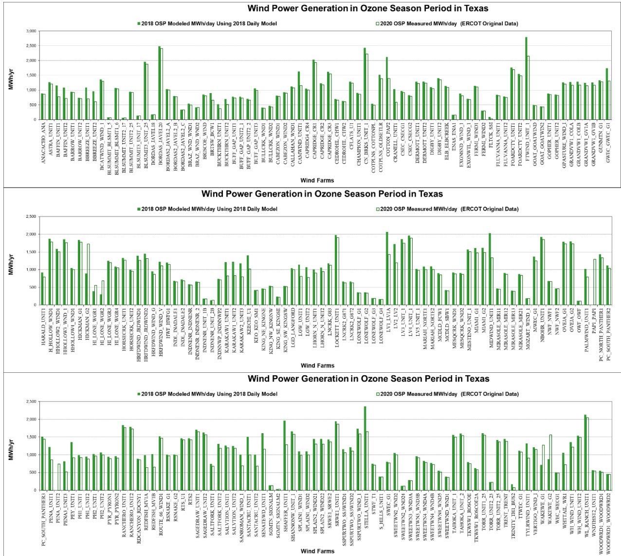
Figure 6: Comparison of 2020 OSP Measured and 2018 OSP Estimated Wind Power Production for Each Wind Farm
