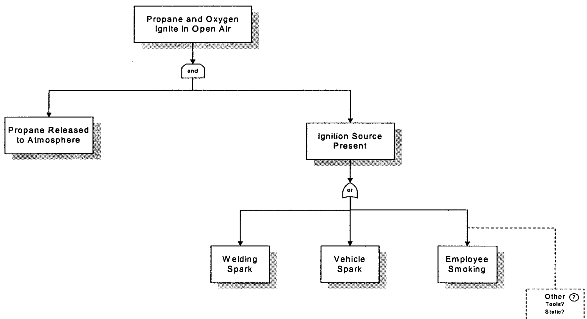
Investigative FAULT TREE Fig.1
