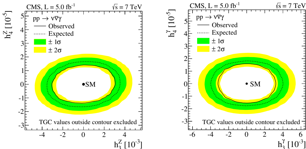
Figure 3. Two-dimensional 95% CL limits on ZZγ couplings (left) and Zγγ couplings (right).
