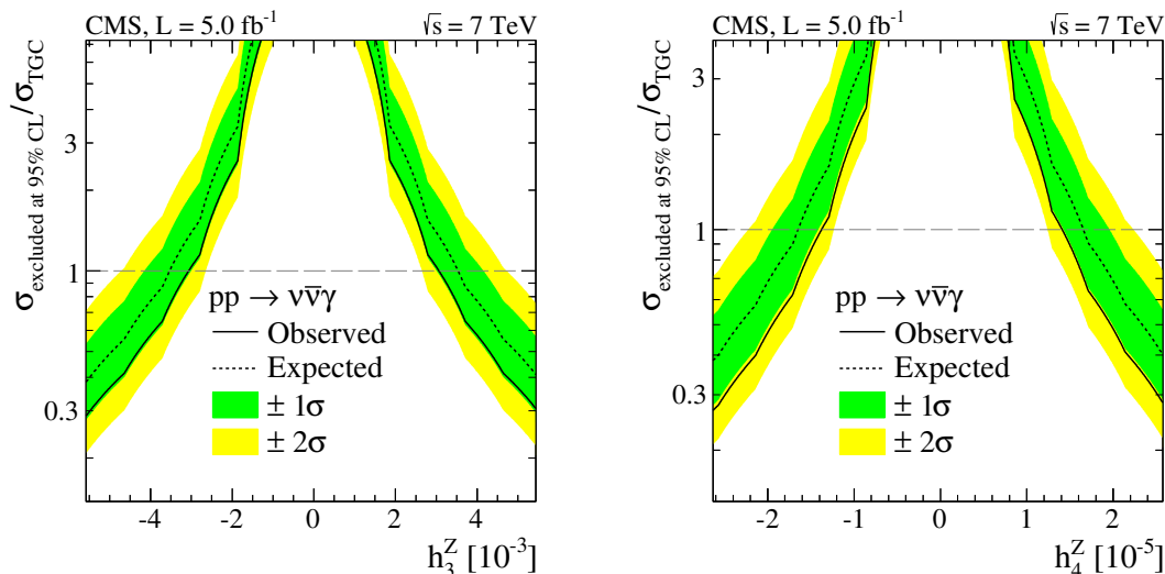
Figure 4. Cross section limits as functions of the ZZγ couplings h_3^Z (left) and h_4^Z (right). The vertical axis represents the ratio of the 95% CL upper limit on the signal contribution from anomalous couplings to the expected contribution for a given TGC hypothesis.
