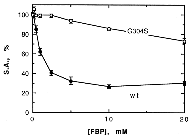
FIG. 1. FBP inhibition of wild-type (wt) and G-304-S glycerol kinases. The specific activities were determined at pH 7, 25°C, 0.44 \mu\text{g} of glycerol kinase per ml, 0.1 mM glycerol, 2 mM ATP, and the indicated concentrations of FBP as described in Materials and Methods. The results are expressed as percentages relative to the specific activities (S.A.) at 0 mM FBP of the wild-type glycerol kinase (26.9 U/mg) and the G-304-S mutant (10.4 U/mg). The values are the means for at least three determinations, and the error bars show the standard deviation.
