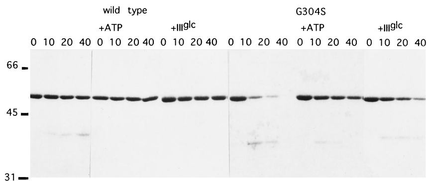
FIG. 3. Comparison of conformations of wild-type and G-304-S glycerol kinases by proteolysis. The glycerol kinases were incubated with α-chymotrypsin for the time (in minutes) indicated above each lane prior to quenching and SDS-PAGE as described in Materials and Methods. Glycerol was present at 1 mM in all digests, and ATP (2 mM) and III Glc (5.5 μM for wild-type glycerol kinase and 16.5 μM for G-304-S) were added as indicated above the lanes; 0.1 mM Zn(II) was added to the digests with III Glc . The positions of molecular weight markers (in thousands) are indicated on the left. The figure is a composite of four different gels.
