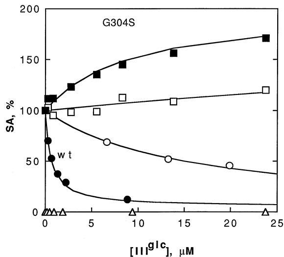
FIG. 2. III Glc inhibition of wild-type (wt) and G-304-S glycerol kinases. The specific activities were determined as described in the legend to Fig. 1, except that the glycerol concentration was 2 mM. The results are expressed as percentages relative to the specific activities (SA) at 0 III Glc of wild type (17.2 U/mg) and G-304-S (18 U/mg). Circles, wild type; squares, G-304-S; open triangles, no glycerol kinase in the assay; closed symbols indicate that 0.1 mM Zn(II) was added to the assay. The lines that are drawn through the datum points were calculated for hyperbolic binding of III Glc to the enzyme with the following dissociation constants: wild type, 15 μM; wild type + Zn(II), 0.6 μM; G-304-S, 110 μM; and G-304-S + Zn(II), 9 μM. For the calculated lines, 95% inhibition was used for the wild-type enzyme and twofold activation was used for G-304-S.
