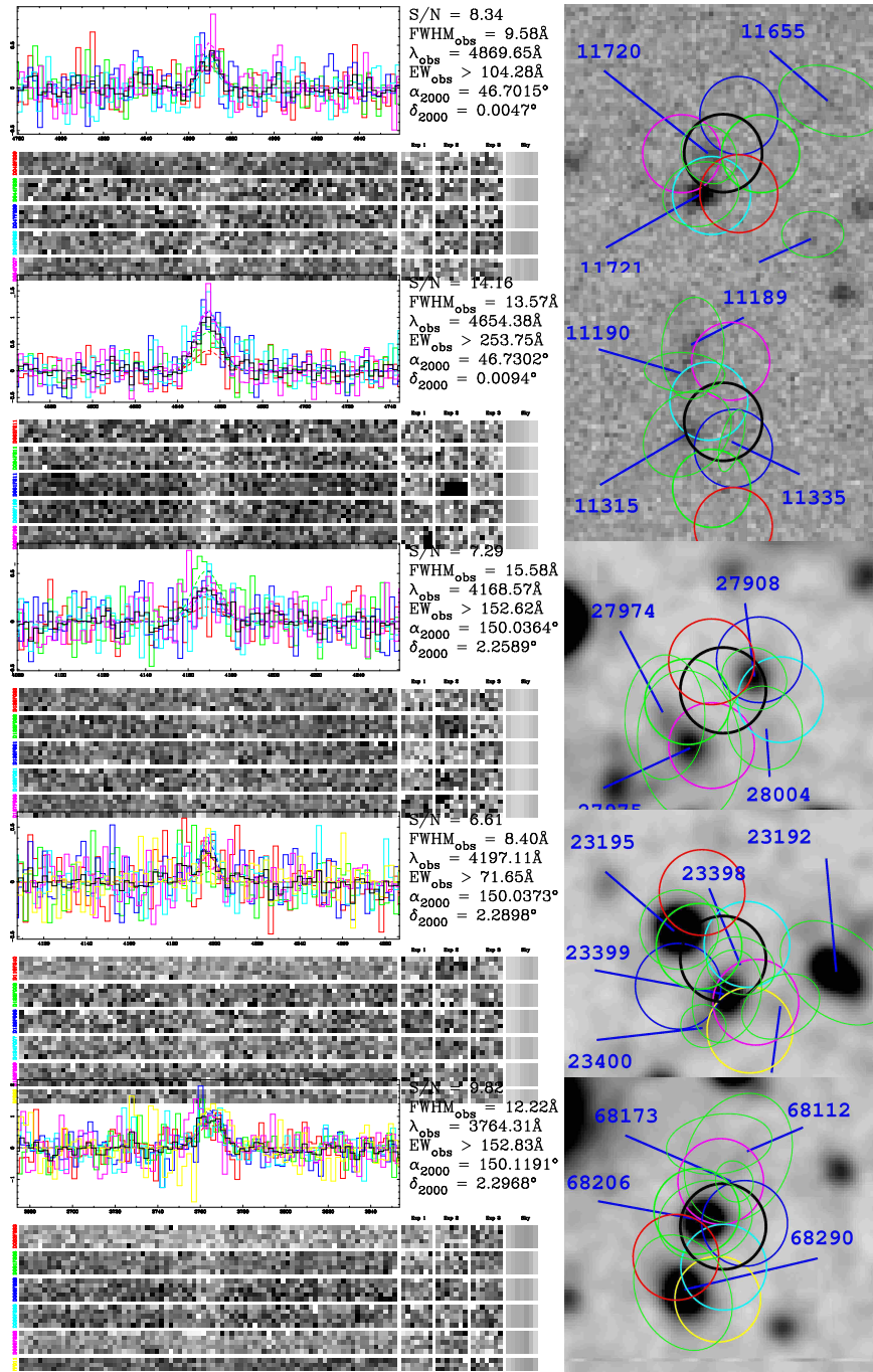
Figure 34. The five objects significantly extended in Ly \alpha . Left The spectral detections. Right The R-band images (i' for the first two MUNICS objects). First Index 99 in MUNICS. The best counterpart is #11720. Second Index 126 in MUNICS. The best counterpart is #11315. This source is also a high EW LAE. Third Index 162 in COSMOS. The best counterpart is #27975. This source has an X-ray detection. Fourth Index 164 in COSMOS. The best counterpart is #23399. Fifth Index 261 in COSMOS. The best counterpart is #68206. This source has an X-ray detection.
