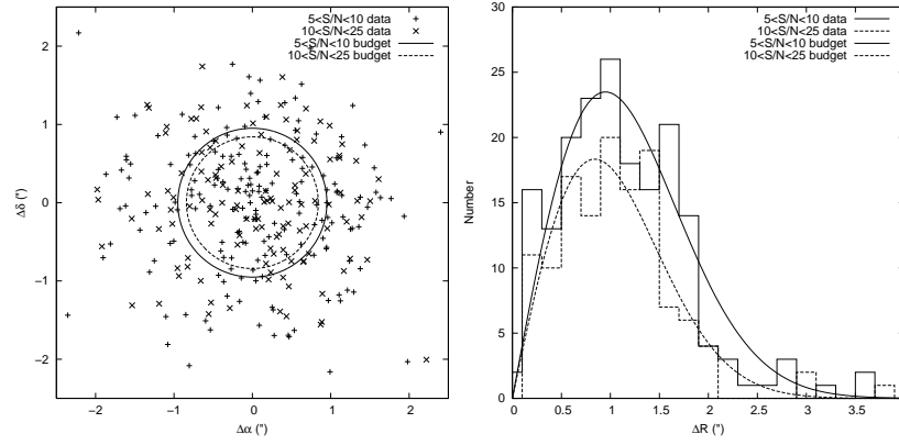
Figure 3. Left: The positional offsets from catalog emission-line detection positions and broadband counterpart image positions divided into two S/N bins. The residual correction discussed in §2.3 has been applied. The 1\sigma astrometric error budget for each bin is also drawn with radii 0''.95 for 5 < S/N < 10 and 0''.84 for 10 < S/N < 25 . Right: A histogram of the same data shown with a Rayleigh distribution. The same dispersions are used to demonstrate the appropriate characterization of the astrometric error as a two-dimensional Gaussian function.
