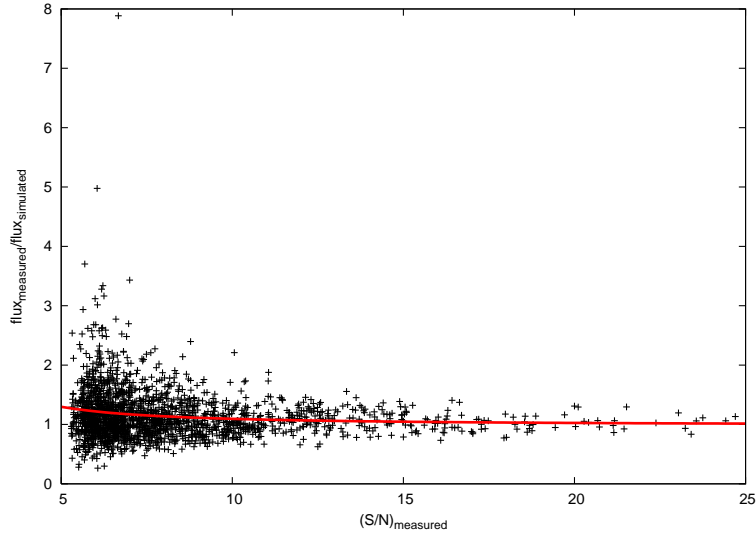
Figure 9. The ratio of measured and input fluxes from point source simulation and a least-squares fit (§4.3). The curve-of-growth method is used here to measure emission line flux. The upturn at low S/N is expected from the Eddington bias. This ratio can be applied to the LAE flux measurements of Table 3 for some applications. The average correction is fit as \text{flux}_{\text{measured}}/\text{flux}_{\text{true}} = 0.98 + 0.74/(\text{S/N})_{\text{measured}} + 4.27/(\text{S/N})_{\text{measured}}^2
