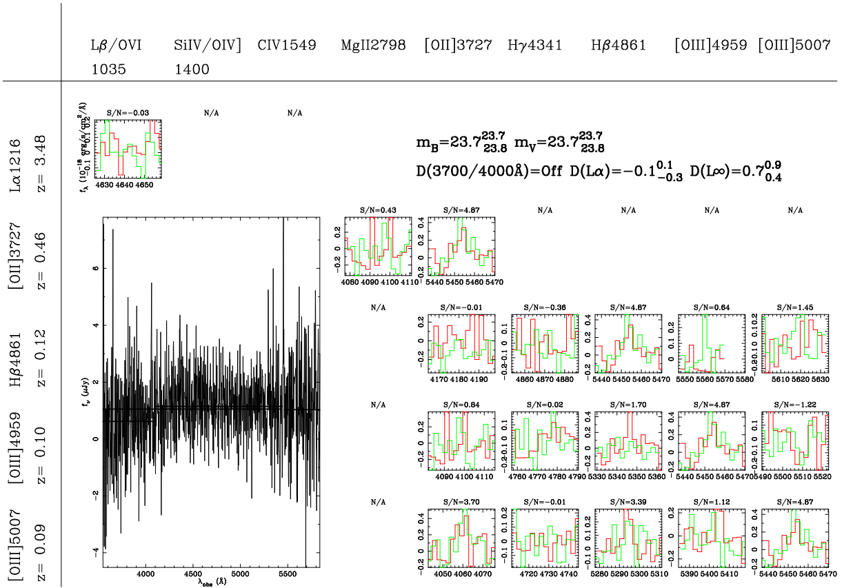
Figure 16. The automated search for multiple emission line in index 430. The format is the same as in Figure 15. This is one of the few cases where the consideration of marginally significant counterpart lines aids the classification. The primary detection is revealed to be [OIII]5007, with marginal detections in [OII] and H \beta that did not make the primary emission line catalog.
