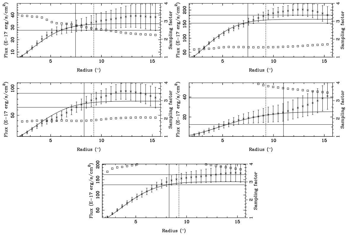
Figure 35. The curve-of-growth plots for the five significant objects extended in Ly \alpha . The format is the same as in Figure 13 and described therein. Top Left Index 99 in MUNICS. The best counterpart is #11720. Top Right Index 126 in MUNICS. The best counterpart is #11315. This source is also a high EW LAE. Middle Left Index 162 in COSMOS. The best counterpart is #27975. This source has an X-ray detection. Middle Right Index 164 in COSMOS. The best counterpart is #23399. Bottom Index 261 in COSMOS. The best counterpart is #68206. This source has an X-ray detection.
