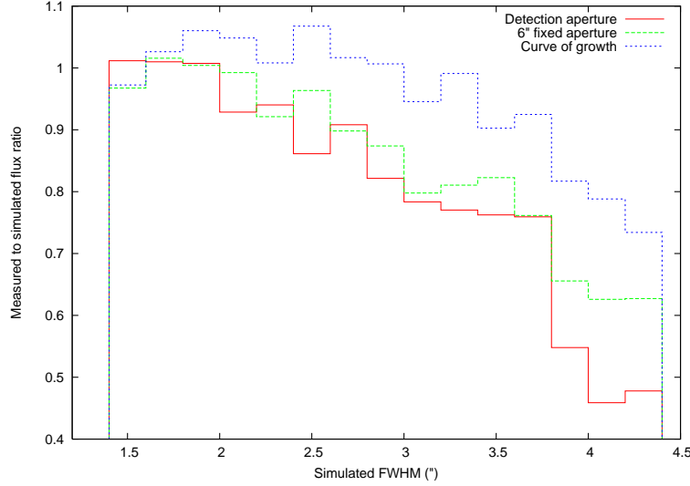
Figure 14. Binned ratios of measured and input fluxes for simulated data under a range of source sizes. The curve-of-growth flux estimator is preferred as the least biased for extended sources compared to either the detection set of fibers or a fixed radius set of fibers as the photometry aperture.
