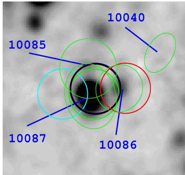
Figure 21. The ground-based, V_j imaging cutout for the Table 3 index 229. The four color circles represent fiber positions and are color coded in accordance with the spectra of Figure 20. The black circle indicates the emission line centroid. The Kron apertures from the imaging catalog are drawn as green, numbered ellipses. The best centered and brightest source is #10087 with an association likelihood of 87% and r^+ = 23.4 . The next two most likely counterparts are #10085 at 6% and r^+ = 25.1 and #10087 at 5% and r^+ = 24.9 . Either of these would also make the LAE EW cut, and it is possible that one or more LAEs at similar redshifts are jointly contributing to the emission-line flux, but this is unlikely.
