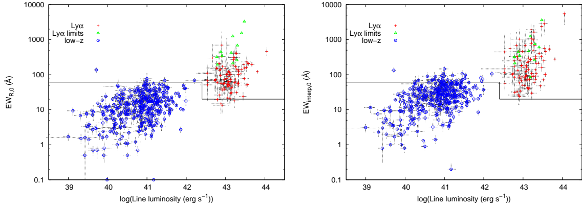
Figure 30. The distribution of rest-frame equivalent width and line luminosity for both the LAE and low- z samples. The primary classification line based on EW is drawn. The jog in the EW cut line is simply due to the cut being defined as EW_{\text{rest}} > 20\text{\AA} assuming the line to be Ly \alpha so the equivalent threshold in the [OII] restframe is 61\text{\AA} . The drawn EW cut doesn't strictly apply to the low- z objects with emission at transitions other than [OII]. A trend between higher EW and line luminosity in the LAEs is somewhat visible but noisy over this survey's dynamic range. The same trend is seen in surveys with lower flux limits and discussed in Cassata et al. (2010). Left Continuum estimated only from the R -band photometry (or the i' -band in MUNICS). Right Continuum estimated from interpolation with the two nearest filters bounding each emission line's wavelength.
