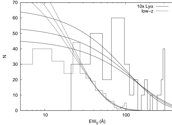
Figure 31. The distribution of rest frame equivalent width for values with S/N > 3 for both the LAE and low- z sample by interpolating from the bounding broadband data. The LAE histogram has been scaled by 10\times for visual clarity. A maximum likelihood fit was made by taking EW_{\text{rest}} > 20\text{\AA} where the samples should be complete. An exponential scale length of 128 \pm 20\text{\AA} fits the LAE distribution and 22 \pm 1.6\text{\AA} fits the [OII] distribution. The exponential fits and error ranges are also plotted. The largest plotted bins contain all values that lie higher than the histogram range.
