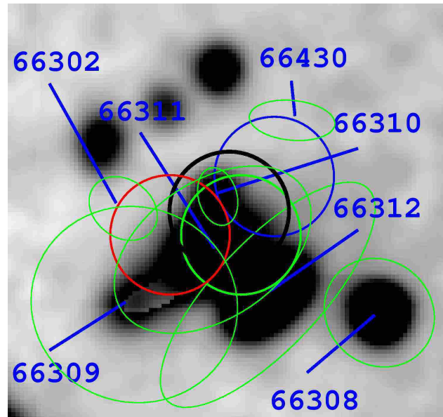
Figure 27. The ground-based, V_j imaging cutout for the Table 3 index 322. The detection spectra are given in Figure 26. The format is the same as in Figure 21. The counterpart #66311 at r^+ = 21.1 has a 84% likelihood in association. The counterpart #66312 is already assigned to the VIRUS-P detection of Table 3 index 310 at \lambda_{\text{obs}} = 4948.2\text{\AA} . The counterpart #66310 at r^+ = 24.9 would be a LAE based on EW and looks like a reasonable candidate system resolved from #66311 in the HST image, but it only holds a 6% chance of association. This source is associated to #66311 as an [OII] emitter in the catalog.
