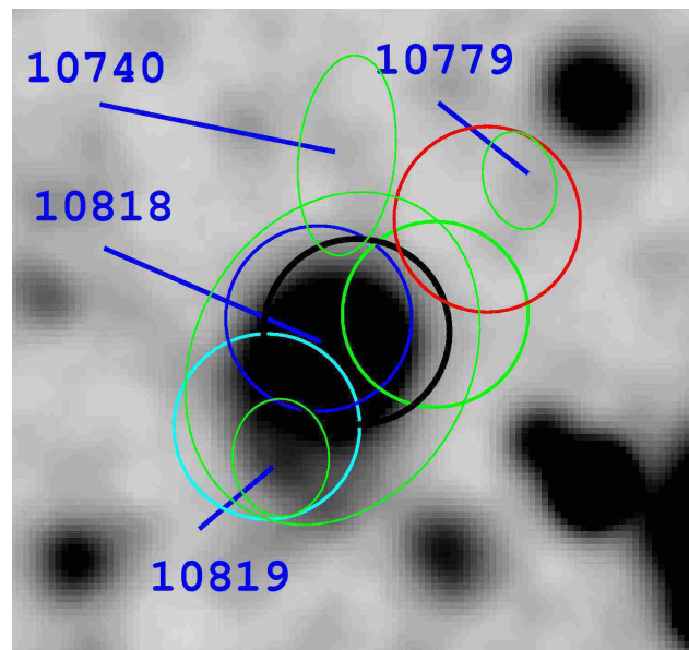
Figure 24. The ground-based, V_j imaging cutout for the Table 3 index 308. The detection spectra are given in Figure 23. The format is the same as in Figure 21. The counterpart #10818 at r^+ = 22.1 has a 99.5% likelihood of being associated. The observed EW of 30.9_{-9.5}^{+14.9}\text{\AA} leads to a firm low- z classification, presumably for [OII].
