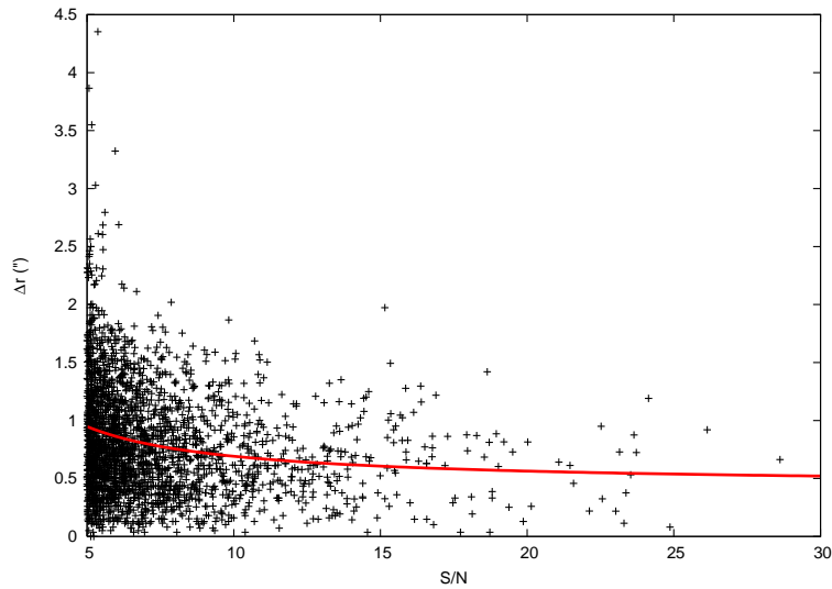
Figure 11. The distribution of simulated source positional errors under VIRUS-P sampling patterns with a fit to the dispersion as a function of measured S/N. The maximum likelihood fit to the peak of a Rayleigh distribution gives \sigma = 0''.348 + 2''.04/(S/N) .
