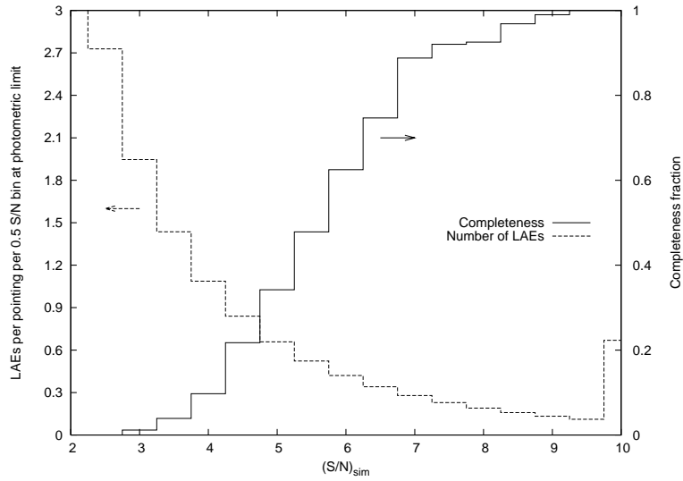
Figure 10. The survey's catalog completeness function for multiples of the flux limit. When combined, this function, the survey's photometric wavelength-based flux limit in Figure 2, and the actual mosaic pattern with photometric calibration in Figure 6 define the limits necessary for volume and luminosity function calculation (Blanc et al. 2010).
