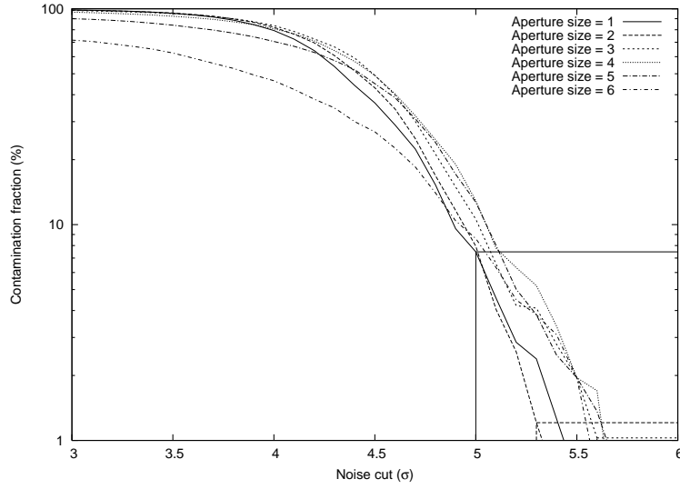
Figure 8. The fractional contamination to the LAE sample by S/N cut. The detection method used is described in detail in §4.1. The LAE predictions are the same as in §2.4. Curves are given for differently sized collections of neighboring fibers. The growth of apertures was allowed whenever the S/N was increased by > 0.3 with the inclusion of another fiber. At a high, constant S/N, the greatest contamination is produced by large apertures. The optimum sized aperture for a point source under all dither-source geometries is two at median. To optimize our selection, we make a staggered series of S/N cuts based on the number of fibers used, N , as S/N > 5.0 + 0.3 \times (N - 1) . The horizontal and vertical lines show the evaluation points of this cut to the simulation curves. This procedure predicts 10\% \pm 1.6\% noise contamination.
