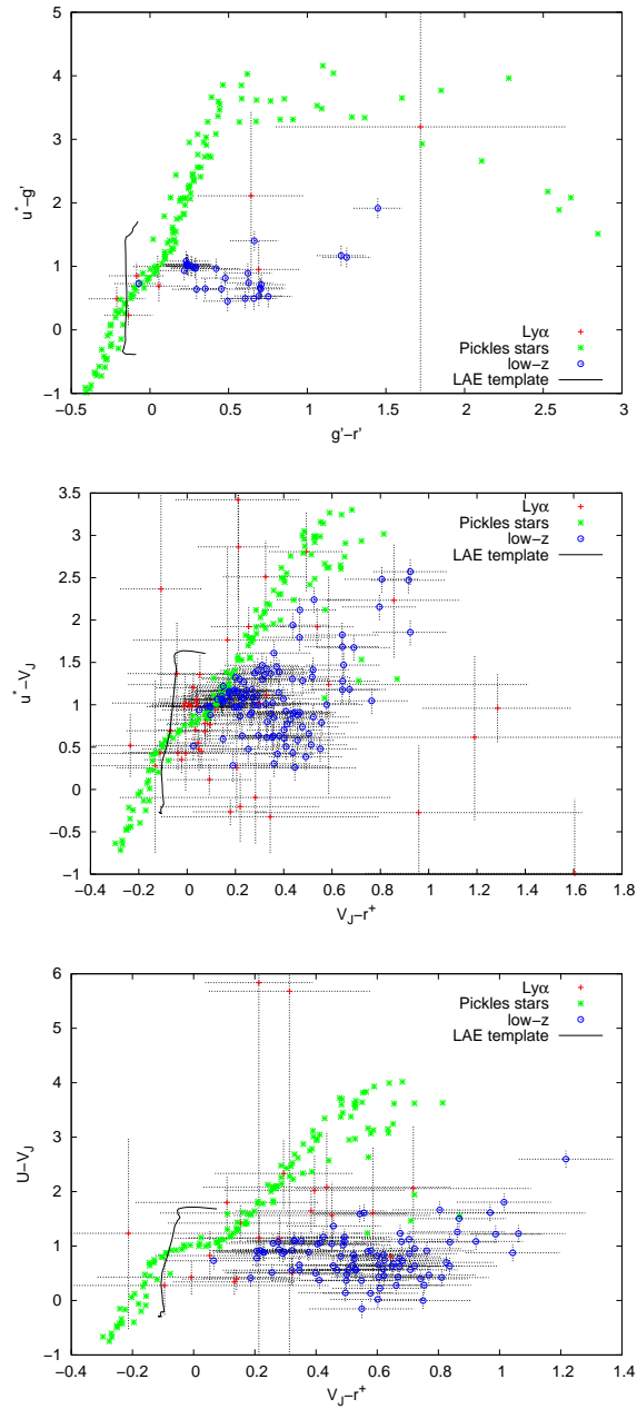
Figure 33. Color-color plots in the photometry bands that commonly define the Lyman Break Galaxy selection. Detections are not shown for the MUNICS field where we lack U -band data. The LBG selection rules are sensitive to the exact filter and telescope choice, so we do not transform these filter data into systems with published LBG rules. Instead, we synthesize colors of the Gawiser et al. (2007) LAE template as the solid, black curve for 1.3 < z < 4.5 and stars (Pickles 1998). Albeit with some exceptions and frequently large color errors, the LAE sample is segregated from the low- z objects and lies where expected. Top XMM-LSS objects, Middle COSMOS objects, and Bottom GOODS-N objects.
