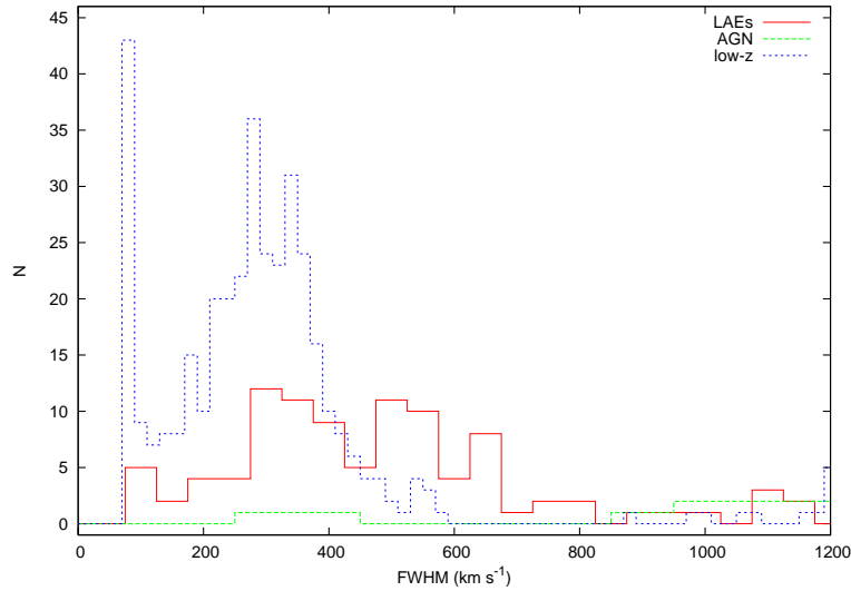
Figure 19. The line width distributions for all survey objects. We have subtracted an instrumental resolution of 300 \text{ km s}^{-1} in quadrature. There is significant overlap between all populations making width-based classification impossible. No attempts have been made here to deconvolve the blended [OII] doublet. The low- z objects are generally contained to low widths, but the LAE distribution overlaps heavily with both the AGN and low- z distributions.
