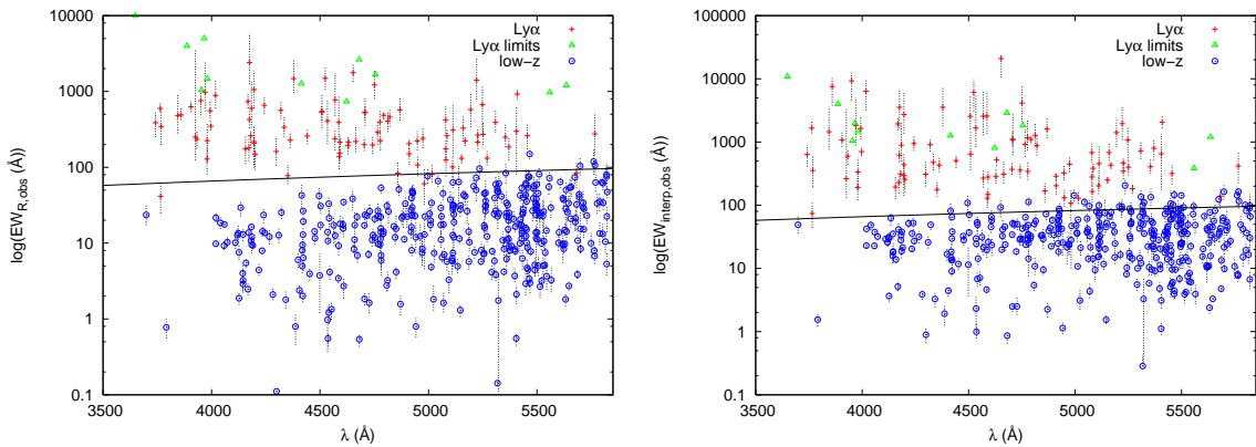
Figure 17. The distribution of observed wavelength and observed EW. The line marks the usual EW cut used in narrowband imaging and adopted here. Exceptions to the EW selection are discussed in §5.2. Left Continuum estimated only from the R -band photometry (or the i' -band in MUNICS). Right Continuum estimated from interpolation with the two nearest filters bounding each emission line's wavelength.
