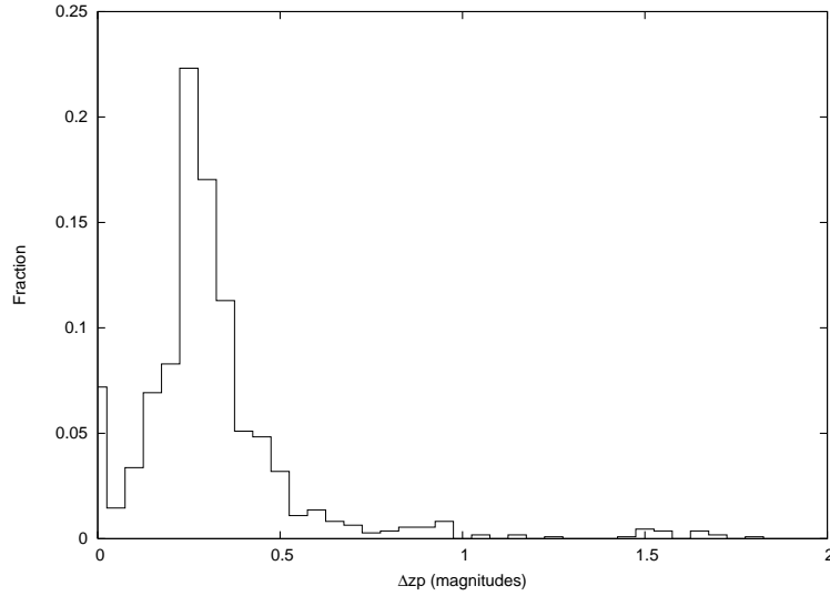
Figure 4. The distribution of zeropoint offsets due to non-photometric transparency as measured with the guider camera. This distribution represents the best 60 th percentile of the observing allocation with the remaining 40% being too poor to guide or requiring dome closure.
