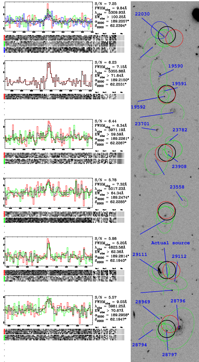
Figure 29. The spectral detection and HST ACS F606W (Giavalisco et al. 2004) cutouts for the final six of twelve new, high- z redshift measurements in GOODS-N. From top to bottom, the objects are indices 415, 426, 434, 447, 467, and 474 in Table 4. The object with index 467 does not have an identified counterpart in the ground-based images due to blending, although a likely counterpart is identified in the HST data. The best counterparts for the remaining five, in order of listing, are 22030, 19592, 23908, 23670, and 28797.
