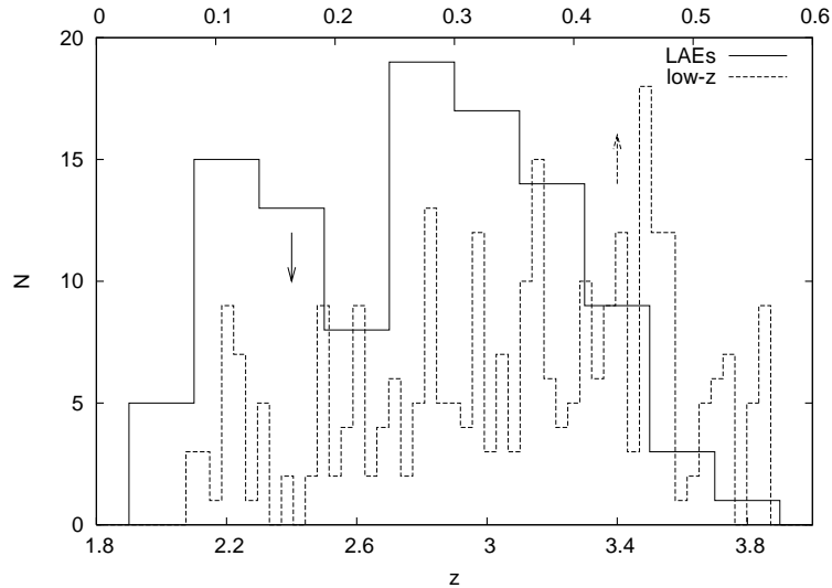
Figure 32. The distribution in redshift for all the survey objects. The upper axis labels apply to the low- z sample and the lower axis labels to the LAE sample. Each significantly overdense low- z bin is primarily contained in one survey field. The overdensities may be early indicators of groups or clusters, but the low number statistics preclude firm classification. There are no clusters from the Koester et al. (2007b) catalog in any of this pilot survey's area.
