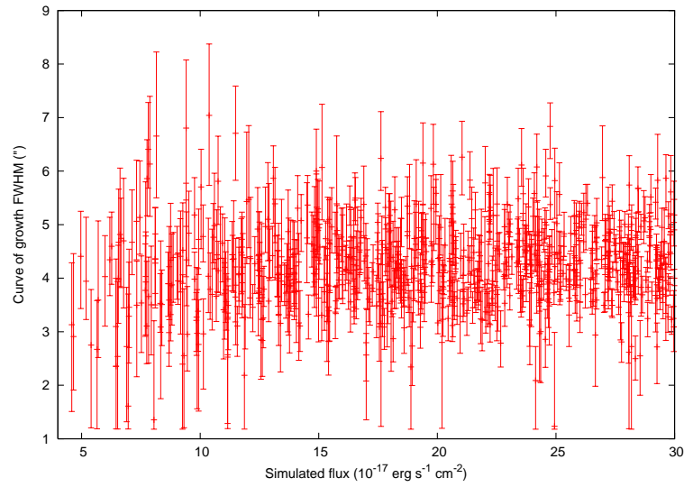
Figure 12. The distribution of measured source sizes in simulated data. The simulation input source sizes were drawn from the survey seeing distribution. The large fiber sizes set a large resolution threshold. Based on the 99.7% confidence interval, we only claim significantly resolved measurements for curve-of-growth FWHM sizes > 6.81'' .
