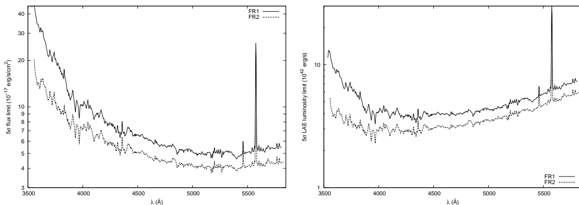
Figure 2. Left The 5\sigma detection limit under photometric conditions for an emission-line object perfectly centered in a fiber in three 20 minute exposures. Different source positions can improve or decrease this limit by \sim 15\% which is captured in our completeness calculation. In both figures, curves are given for the two focal reducers, FR1 and FR2. Right The 5\sigma luminosity limit under photometric conditions for objects detected in the Ly \alpha line.
