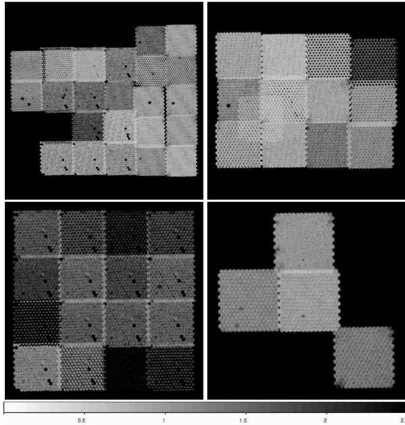
Figure 6. Sensitivity maps ( 1\sigma per detection element) at 4500\text{\AA} in 10^{-17} \text{ erg s}^{-1} \text{ cm}^{-2} . The three broken fibers in fiber bundle IFU-1 are evident. Top left: COSMOS, Top right: GOODS-N, Bottom left: MUNICS, Bottom right: XMM-LSS.
