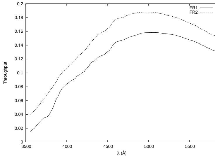
Figure 5. The total system throughput of VIRUS-P, the 2.7m telescope, and the atmosphere at an airmass of one. Curves are given for the two eras of focal reducers, FR1 and FR2.
