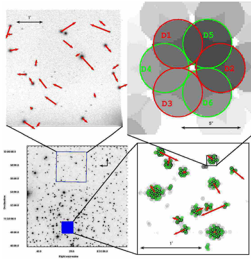
Figure 1. The layout of a VIRUS-P observation and the quality of a guider-based astrometric solution. Bottom left: The footprints of the spectroscopic science FOV and the northerly offset guider FOV overlaid on a Digital Sky Survey (DSS) image of the open cluster M67. This type of field is used to calibrate the astrometry of the guider and the fibers as discussed in §2.3. Top left: An expanded view of the VIRUS-P guider field with residuals from the astrometric model. The residuals are shown as red vectors scaled by 60\times . The rms is 0''.42 . Bottom right: An expanded view of the science FOV. The continuum map is generated from the IFS data summed over 4100\text{\AA} < \lambda < 5700\text{\AA} . Fibers that have significant flux and border other significant fibers are highlighted with green circles and bunched as point source detections for the astrometric fit. The residuals are shown as red vectors scaled by 60\times . The residuals in the IFU are less than the residuals in the guider as both fields have a similar number of degrees of freedom, but the guider has more datapoints. Top right: The expanded view of one fiber moving through the six dither positions. The pattern, marked with D1-D6, gives very nearly an oversampling of two. The small offsets necessary to complete the dither patterns are controlled by sending offsets to the guider.
