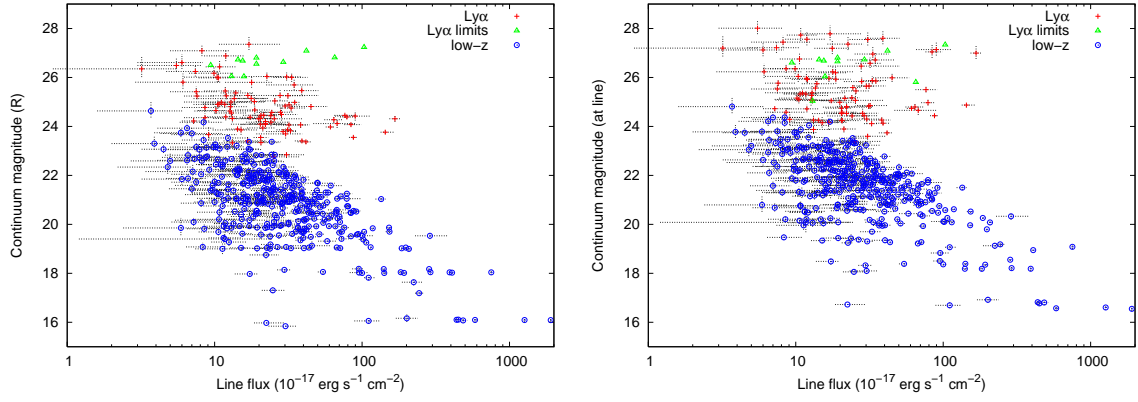
Figure 18. The distribution of emission line flux and broadband magnitude. Left Continuum estimated only from the R -band photometry (or the i '-band in MUNICS). Right Continuum estimated from interpolation with the two nearest filters bounding each emission line's wavelength.
