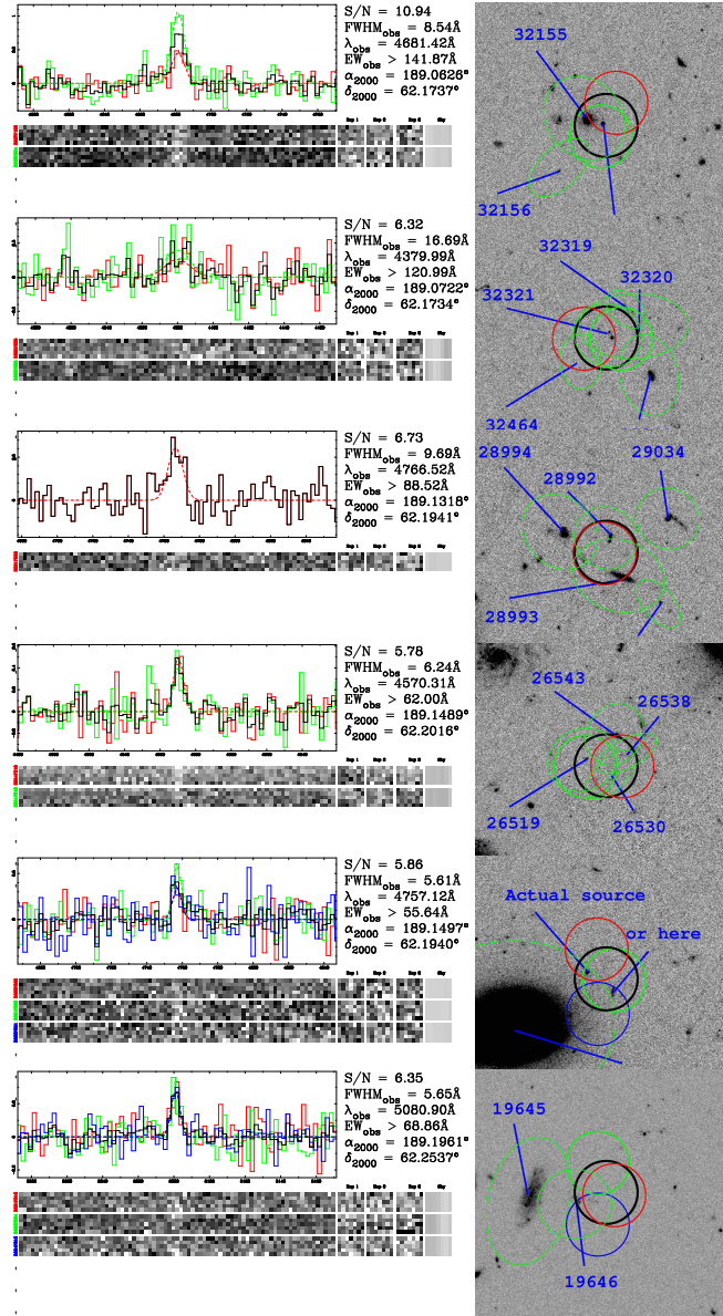
Figure 28. The spectral detection and HST ACS F606W (Giavalisco et al. 2004) cutouts for six of the twelve new, high- z redshift measurements in GOODS-N. From top to bottom, the objects are indices 334, 338, 360, 372, 373, and 403 in Table 4. The first and fifth objects do not have identified counterparts in the ground-based images due to blending, although likely counterparts are identified in the HST data. The best counterparts for the second, third, fourth, and sixth objects are #'s 32321, 28992, 26519, and 19646.
