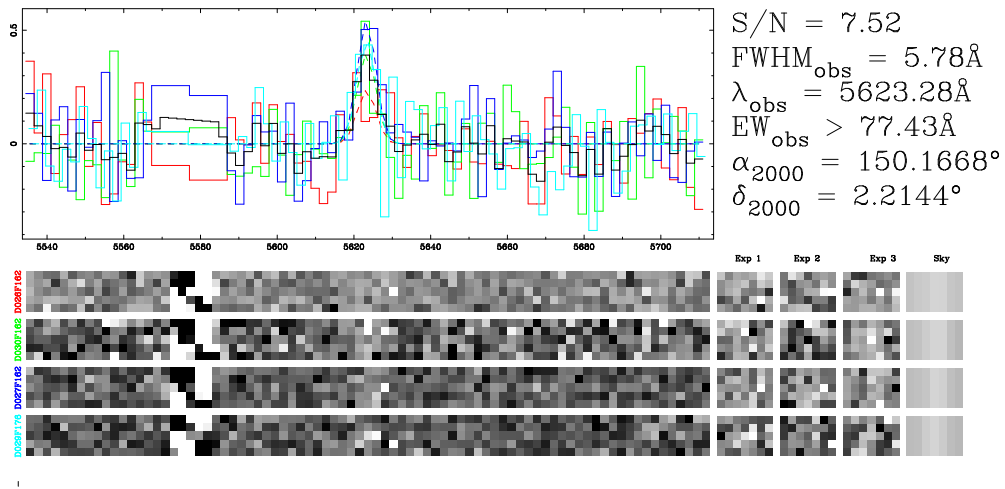
Figure 23. The emission-line source detection for index 308 which lies in the COSMOS field. The format is the same as in Figure 20. The spectrum-based EW does not go deep enough to discriminate between the classifications. This source neither shows alternate emission lines nor has an X-ray counterpart.
