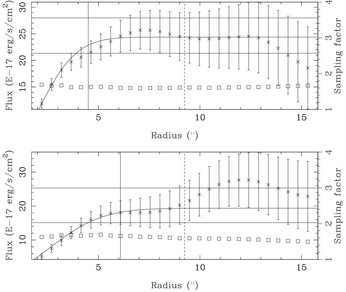
Figure 13. The data, fits, and final evaluation for the curve of growth line flux measurements of a LAE ( top ) and an [OII] emitter ( bottom ). In both, the open square symbols display the cumulative sampling factor on the right hand scale. The sampling factor is written in Equation 3 as N(\Delta r < r_{fib}, r, \theta) and is the average number of fibers overlaying the surface enclosed in radius r . The points with errors show the estimated cumulative flux on the left hand scale. The vertical dotted lines mark where the fit is truncated. This threshold has been selected with consideration towards being significantly larger than the widest objects found and small enough to limit unnecessary noise. The vertical solid line marks the radius to the fit where 90% of the flux is enclosed. The horizontal solid lines show the 1\sigma confidence of the fit's normalization. The top fit returns a total flux of 24^{+3.6}_{-3.0} \times 10^{-17} \text{ erg s}^{-1} \text{ cm}^{-2} . The bottom fit returns a total flux of 19^{+6.0}_{-4.3} \times 10^{-17} \text{ erg s}^{-1} \text{ cm}^{-2} . The errors are correlated on the displayed scale, but the Monte Carlo fit varies the data from each fiber independently to generate proper errors.
