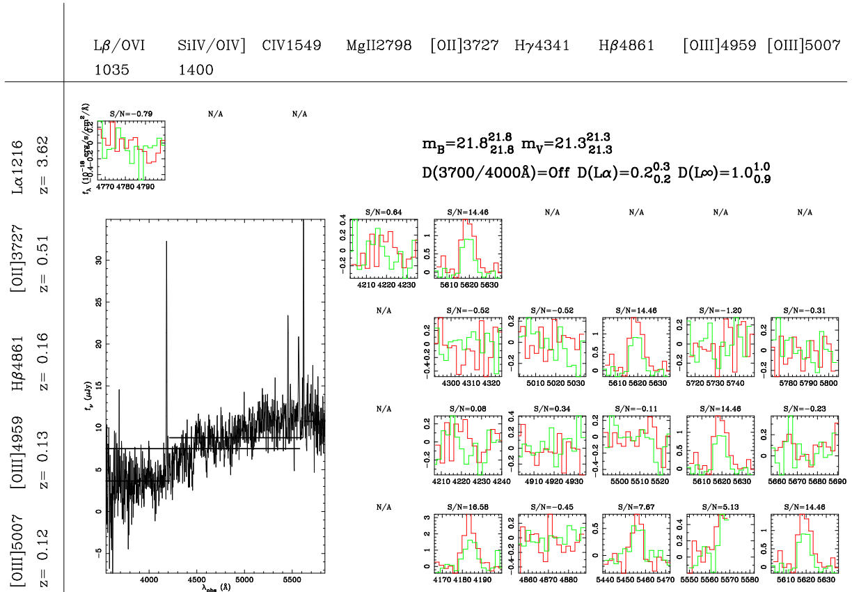
Figure 15. The attempts to find matching lines to an [OIII]5007 detection in index 323 of Table 3. The detection is formed from two fibers represented independently with the red and green lines. The leftmost column shows the prospective identifications of our originally detected line at 5619Å. For each prospective identification, we attempt fits to the emission-line possibilities in the top row. In this case, matches to [OII] and H \beta both give a clear identification. The [OIII]4959 is detected but overlapping with the mask around 5577Å. This technique only rarely gives positive evidence for Ly \alpha classification by ruling out low- z emission line combinations because our wavelength bandpass is not much larger than common bright optical emission-line spacings. However, is often useful in classifying transitions between low redshift options as in this case. The full spectrum is shown in the large window to the left. Various continuum regions are evaluated by assuming the primary emission line to be Ly \alpha and [OII] shown by the horizontal lines. The continuum fits are used to look for various breaks as calculated in the upper right. This galaxy is also identified by significant detections of H \beta , [OIII]4959, and [OII] in entries 325, 326, and 327 of Table 3.
