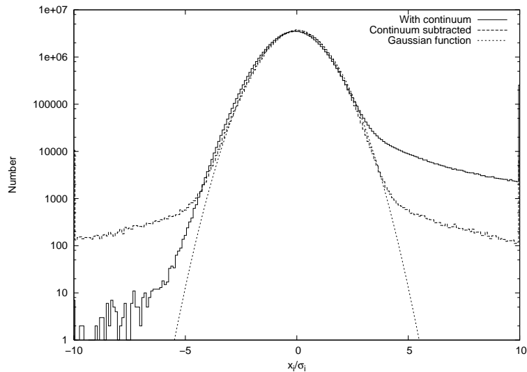
Figure 7. A histogram of the ratio between the reduced data and error for all 87.8M independent spectral elements in this survey. Most elements only see the sky background with residuals consistent to a normally distribution noise model. A small but obvious fraction of the elements also see bright, positive signal from continuum sources. The normalized Gaussian function shows the expected distribution in the absence of signal and systematics. The influence of the fiber throughput systematic (§3.6) likely broadens the distribution. This is most evident on the negative side which becomes nearer the normal distribution after background subtraction. The distribution after continuum subtraction appears much more symmetric and with a better matching width. The data wings at high and low ends represent the fiber positions with strong continuum. The boxcar-based continuum fitting is a rather crude tool that does not characterize all the continuum signal, but the emission line catalog is uncompromised by its use.
