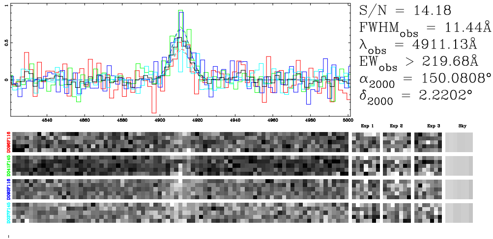
Figure 20. The VIRUS-P emission-line detection image for index 229 which lies in the COSMOS field. This object is undoubtedly a real detection with one of the largest S/N ratios we find for any high- z object. In this case, the aperture is grown to include four fibers. The four rows in the Figure's bottom half show the spectra from the four detection fibers. The right side, square cut-outs show the spectra from individual 20-minute exposures and the sky model. The three exposures in each fiber are then biweight combined into the two-dimensional, bottom-left spectra and the one-dimensional spectra in the upper-left line plot. The collapsed, one-dimensional spectra are color-coded by fiber number. The Gaussian fits to each fiber are given by dotted curves. For visual clarity, the spectra are resampled and stacked into the black histogram. Continuum is not detected within a 200\text{\AA} boxcar around the line, and the high level of flux permits the Ly \alpha classification from the spectrum alone in this rare case. The tabulated EW instead is based on the flux density of the imaging counterpart. The quoted central wavelength in this figure has not yet had the heliocentric and vacuum corrections applied as is done with the tabulated values.
