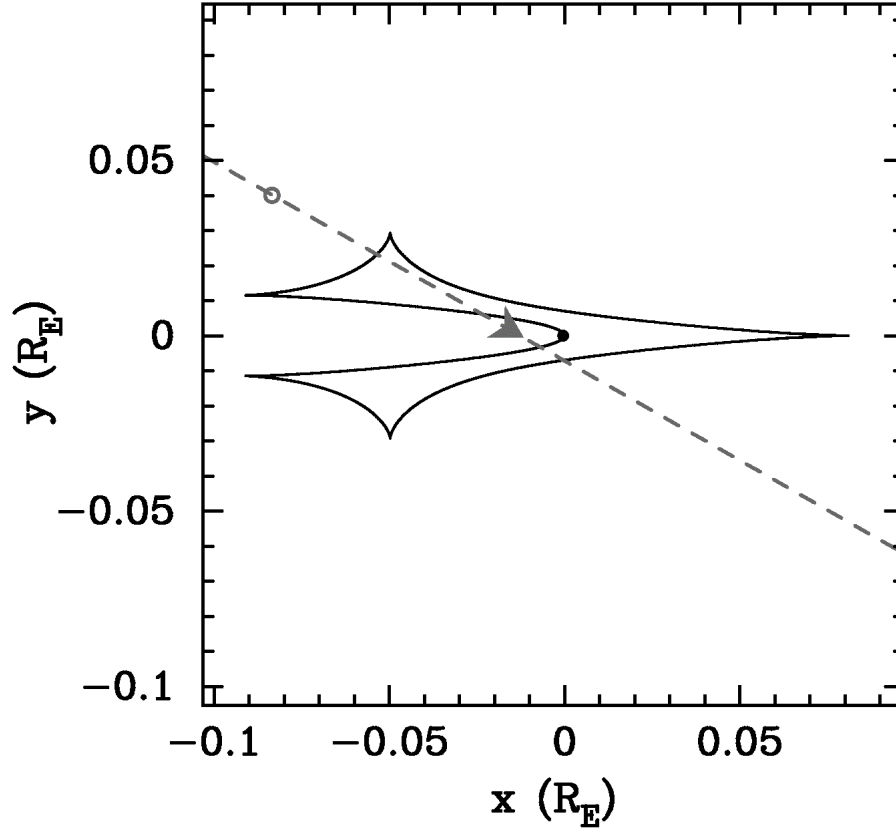
Fig. 2.— The caustic is plotted in solid curve for the MOA-2009-BLG-319 best fit model, and the dash line indicates the source star trajectory. The circle represents the source star size. The source star crosses the caustic curve four times, with peak magnification of A_{\max} \sim 205 during the third caustic crossing at \text{HJD}' \sim 5006.96 .
