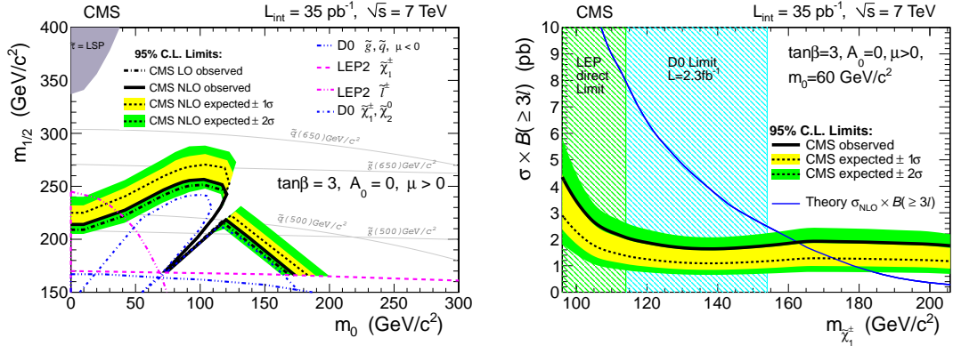
Figure 5: Left: excluded region for the mSUGRA/CMSSM scenario along with the limits from the multilepton searches from the Tevatron [8] and the exclusion derived from slepton and chargino limits from LEP [36–41]. The region below the lines is excluded at 95% CL. Right: the expected cross section times branching ratio \sigma \times B(3\ell) as a function of the chargino mass. The theoretical curve crosses the observed 95% CL upper limit on the cross section at 163 \text{ GeV}/c^2 , thus excluding charginos below this mass for these values of the other parameters. For comparison the regions excluded by LEP (from slepton limits [36–41]), Tevatron chargino-neutralino production [8], and Tevatron squark-gluino production [42] are indicated as well. This and other results have the other MSSM parameters fixed at \tan\beta = 3, A_0 = 0 , and \mu > 0 except [42], which uses \mu < 0 .
