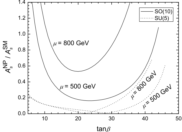
Figure 3: The possible SUSY contributions are plotted as a function of \tan \beta when the \tau \rightarrow \mu \gamma bound is saturated. The SO(10) boundary condition can give a larger SUSY contribution than the SU(5) boundary condition. We choose m_{1/2} = 300 GeV and m_0 = 800 GeV. The detail to draw the plot is written in the text.
