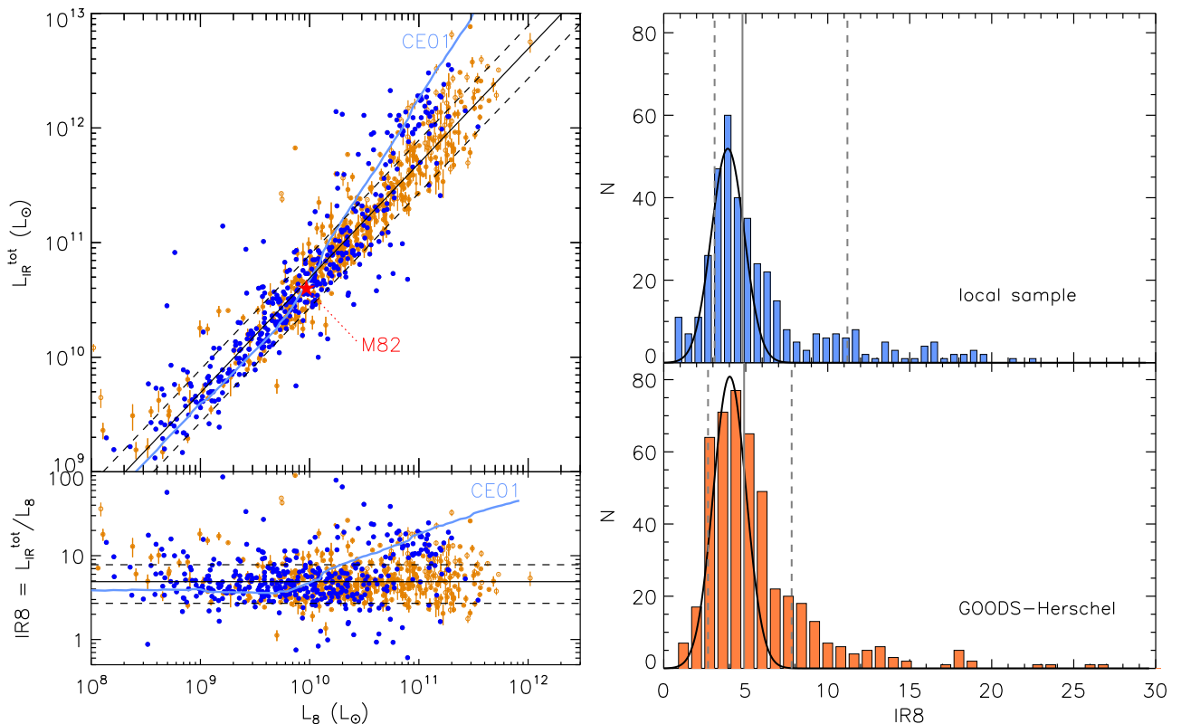
Fig. 9. Left: L_{\text{IR}}^{\text{tot}} [IRAS] versus L_8 for local ISO and AKARI galaxies (filled blue dots). The GOODS–Herschel galaxies are shown in the background with lighter orange symbols (same points as in Fig. 6) together with their median (black solid line) and 68 % dispersion (black dashed lines). The light blue line shows the locus traced by the CE01 SED library. Right: Histogram of the IR8 ratios for the local galaxy sample (blue, upper panel) and GOODS–Herschel sample (orange, bottom panel). The solid curves show Gaussians fit to the distributions. The vertical grey lines indicate the median (solid) and 68 % dispersion (dashed) for the full samples (as in Eqs. 3, 2).
