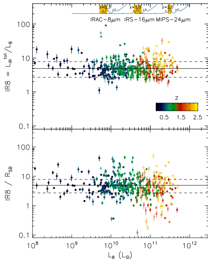
Fig. 25. IR8=L_{IR}^{tot}/L_{8\mu m} ratio as a function of L_{8\mu m} for star-forming galaxies, excluding recognized X-ray/optical AGN and infrared power-law AGN. The plain and dashed horizontal lines show the center and width of the Gaussian distribution of main sequence galaxies (Fig. 9 and Eq. 5). Upper panel: position of the star-forming galaxies as measured. Most fall on the same sequence as local star-forming galaxies. Bottom panel: position of the same galaxies after correcting their IR8 ratio for starburstiness (unless 0.5 \leq R_{SB} \leq 2 , where R_{SB} is consistent with unity within the error bars).
