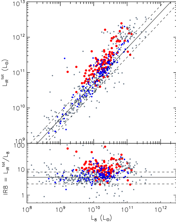
Fig. 14. L_{\text{IR}}^{\text{tot}} (top) and IR8 ratio (bottom) versus L[8\mu\text{m}] for the local galaxy sample (ISO, AKARI , Spitzer -GOALS). Galaxies with compact mid-IR (more than 60% of the light emitted at 13.2\mu\text{m} within the resolution element of 3.6'' ) and radio ( \Sigma_{\text{IR}} \geq 3 \times 10^{10} L_{\odot} ) light distributions are marked with large filled red dots. Here the solid and dashed lines present the median and 68% dispersion around the Gaussian distribution as defined in Eq 4.
