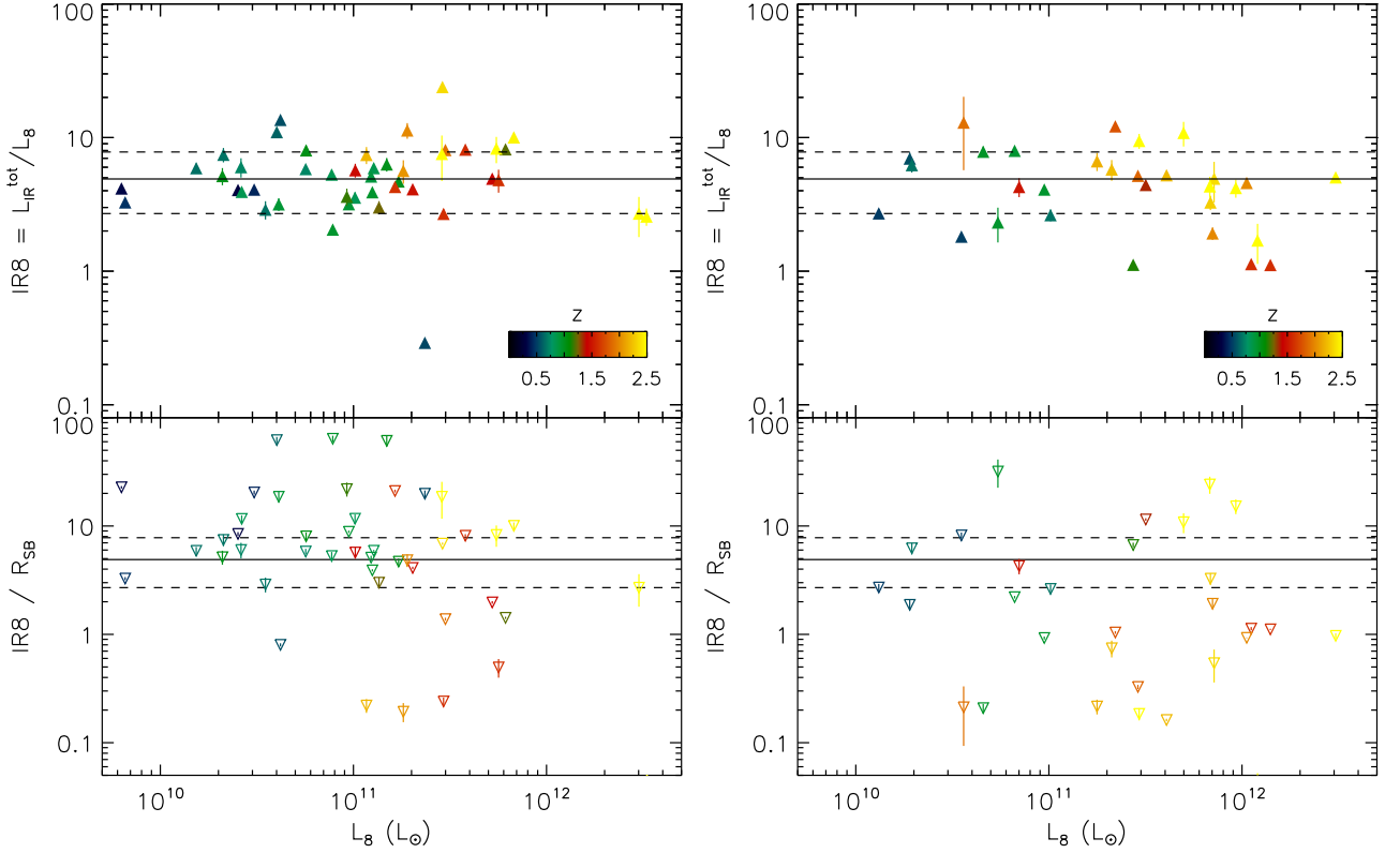
Fig. 24. Left: IR8=L_{IR}^{tot}/L_8 ratio as a function of L_8 for X-ray/optical AGN excluding power-law AGN. Upper panel: As-measured IR8 ratios of the X-ray/optical AGN. They fall on the same sequence as star-forming galaxies. Bottom panel: The same galaxies after de-boosting their IR8 ratios for starburstiness. The galaxies present a slightly different configuration, but basically remain centered on the trend of star-forming galaxies, suggesting that in these AGN the IR emission is dominated by star formation. Right: IR8 ratio as a function of L_8 for power-law AGN. Upper panel: As-measured IR8 ratios of the power-law AGN. They fall on the same sequence as star-forming galaxies, like the X-ray/optical AGN at left. Bottom panel: The same galaxies after de-boosting their IR8 ratios for starburstiness. A significant fraction of the galaxies now fall systematically below the main sequence IR8 ratio, showing that their 8\ \mu\text{m} emission is boosted by the hot dust heated by the AGN.
