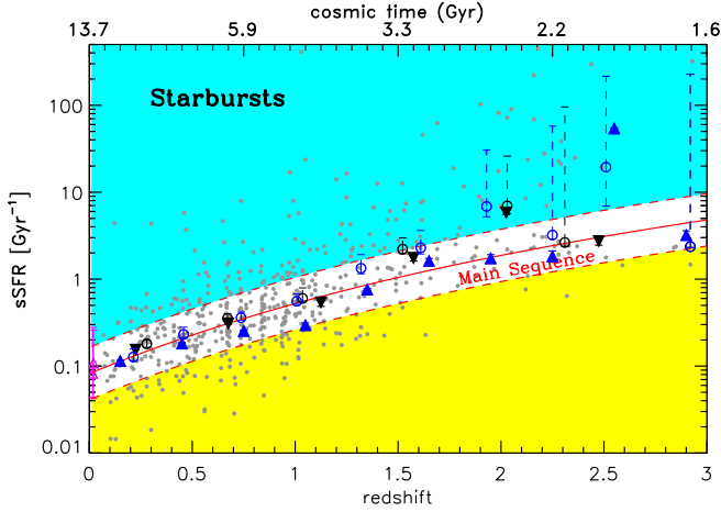
Fig. 18. Redshift evolution of the median specific SFR ( sSFR = SFR/M_* ) of star-forming galaxies. Values for individual GOODS– Herschel galaxies are shown as grey points. Median sSFR values in redshift bins are shown with open circles (blue for GOODS–N and black for GOODS–S). Values combining individual detections and stacking measurements for undetected sources are shown with filled triangles (blue upward for GOODS–N and black downward for GOODS–S). The red solid line is the fit shown in Eq. 13, and the dashed lines are a factor 2 above and below this fit. Starbursts are defined as galaxies with a sSFR > 2 \times sSFR_{MS} (blue zone). The yellow zone shows the galaxies with significantly lower sSFR values.
