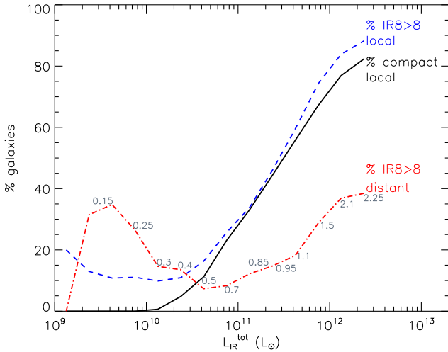
Fig. 15. Fractions of compact local galaxies (black line), local galaxies with IR8 > 8 (blue dashed line) and GOODS– Herschel galaxies with IR8 > 8 (red dash-dotted line) as a function of total IR luminosity. The median redshift of the GOODS– Herschel galaxies varies with L_{\text{IR}}^{\text{tot}} , and is indicated by labels in grey along the red dash-dotted line.
