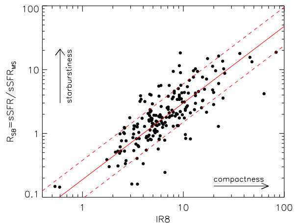
Fig. 17. R_{\text{SB}} = sSFR/sSFR_{\text{MS}} versus IR8 (= L_{\text{IR}}^{\text{tot}}/L_8) for z \sim 0 galaxies (AKARI and GOALS samples). The red line is the best fit (plain) and its 0.3 dex dispersion (dashed).
