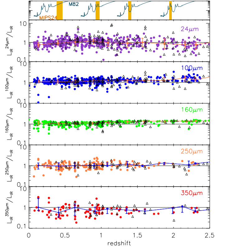
Fig. 23. Ratio of the extrapolated ( L_{\text{IR}}^{\lambda} ) over Herschel total IR luminosity as a function of redshift, for all clean GOODS– Herschel galaxies. L_{\text{IR}}^{\lambda} is computed by normalizing the main sequence SED to the broadband photometric measurement at \lambda . The 5 passbands used for the extrapolation are, from the top to bottom, Spitzer MIPS– 24\mu\text{m} , Herschel PACS– 100\mu\text{m} & 160\mu\text{m} , Herschel SPIRE– 250\mu\text{m} & 350\mu\text{m} . L_{\text{IR}} = L_{\text{IR}}^{\text{Herschel}} is measured using the full set of Herschel measurements at rest-frame wavelengths \lambda > 30\mu\text{m} to normalize the main sequence SED and by integrating over 8\text{--}1000\mu\text{m} . Black triangles: AGN. The solid lines with error bars are the sliding median and the 16th and 84th percentiles around it. Upper panel: SED of M82 and MIPS 24\mu\text{m} filter at z=0.25, 0.9, 1.4, 2 .
