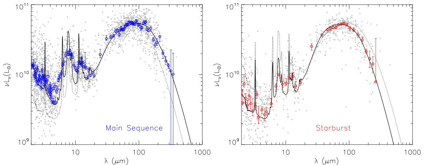
Fig. 21. Composite spectral energy distribution of the typical main sequence galaxy ( left ; IR8=4\pm 2 , see Eq. 5) and starburst ( right ; IR8>8 , i.e., above 2\sigma ). Light grey dots: individual GOODS–Herschel galaxies normalized to L_{IR}^{tot} = 10^{11} L_{\odot} . The large filled symbols with error bars are the median and associated uncertainty of the MS (left figure, blue dots) and SB (right figure, red dots) galaxies computed in intervals of wavelengths defined to contain a fixed number of 25\pm 5 galaxies. The uncertainty on the median values is derived from the 16th and 84th percentiles around the median divided by the square root of the number of galaxies. The model fit to each SED is shown with a solid black line while the opposing SED (MS or SB) is shown with a dotted black line for comparison.
