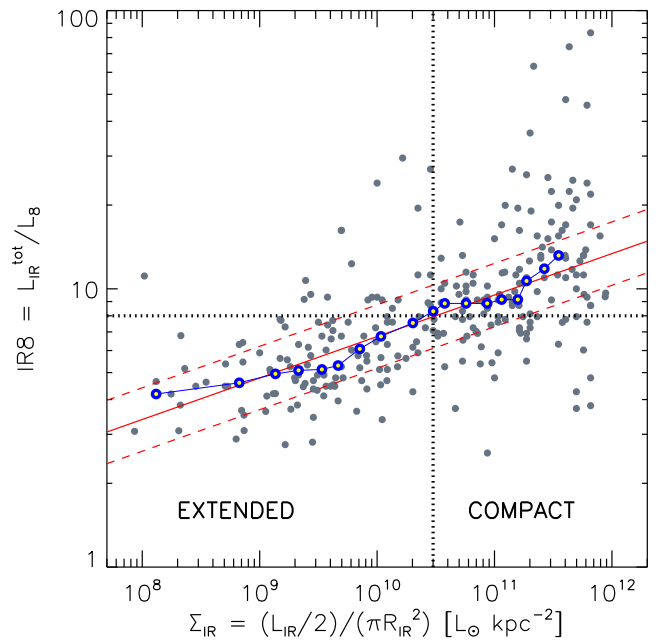
Fig. 13. Dependence of IR8 ( =L_{\text{IR}}^{\text{tot}}/L[8\mu\text{m}] ) with \Sigma_{\text{IR}} ( =L_{\text{IR}}^{\text{tot}}/(2\times\pi R_{\text{IR}}^2) ), the IR surface brightness. Galaxies to the right of the vertical dotted line are considered to be compact star-forming galaxies ( \Sigma_{\text{IR}}\geq 3\times 10^{10} L_{\odot}\text{kpc}^{-2} ). Galaxies above the horizontal dotted line exhibit IR8 ratio that is two times larger than that of main sequence galaxies, which follow the Gaussian IR8 distribution shown in Fig. 9). The sliding median is shown with open blue dots. It is fitted by the solid line in red and its 16th and 84th percentiles are fitted with the dashed red lines (see Eq. 8).
