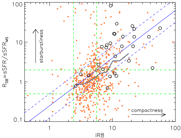
Fig. 19. R_{\text{SB}} = \text{sSFR}/\text{sSFR}_{\text{MS}} versus IR8 (=L_{\text{IR}}^{\text{tot}}/L_8) for the distant GOODS–Herschel galaxies. The green lines show the range of values occupied by main sequence galaxies (68 % dispersion) in sSFR (horizontal lines; R_{\text{SB}} = 1 \pm 1 ) and IR8 (vertical lines; IR8_{\text{MS}} = 4 \pm 1.6 , see Eq. 5). The thick grey line shows the sliding median for the GOODS–Herschel galaxies. The diagonal blue lines are the best fit (solid) and 68 % dispersion (dashed) for local galaxies as in Fig. 17. Large open dots show the position of sub-mm galaxies from Menendez-Delmestre et al. (2009) and Pope et al. (2008a).
