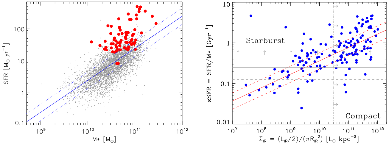
Fig. 16. Left: SFR – M_{*} correlation at z \sim 0 . Galaxies classified as compact are marked with large filled red dots. Solid line: fit to the main sequence SFR– M_{*} relation: SFR \propto M_{*}/[4 \times 10^9 M_{\odot}] . Dotted lines: 16th and 84th percentiles of the distribution around the sliding median (0.26 dex). Right: Relation of the sSFR and IR surface brightness of galaxies for which a radio size was estimated. The vertical dashed line illustrates the threshold above which galaxies have been classified as compact. The solid and dashed red lines are a fit to the sliding median of the relation (Eq. 11) and its 68 % dispersion.
