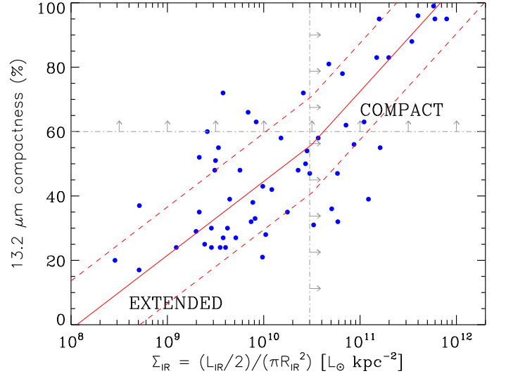
Fig. 11. Comparison of the two compactness indicators: \Sigma_{\text{IR}} ( =L_{\text{IR}}^{\text{tot}}/(2\times\pi R_{\text{IR}}^2) ), the IR surface brightness, and 13.2 \mu\text{m} compactness (percentage of unresolved Spitzer /IRS light at 13.2 \mu\text{m} , Díaz-Santos et al. 2010).
