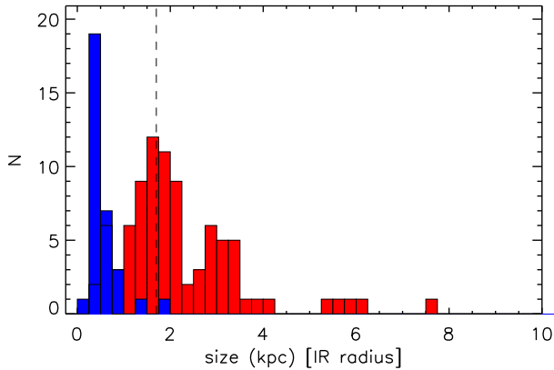
Fig. 12. Distribution of IR sizes (half-light radius) of 119 local galaxies as derived from their 1.4 GHz radio continuum using Eq. 6. Galaxies with an IR surface brightness greater than \Sigma_{\text{IR}}=3\times 10^{10} L_{\odot}\text{kpc}^{-2} , i.e., compact galaxies, are in blue, while extended galaxies are in red. The vertical dashed line indicates the typical resolution of \sim 1.7 kpc of the mid-IR compactness at 13.2\mu\text{m} estimated by Díaz-Santos et al. (2010).
