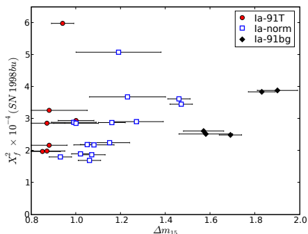
FIG. 9.— \chi_f^2 versus \Delta m_{15} for the fit of the time-integrated, dust-scattered, reddened, and flattened SN Ia spectra to the observed light echo spectrum associated with SN 1998bu. The SN Ia subtypes “Ia-91T”, “Ia-norm”, and “Ia-91bg” are indicated with filled red circles, open blue squares, and filled black diamonds, respectively.
