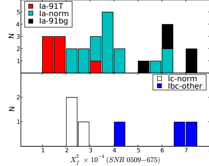
FIG. 14.— The upper panel shows the histogram of \chi_f^2 for the fit of the time-integrated, dust-scattered, reddened, and flattened SN Ia spectra fit to the flattened observed light echo spectrum associated with SNR 0509-675. Note that nearly all 91T-like SNe Ia have a better \chi_f^2 than any SNe of the other subtypes. The lower panel shows the same histogram of \chi_f^2 for the SNe Ib/c. Note that the normal SNe Ic have a decent \chi_f^2 , but all 91T-like SNe with \Delta m_{15} < 0.9 have a better \chi_f^2 .
