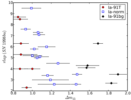
FIG. 8.— Correlation parameter rlap of the light echo of SN 1998bu determined with SNID versus \Delta m_{15} of the time-integrated, dust-scattered, reddened, and flattened SN Ia spectra. The SN Ia subtypes “Ia-91T”, “Ia-norm”, and “Ia-91bg” are indicated with filled red circles, open blue squares, and filled black diamonds, respectively.
