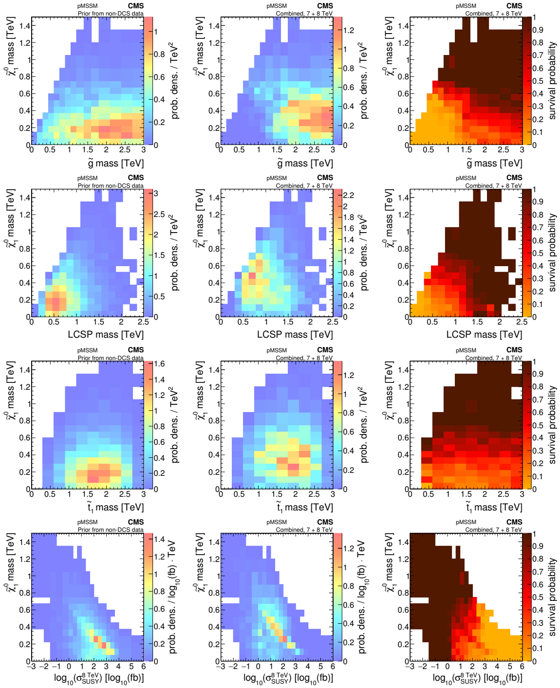
Figure 11. Marginalized non-DCS distributions (first column), compared with posterior distributions (second column) and survival probabilities (third column) after inclusion of the considered CMS searches, are shown for the \tilde{\chi}_1^0 mass versus gluino mass (first row), the LCSP mass (second row), the top squark mass (third row), and the logarithm of the cross section for inclusive sparticle production at 8 TeV (bottom row).
