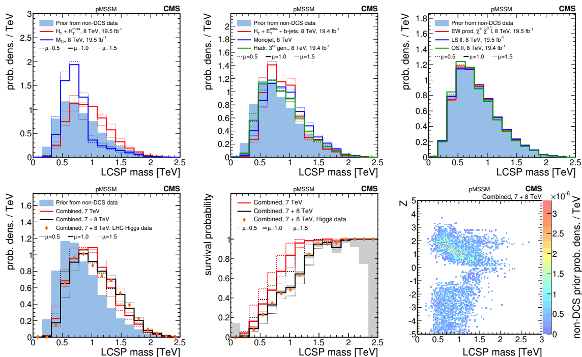
Figure 4. A summary of the impact of CMS searches on the probability density of the mass of the lightest colored SUSY particle (LCSP) in the pMSSM parameter space. The first-row and bottom-left plots compare the non-DCS prior distribution of the LCSP mass to posterior distributions after data from various CMS searches, where the bottom-left plot shows the combined effect of CMS searches and the Higgs boson results. The bottom-center plot shows survival probabilities as a function of the LCSP mass for various combinations of CMS data and data from Higgs boson measurements. The bottom-right plot shows the distribution of the LCSP mass versus the Z -significance calculated from the combination of all searches. See figure 2 for a description of the shading.
