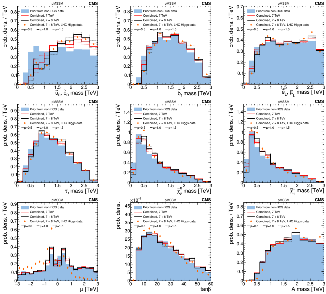
Figure 9. Comparison of prior and posterior distributions after several combinations of data from the CMS searches for the \tilde{u}_R, \tilde{c}_R mass, \tilde{b}_1 mass, \tilde{e}_L, \tilde{\mu}_L mass, \tilde{\tau}_1 mass, \tilde{\chi}_1^0, \tilde{\chi}_2^0 mass, \tilde{\chi}_1^\pm mass, the higgsino mass parameter \mu , \tan\beta , and A mass.
