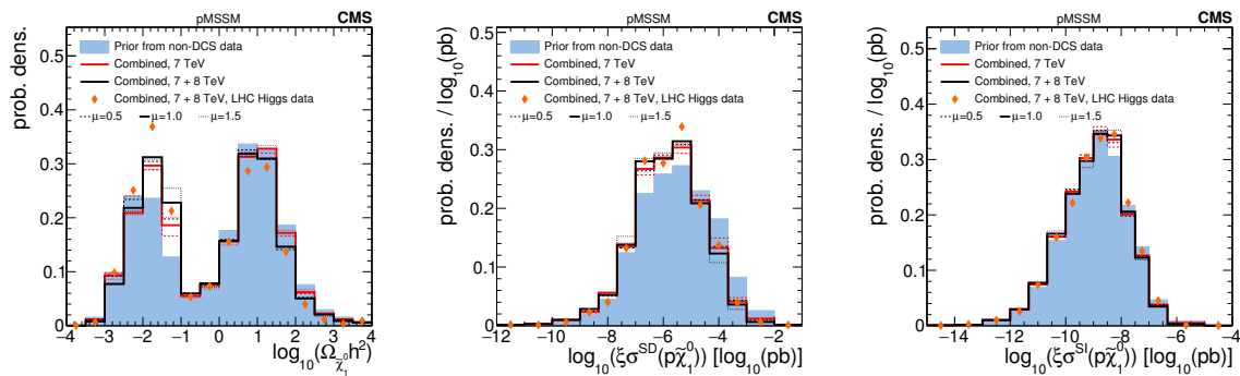
Figure 10. Comparison of prior and posterior distributions after several combinations of data from the CMS searches for \Omega_{\tilde{\chi}_1^0} , \xi\sigma^{SD}(p\tilde{\chi}_1^0) , and \xi\sigma^{SI}(p\tilde{\chi}_1^0) .
