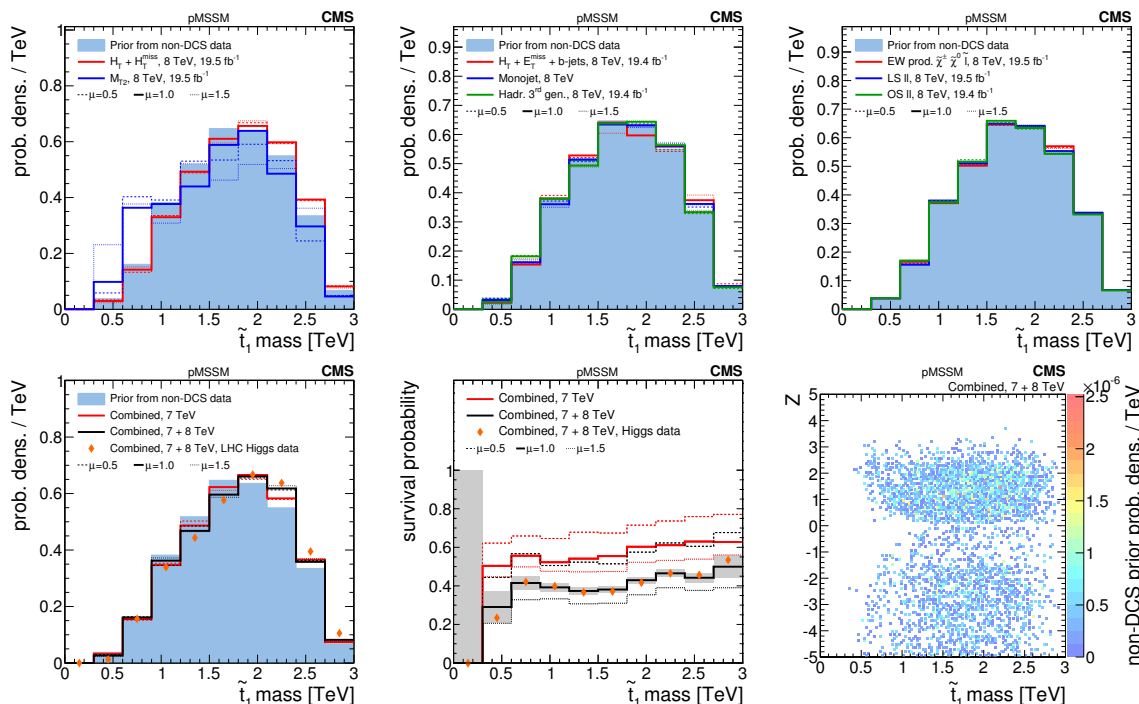
Figure 5. A summary of the impact of CMS searches on the probability density of the \tilde{t}_1 mass in the pMSSM parameter space. The first-row and bottom-left plots compare the non-DCS prior distribution of the \tilde{t}_1 mass to posterior distributions after data from various CMS searches, where the bottom-left plot shows the combined effect of CMS searches and the Higgs boson results. The bottom-center plot shows survival probabilities as a function of the \tilde{t}_1 mass for various combinations of CMS data and data from Higgs boson measurements. The bottom-right plot shows the distribution of the \tilde{t}_1 mass versus the Z -significance calculated from the combination of all searches. See figure 2 for a description of the shading.
