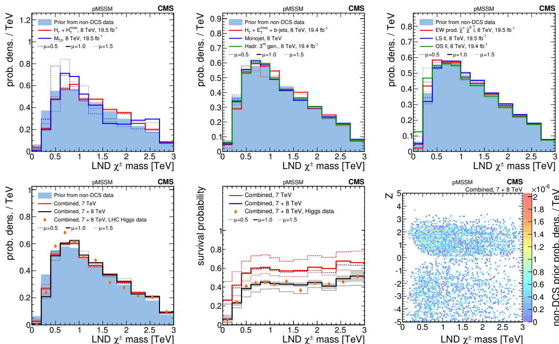
Figure 7. A summary of the impact of CMS searches on the probability density of the mass of the lightest non-degenerate (LND) chargino in the pMSSM parameter space. The first-row and bottom-left plots compare the non-DCS prior distribution of the LND \tilde{\chi}^\pm mass to posterior distributions after data from various CMS searches, where the bottom-left plot shows the combined effect of CMS searches and the Higgs boson results. The bottom-center plot shows survival probabilities as a function of the LND \tilde{\chi}^\pm mass for various combinations of CMS data and data from Higgs boson measurements. The bottom-right plot shows the distribution of the LND \tilde{\chi}^\pm mass versus the Z-significance calculated from the combination of all searches. See figure 2 for a description of the shading.
