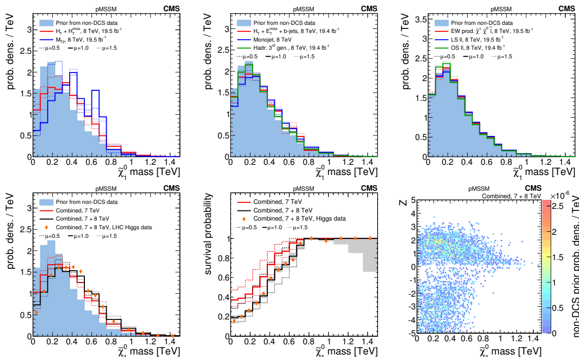
Figure 6. A summary of the impact of CMS searches on the probability density of the \tilde{\chi}_1^0 mass in the pMSSM parameter space. The first-row and bottom-left plots compare the non-DCS prior distribution of the \tilde{\chi}_1^0 mass to posterior distributions after data from various CMS searches, where the bottom-left plot shows the combined effect of CMS searches and the Higgs boson results. The bottom-center plot shows survival probabilities as a function of the \tilde{\chi}_1^0 mass for various combinations of CMS data and data from Higgs boson measurements. The bottom-right plot shows the distribution of the \tilde{\chi}_1^0 mass versus the Z -significance calculated from the combination of all searches. See figure 2 for a description of the shading.
