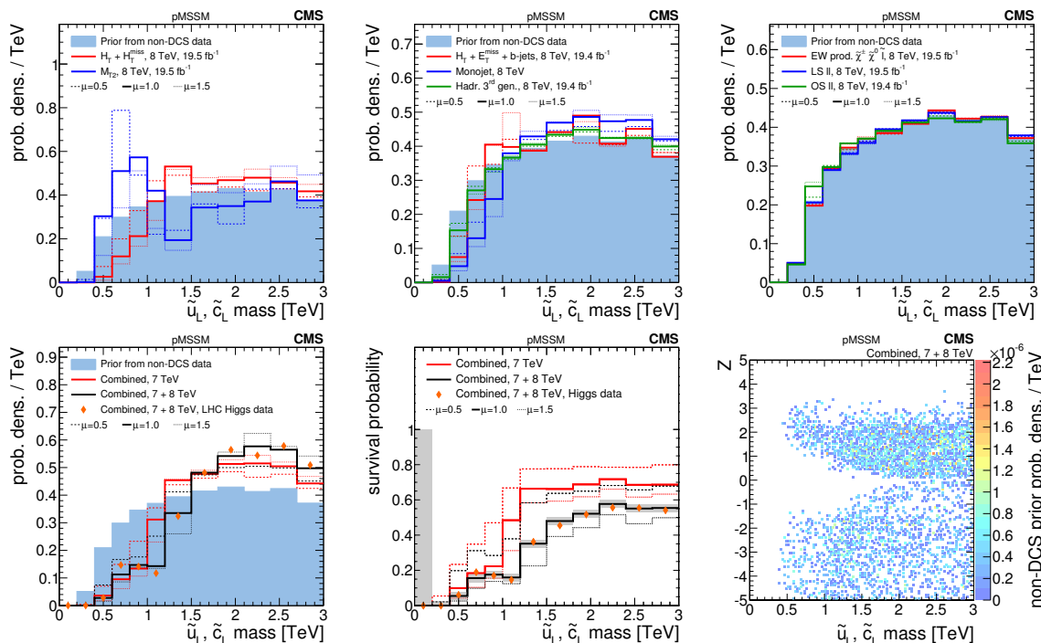
Figure 3. A summary of the impact of CMS searches on the probability density of the \tilde{u}_L mass (equivalently, the \tilde{c}_L mass) in the pMSSM parameter space. The first-row and bottom-left plots compare the non-DCS prior distribution of the \tilde{u}_L mass to posterior distributions after data from various CMS searches, where the bottom-left plot shows the combined effect of CMS searches and the Higgs boson results. The bottom-center plot shows survival probabilities as a function of the \tilde{u}_L mass for various combinations of CMS data and data from Higgs boson measurements. The bottom-right plot shows the distribution of the \tilde{u}_L mass versus the Z -significance calculated from the combination of all searches. See figure 2 for a description of the shading.
