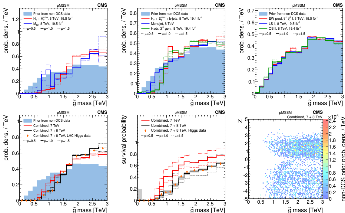
Figure 2. A summary of the impact of CMS searches on the probability density of the gluino mass in the pMSSM parameter space. The first-row and bottom-left plots compare the non-DCS prior distribution of the gluino mass (blue filled histograms) to posterior distributions after data from various CMS searches (line histograms), where the bottom-left plot shows the combined effect of CMS searches and the Higgs boson results. The bottom-center plot shows survival probabilities as a function of the gluino mass for various combinations of CMS data and data from Higgs boson measurements, where the shaded grey band gives the statistical uncertainty on the black histogram. The bottom-right plot shows the distribution of the gluino mass versus the Z -significance calculated from the combination of all searches.
