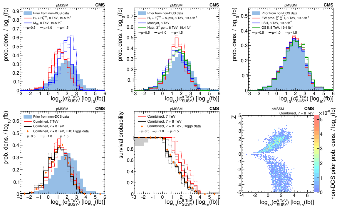
Figure 8. A summary of the impact of CMS searches on the probability density of the logarithm of the cross section for inclusive sparticle production in 8 TeV pp collisions, \log_{10}(\sigma_{\text{SUSY}}^{8 \text{ TeV}}) , in the pMSSM parameter space. The first-row and bottom-left plots compare the non-DCS prior distribution of the \log_{10}(\sigma_{\text{SUSY}}^{8 \text{ TeV}}) to posterior distributions after data from various CMS searches, where the bottom-left plot shows the combined effect of CMS searches and the Higgs boson results. The bottom-center plot shows survival probabilities as a function of the \log_{10}(\sigma_{\text{SUSY}}^{8 \text{ TeV}}) for various combinations of CMS data and data from Higgs boson measurements. The bottom-right plot shows the distribution of the \log_{10}(\sigma_{\text{SUSY}}^{8 \text{ TeV}}) versus the Z -significance calculated from the combination of all searches. See figure 2 for a description of the shading. In plot (bottom left), the apparent enhancement of the left tail of the posterior density with respect to the prior is due to the suppression of the right tail and an overall renormalization.
