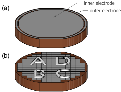
FIG. 2 (color online). a) Inner and outer electrodes for measuring the ionization signal. The inner electrode extends from the center to a radius of 34.5 mm and the outer electrode extends from a radius of 35.5 mm to just before the edge (0.5–2 mm; the diameter of the detectors is 76 mm). b) Phonon channels (QETs) A–D arranged in quadrants on the opposite side of the detector. Each phonon channel is composed of approximately 1000 TESs formed from thin films deposited onto the crystal surface and then photolithographically structured. The TESs are connected in parallel to form the QETs and each QET is read out by its own circuit containing a SQUID array.
