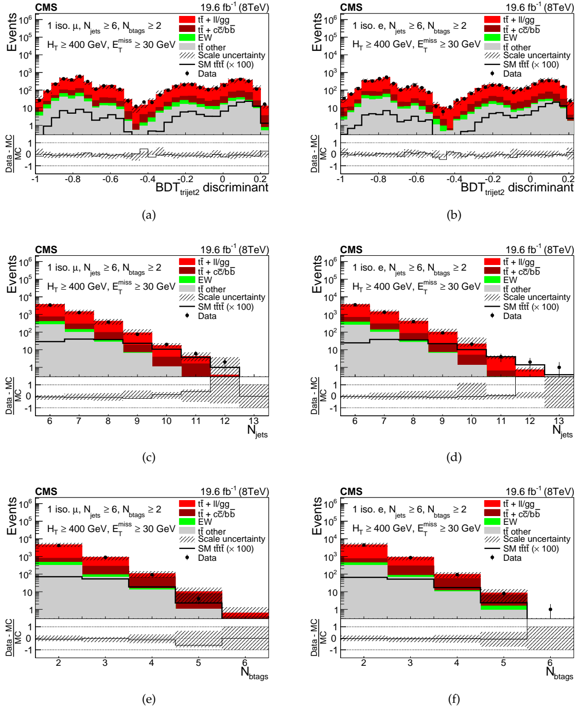
Figure 2: The distribution in the \text{BDT}_{\text{trijet2}} discriminant for the \mu + jets and e + jets channels in (a) and (b), respectively, and the same for N_{\text{jets}} in (c) and (d), and for N_{\text{btags}} in (e) and (f). The ratios plotted at the bottom of each panel reflect the percent differences between data and MC events. The hatched areas show the changes in the calculated predictions produced by factors of two and one half changes in the factorisation and renormalisation scales in the t\bar{t} simulation.
