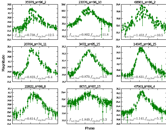
Figure 8. Light curves for a selection of candidates showing secondary periods with f_{\text{sig}} > 5.0 . The ratio f_{\text{primary}}/f_{\text{secondary}} does not fall into the range for either F or FO pulsators. These candidates also show somewhat less scatter with respect to their characteristic photometric uncertainties. This suggests that the pulsation amplitudes for both modes may be similar which may contribute error to the secondary frequency determination.
