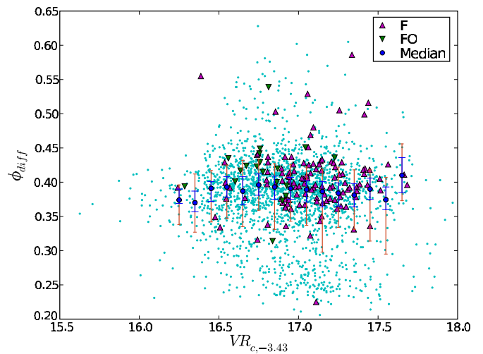
Figure 13. \phi_{\text{diff}} against VR_c for all candidates. Blue circles and error bars are as described in the caption of Figure 5. See the caption of Figure 3 for description of remaining symbols. We find that the lag between \phi_{\text{max}} and \phi_{\text{min}} is similar for all candidates, though candidates pulsating in overtone modes tend to have \phi_{\text{diff}} greater than the median. \phi_{\text{diff}} closer to 0.5 indicates a more symmetric light curve.
