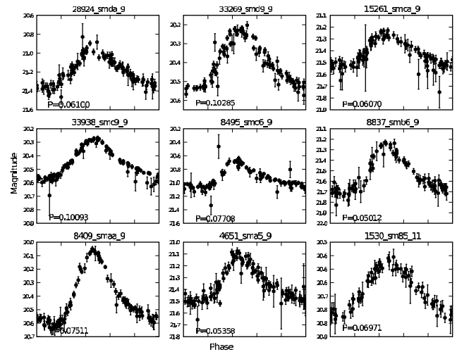
Figure 2. Light curves for a selection of \delta -Scuti candidates.
