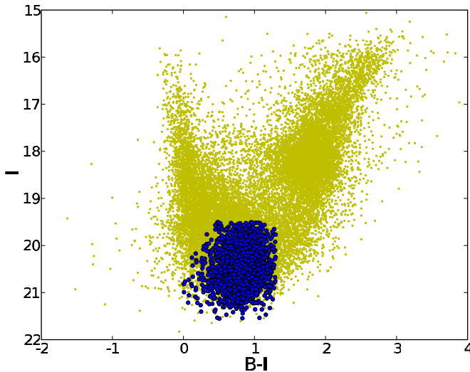
Figure 1. B-I color-magnitude diagram. Yellow dots show all star-type sources in the B and I catalog for a single amplifier in field sm97. The CMD is similar for all SuperMACHO fields. The filled blue circles show the final set of HADS candidates. Candidate selection criteria include the requirement that the source lie on the main sequence.
