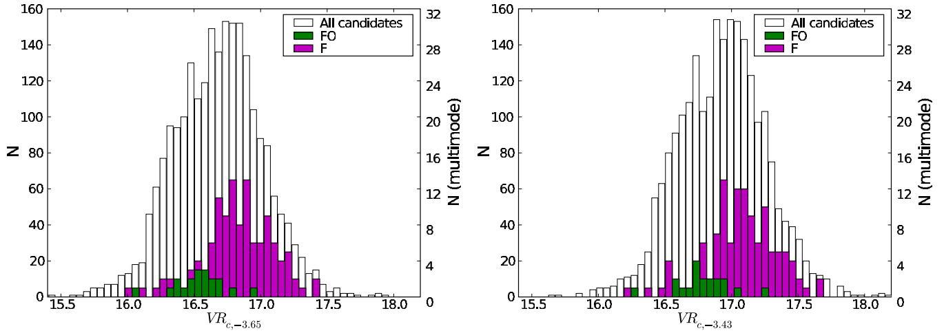
Figure 4. Figure showing the histogram of PL-relation-corrected luminosities, VR_c . We show histograms for the PL-relation-corrected magnitudes of the candidates using both the slope from P08 (left) and the slope independently determined from this data (right). The double-mode F and FO pulsators are overlotted in maroon and green, respectively. The histograms of the double-mode candidates are scaled for visibility, and the scaling is shown on the right y-axis. For both slopes, we find the histogram is skewed toward brighter sources. This excess of brighter sources is often interpreted as evidence of overtone mode pulsators (see Section 4.3). (A color version of this figure is available in the online journal.)
