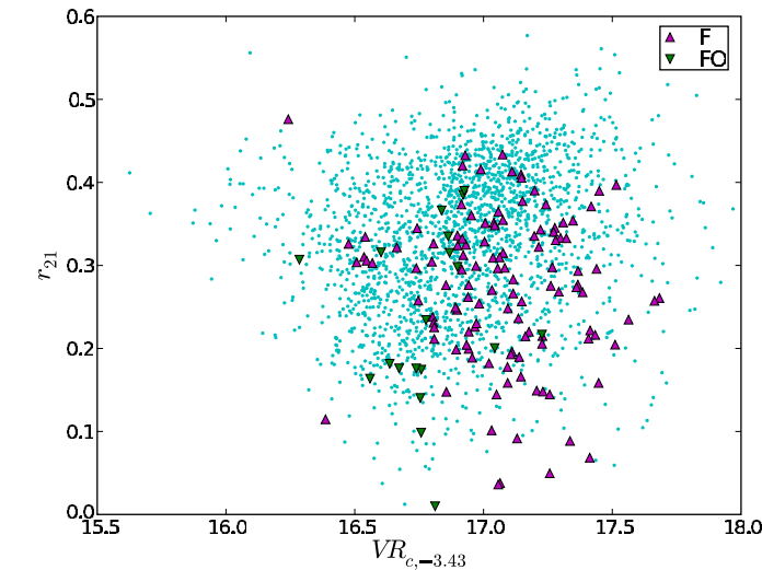
Figure 11. r_{21} against VR_c and histogram of r_{21} for all candidates. Because \phi_{21} is similar for all candidates (see Figure 12), r_{21} measures the relative contributions of the second and first Fourier components to the overall amplitude. See the caption of Figure 3 for description symbols in the left panel. In the right panel, white bars show the histogram of r_{21} for all candidates. Overplotted in red are fainter candidates with VR_c > 16.8 . Overplotted in blue are brighter candidates with VR_c < 16.8 . We find that the brighter values of VR_c also have smaller values of r_{21} indicating a more symmetric light curve.
