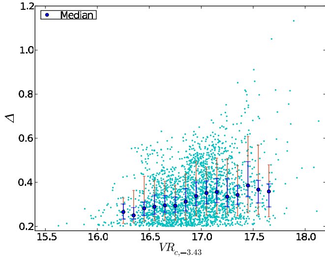
Figure 10. \Delta against VR_c for all candidates. \Delta gives the peak-to-trough amplitude of the phased light curve. We bin the candidates by VR_c . The blue circles show the median amplitudes for each bin. The error bars show the 33rd and 66th percentile as described in the caption of Figure 5. We do not show bins containing fewer than 20 candidates. We find that the brightest candidates have the lowest amplitudes. We also find few candidates having \Delta > 0.4 mag that are brighter than VR_c = 16.8 .
