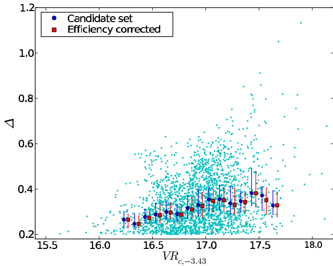
Figure 14. Efficiency-corrected plot of amplitude against VR_c . We show a plot similar to Figure 10. The red squares show the efficiency-corrected median values. We show the original (blue circles) and corrected (red squares) 33rd percentile errors (see the caption of Figure 5). For visibility, we show these values slightly offset from the center of the bin positions.
