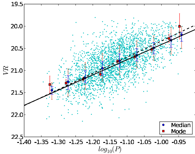
Figure 5. PL diagram of all candidates with fitted PL relation. The cyan dots show all \delta -Scuti candidates. The blue circles give the median magnitudes for each period. The blue and orange error bars show the 33rd and 66th percentiles of the population, respectively, i.e., 33% ( \pm 17.5\% ) and 66% ( \pm 33\% ) of the candidates within each bin lie between the ends of the error bars. We note that the distribution in each bin is not always symmetric about the median. The red squares show the mode for each bin, and their errors show the inverse square root of the number of sources in the bin. To improve visibility, we show the median and mode values slightly offset from the center of the bin position. The solid line is the best-fit PL relation to the modes (see Equation (4)). The dashed black line is the best-fit PL relation when fixing the slope to that given by P08 (see Equation (3)).
