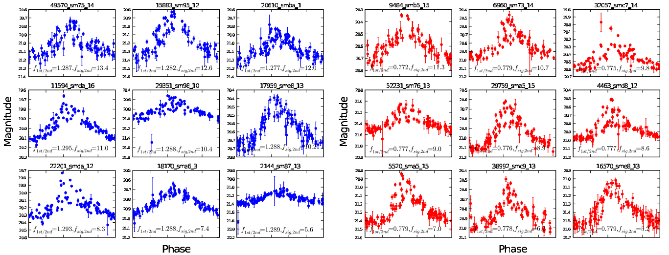
Figure 7. Light curves for a selection of candidates showing secondary periods with f_{\text{sig}} > 5.0 . The plot on the left shows candidates with 1.275 < f_{\text{primary}}/f_{\text{secondary}} < 1.305 . The plot on the right shows candidates with 0.765 < f_{\text{primary}}/f_{\text{secondary}} < 0.790 . These groups correspond to multimode FO and F pulsators, respectively.
