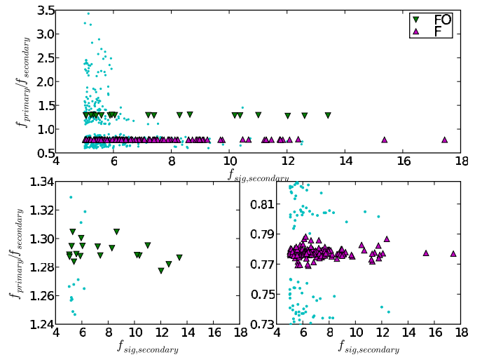
Figure 6. Ratio between primary and secondary frequencies against f_{\text{sig,secondary}} . We plot the ratio of the primary to the secondary frequency of variability against the significance of the secondary frequency for all candidates showing secondary frequencies with significance greater than 5 (see Reegen 2007). We have removed any candidates showing only secondary frequencies that have whole number ratios to the primary. We find 119 candidates with 0.765 < f_{\text{primary}}/f_{\text{secondary}} < 0.790 (green pentagons) and 19 candidates with 1.275 < f_{\text{primary}}/f_{\text{secondary}} < 1.305 (maroon diamonds). These likely correspond to double-mode and overtone pulsators, respectively. We note the appearance of less dense additional clusters of candidates with secondary modes at frequency ratios of \sim 0.74 and \sim 0.8 , and we identify an outlier at f_{\text{primary}}/f_{\text{secondary}} = 1.452 . The close proximity of these clusters to ratios with the FO frequency suggests that these may also belong to the groups described above. As shown in Figure 8, these light curves show significantly less scatter with respect to their characteristic photometric uncertainties than those falling into the above classifications, even for similar values of f_{\text{sig,secondary}} . We conclude that the secondary frequency determination for these sources may be unreliable.
