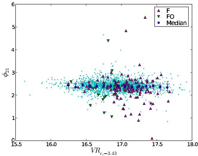
Figure 12. \phi_{21} against VR_c for all candidates. We find that \phi_{21} is similar for all candidates, r_{21} can be used as a measure of the ratio of the overall amplitude. Blue circles and error bars are as described in the caption of Figure 5. See the caption of Figure 3 for description of remaining symbols.
