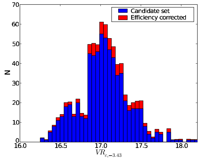
Figure 15. Efficiency-corrected histogram of VR_c for only sources with \Delta > 0.4 . The blue bars show the observed histogram, and the red bars give the efficiency-corrected histogram. We find an indication of an excess of larger amplitude, subluminal sources around VR_c = 17.4 . This may be the subluminal population observed in Fornax by Poretti et al. (2008).
