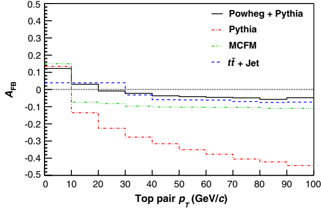
FIG. 22 (color online). Expected A_{\text{FB}} as a function of the p_T^{\bar{t}t} of the t\bar{t} system at the parton level from MCFM, POWHEG, and PYTHIA, as well as a NLO prediction for events where the top-quark pair is produced in association with an extra energetic jet.
