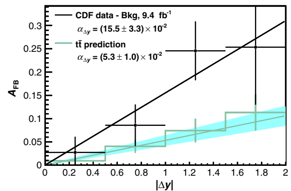
FIG. 15 (color online). The background-subtracted asymmetry as a function of |\Delta y| with a best-fit line superimposed. Error bars include both statistical and background-related systematic uncertainties. The shaded region represents the theoretical uncertainty on the slope of the prediction.
