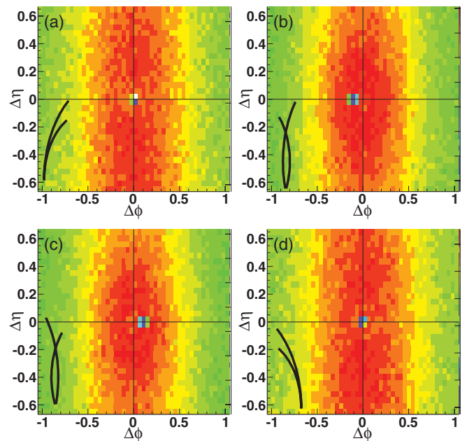
FIG. 3. (Color online) The dip region in (\Delta\phi, \Delta\eta) uncorrected dihadron correlations in 0–12% central Au+Au collisions at \sqrt{s_{NN}} = 200 \text{ GeV} for 3 < p_T^{\text{trigger}} < 6 \text{ GeV}/c and 1.5 \text{ GeV}/c < p_T^{\text{associated}} < p_T^{\text{trigger}} in the four helicity combinations of trigger and associated particles: (a) (h_{\text{trig}}, h_{\text{assoc}}) = (1, 1) , (b) (h_{\text{trig}}, h_{\text{assoc}}) = (1, -1) , (c) (h_{\text{trig}}, h_{\text{assoc}}) = (-1, 1) , and (d) (h_{\text{trig}}, h_{\text{assoc}}) = (-1, -1) . Cartoons indicate which dips are from track merging and which are from track crossing.
