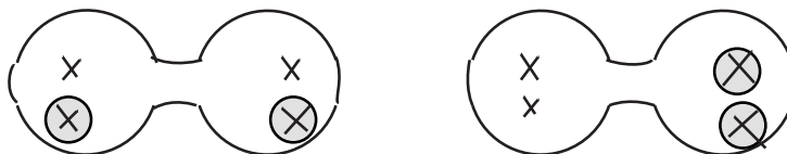
Figure 5. a) The weakly coupled SU(3) description, here the cross denotes U(1) puncture and circle cross denotes SU(3) puncture; b) Description with weakly coupled SU(2) gauge group
