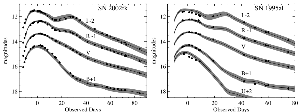
Figure 14. MLCS2k2 fits to the multi-band data for SN 1995al and SN 2002fk. (Light curves and fits.)
