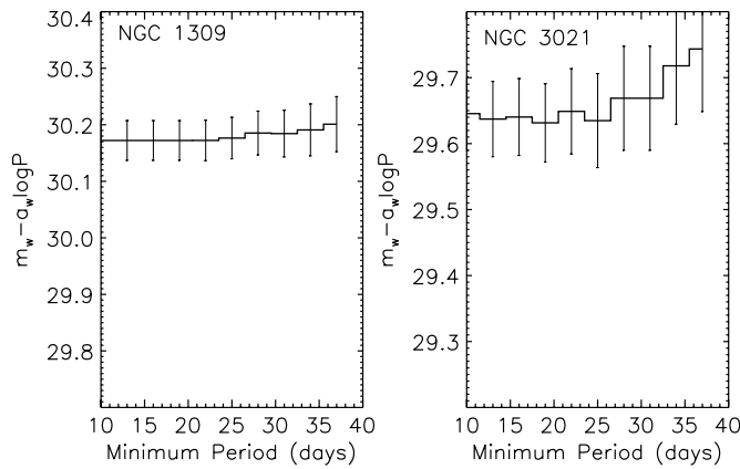
Figure 7. Dereddened distance modulus from the P - w relation as a function of the period cutoff. Although there is some evidence of an incompleteness bias at the short-period end of the V -band and I -band P - L relations, there is no significant change in the dereddened distance modulus with period cutoff.
