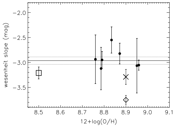
Figure 12. The measured slopes of the dereddened (Wesenheit) P-w relations as a function of the mean metallicity parameter. The seven hosts in Table 2 (including the inner region of NGC 4258) have solar-like metallicities and slopes which are mutually consistent with their mean of -2.98 \pm 0.07 . This mean is consistent with the slope inferred from parallax distances to Galactic Cepheids (van Leeuwen et al. 2007) indicated by the X, in good agreement with the LMC slope (square), and inconsistent with the Galactic slope (diamond) inferred from non-geometric distance measures (Tammann et al. 2003).
