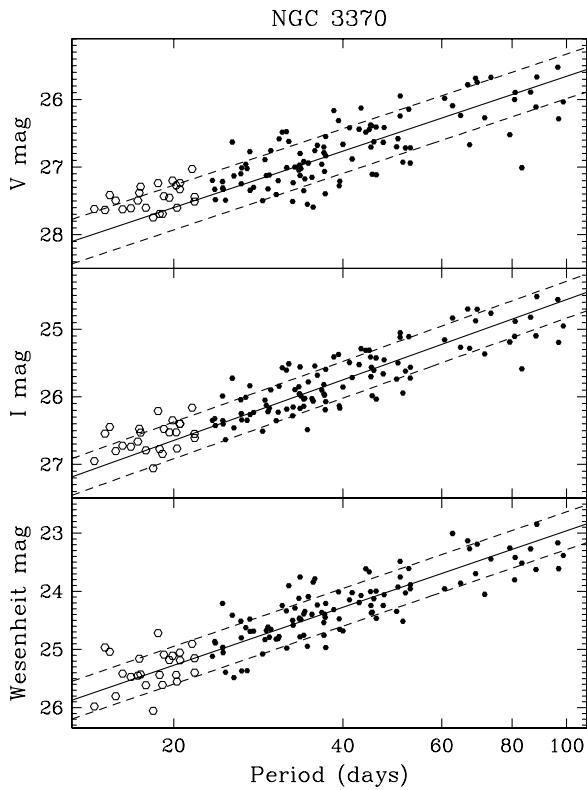
Figure 8. Same as Figure 5 but for NGC 3370.
