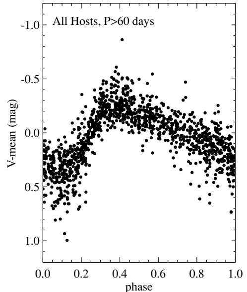
Figure 10. Composite V-band Cepheid light curves of the longer-period Cepheids, P > 60 d, whose discovery was enabled by reobservations of each host HST cycles subsequent to the discovery cycle. Although Cepheids at P > 60 d have reduced amplitudes, they exhibit the characteristic sawtooth light curve of a classical Cepheid and serve to extend the use of the P-L to greater distances.
