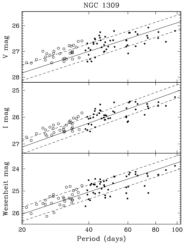
Figure 5. V -band, I -band, and Wesenheit dereddened [V - 2.45(V - I)] P-L relations for Cepheids identified in NGC 1309. The P-L relation shown is from the LMC and is only fit to the filled symbols (see Figure 12 for a slope fit to the individual relations). An approximate instability-strip width of 0.35 mag is also given for comparison. Open symbols indicate short-period Cepheids in the period range which appears to suffer an incompleteness bias (preferentially bright or significantly blended with a blue source).
