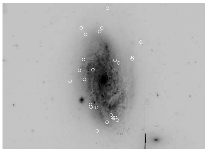
Figure 2. Same as Figure 1 but for NGC 3021.
