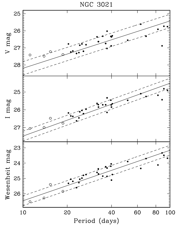
Figure 6. Same as Figure 5 but for NGC 3021.
