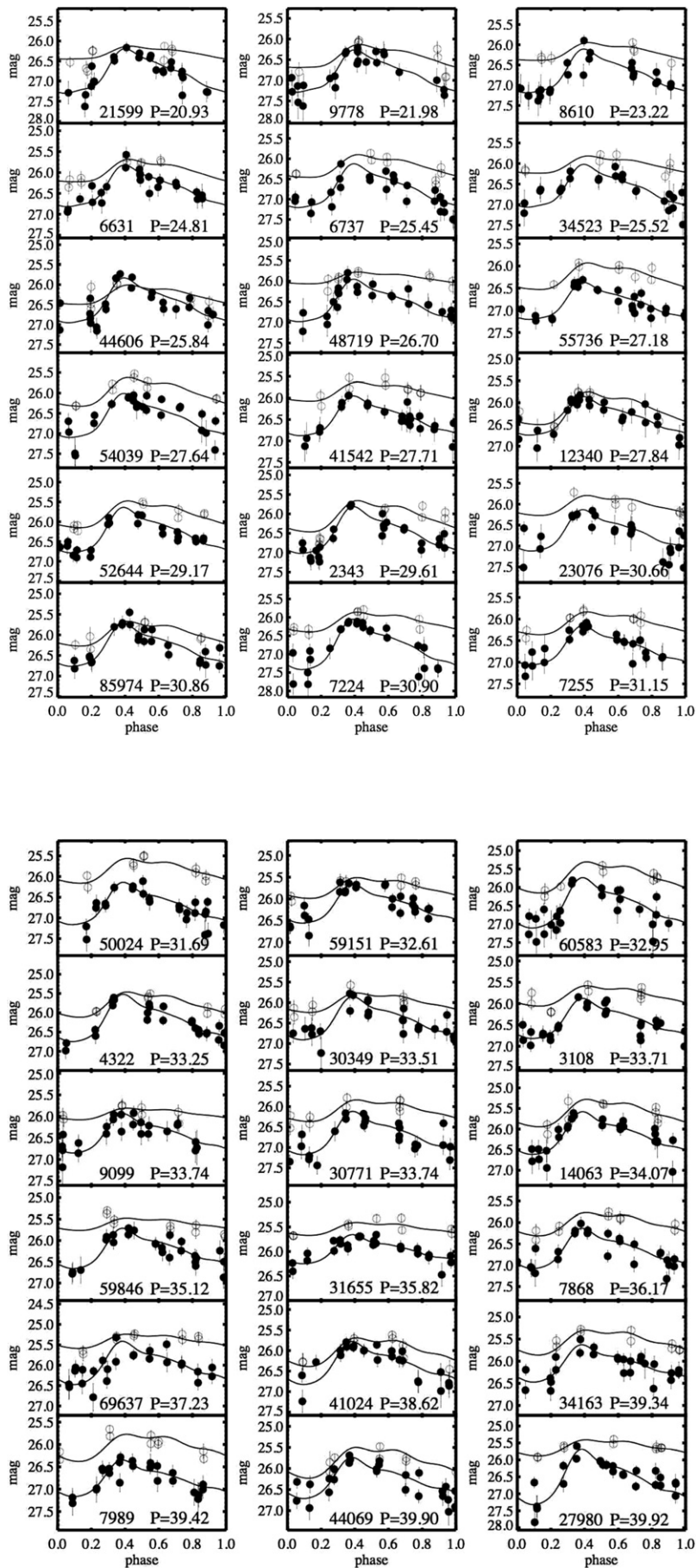
Figure 4. Same as Figure 3 but for NGC 1309 (see Table 7).
