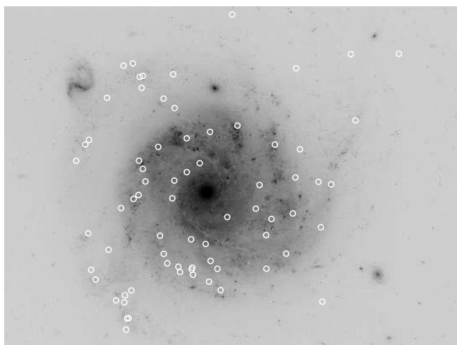
Figure 1. Image of a 2' \times 2' region of the field of NGC 1309 from ACS WFC F555W . North is up and east to the left. The locations of the Cepheids identified are indicated by circles.
