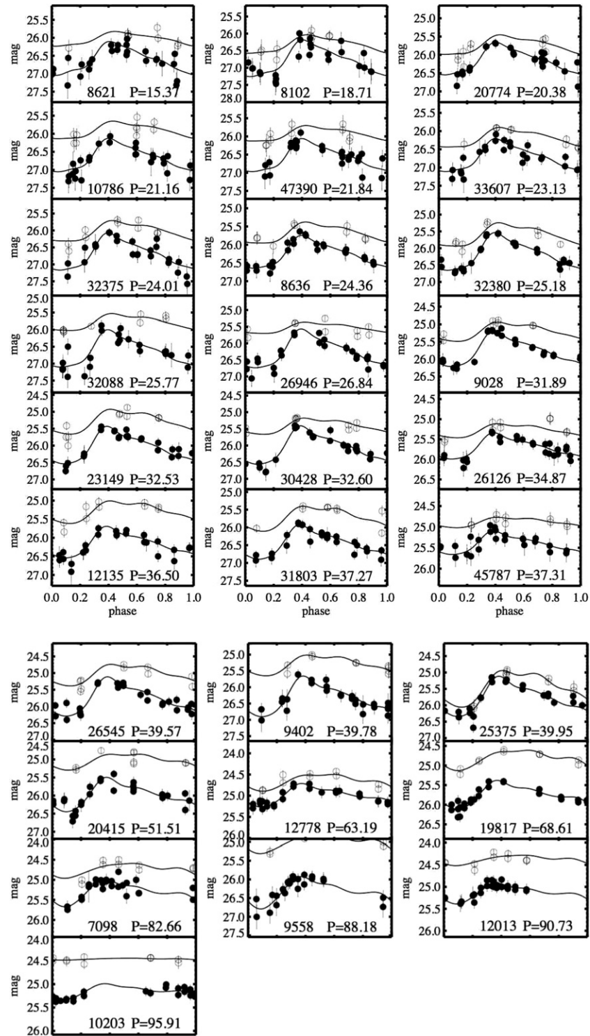
Figure 3. F555W and F814W light curves of Cepheids in NGC 3021. For each of the Cepheid candidates listed by identification number in Table 8, the photometry is fit to the period-specific light-curve template.
