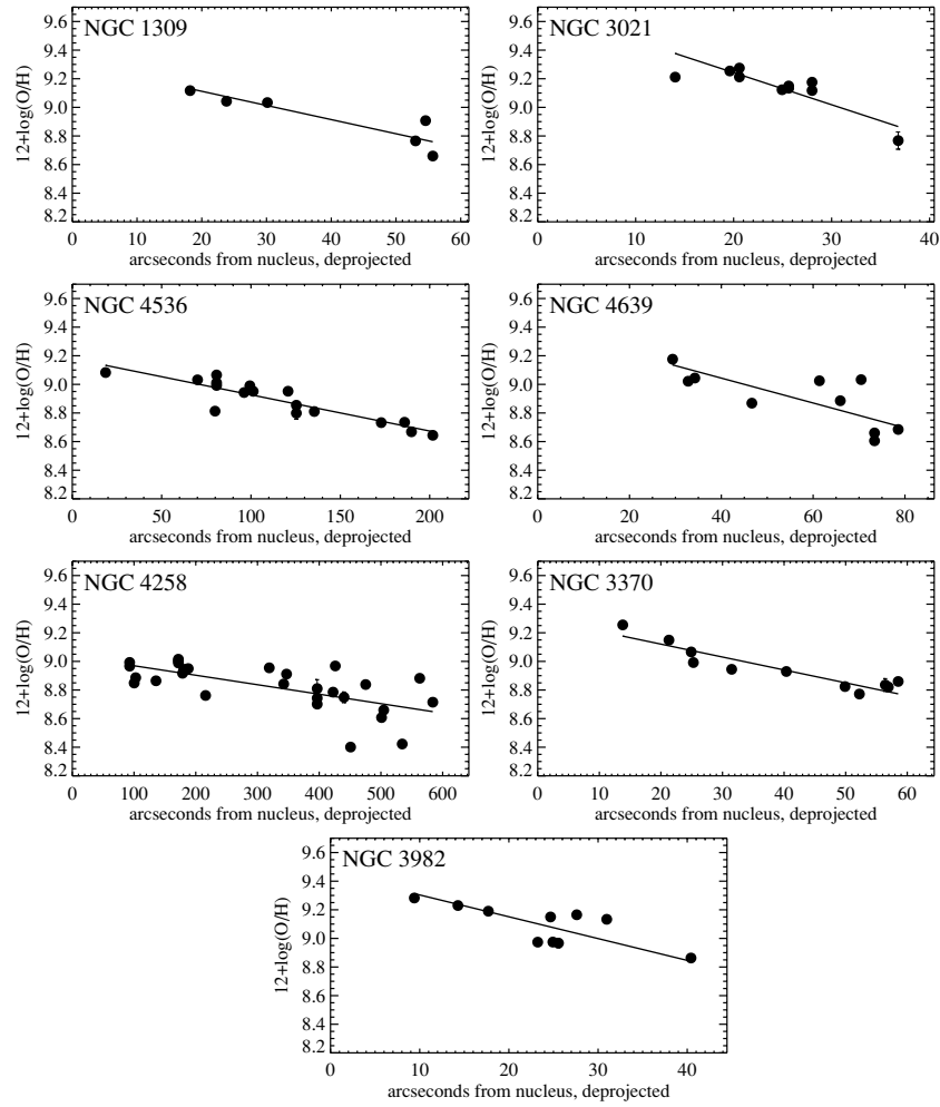
Figure 11. Radial gradients of the oxygen-to-hydrogen ratios [O/H] of H II regions in the Cepheid hosts. Following the method of Zaritsky et al. (1994), emission-line intensity ratios of [O II] \lambda\lambda 3726, 3729 , [O III] \lambda\lambda 4959, 5007 , and H\beta were used to derive values of 12 + \log[O/H] for H II regions. The fitted linear gradient was used to determine the value of the metallicity correction at the individual radii of the observed Cepheids. The variance in the data is dominated by spatial variations, not measurement errors.
