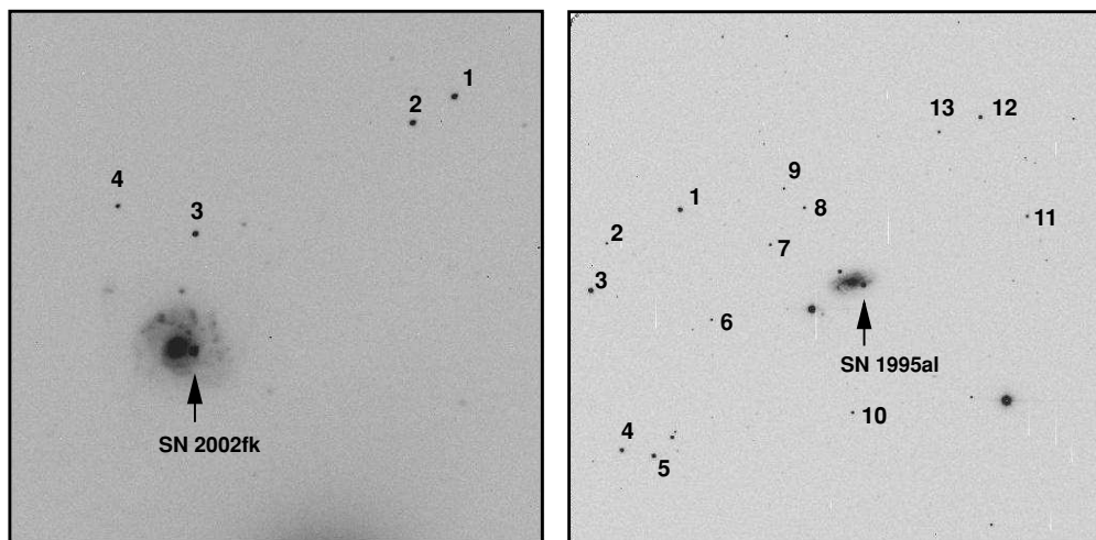
Figure 13. Ground-based comparison stars in the field of NGC 1309 (SN 2002fk; left) and NGC 3021 (SN 1995al; right) used to calibrate the light curves of the respective SNe Ia. (Comparison star finders for SNe.)
