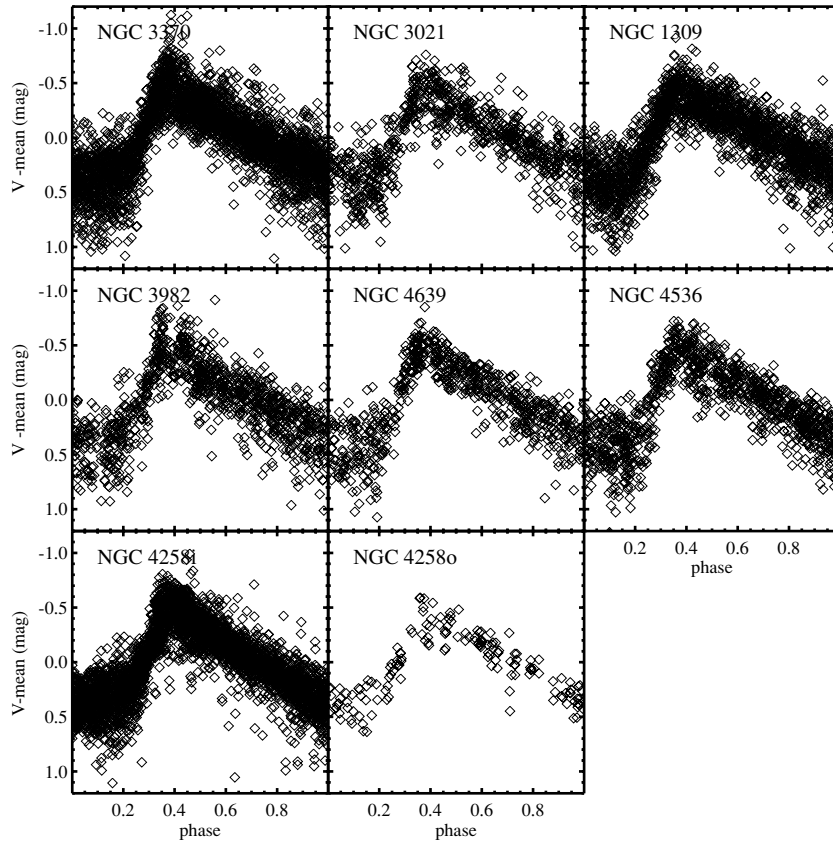
Figure 9. Composite V-band Cepheid light curves. For the Cepheids with P > 10 d in each host, the fitted mean magnitude was subtracted from the observations which were then plotted as a function of their phase, as inferred from the fitted period. As seen and shown in Table 11, for each host the mean half-amplitude is consistent with 0.48 mag. This consistency indicates a lack of significant variation in blending from host to host and also provides a more direct probe of metallicity which can cause amplitude differences in the mean.
