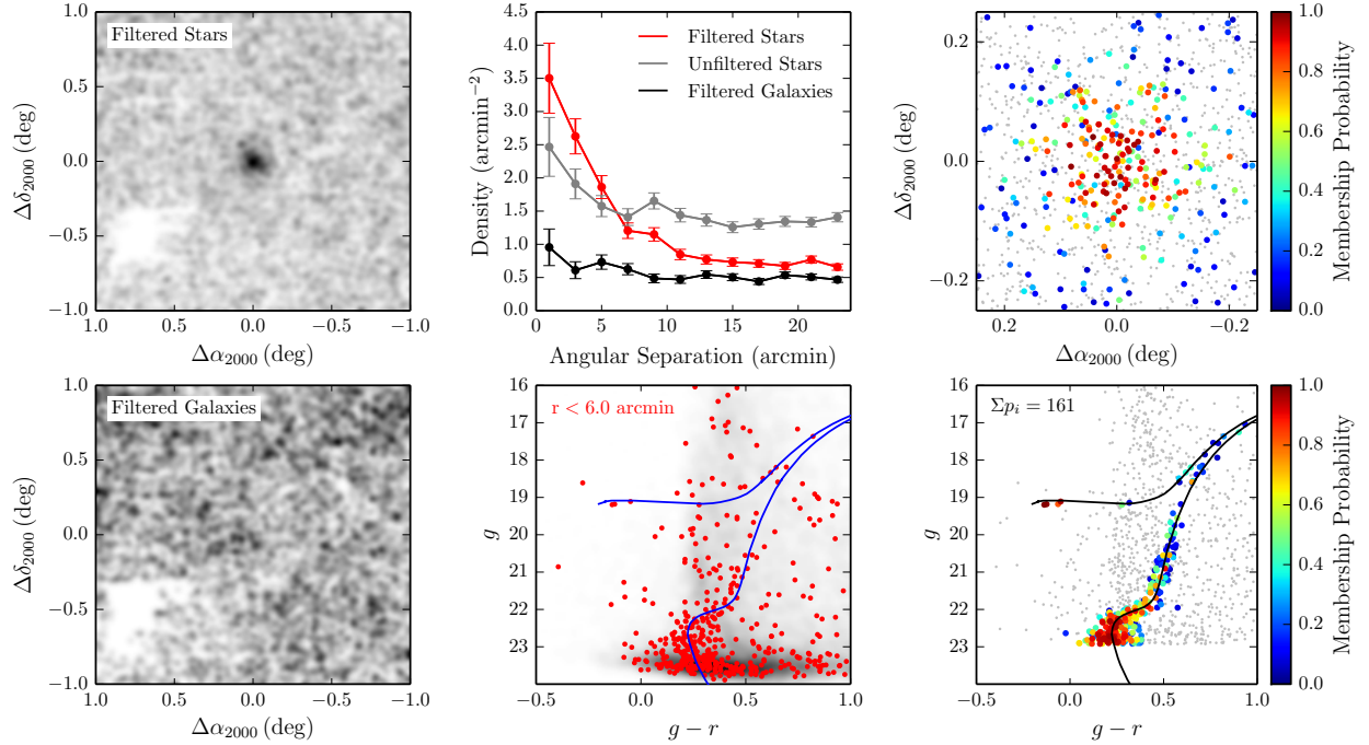
Fig. 6.— Stellar density and color-magnitude diagrams for DES J2204–4626 (Grus II). Top left : Spatial distribution of stellar objects with g < 24 mag that pass the isochrone filter (see text). The field of view is 2^{\circ} \times 2^{\circ} centered on the candidate and the stellar distribution has been smoothed by a Gaussian kernel with standard deviation 1''.2 . Top center : Radial distribution of objects with g - r < 1 mag and g < 24 mag: stars passing the isochrone filter (red), stars excluded from the isochrone filter (gray), and galaxies passing the isochrone filter (black). Top right : Spatial distribution of stars with high membership probabilities within a 0''.5 \times 0''.5 field of view. Small gray points indicate stars with membership probability less than 5%. Bottom left : Same as top left panel, but for probable galaxies that pass the isochrone filter. Bottom center : The color-magnitude distribution of stars within 0''.1 of the centroid are indicated with individual points. The density of the field within an annulus from radii of 0''.5 to 1''.0 is represented by the background two-dimensional histogram in grayscale. The blue curve shows the best-fit isochrone as described in Table 1 and Table 2. Bottom right : Color-magnitude distribution of high membership probability stars.
