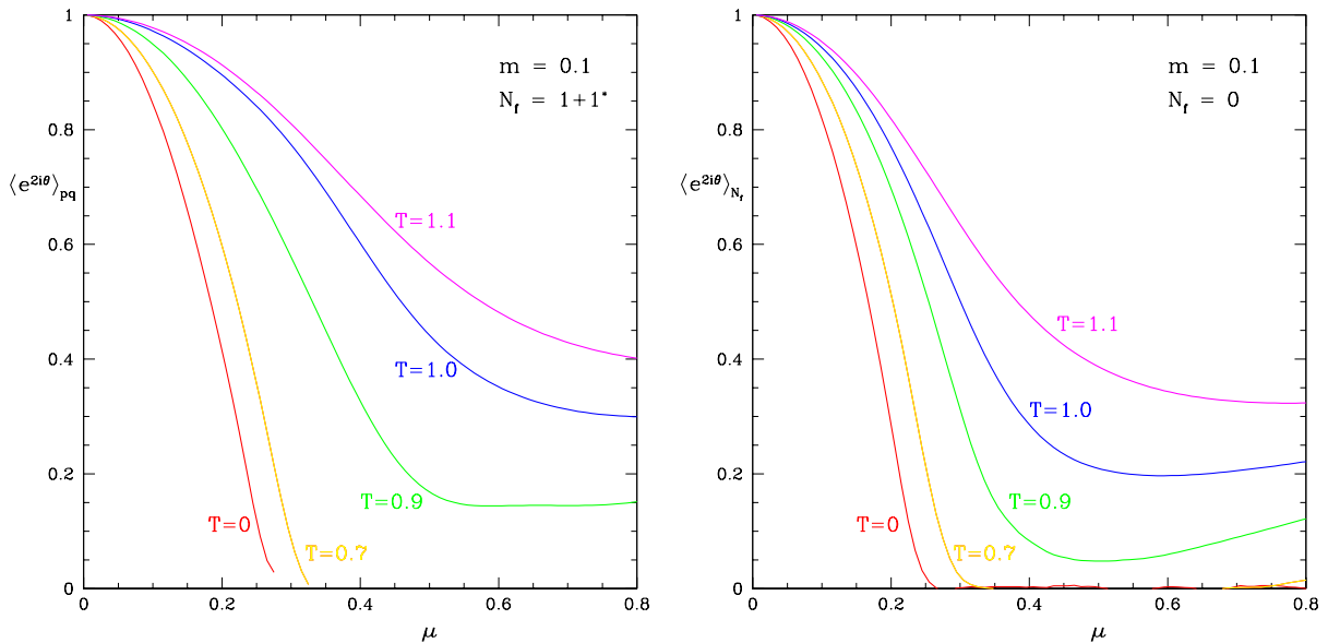
FIG. 6: Phase quenched (left) and quenched (right) average phase factor versus chemical potential. Results have been obtained from the chiral random matrix model (74).
