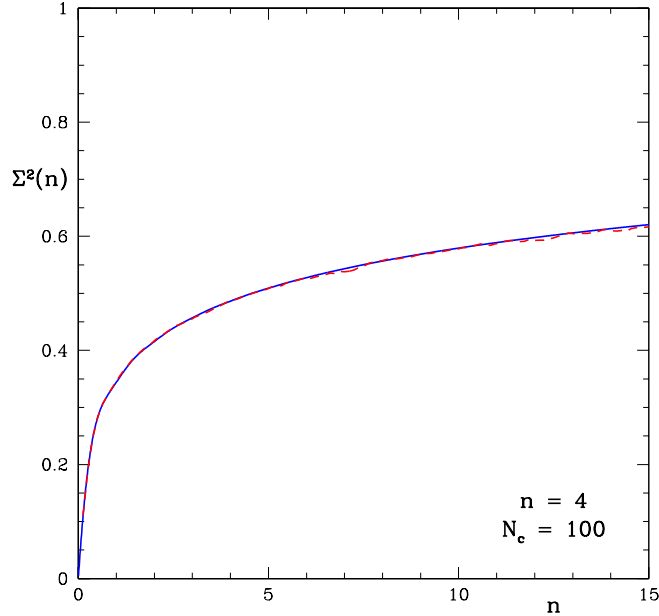
FIG. 7: The number variance for n = 4 and N_c = 100 .
