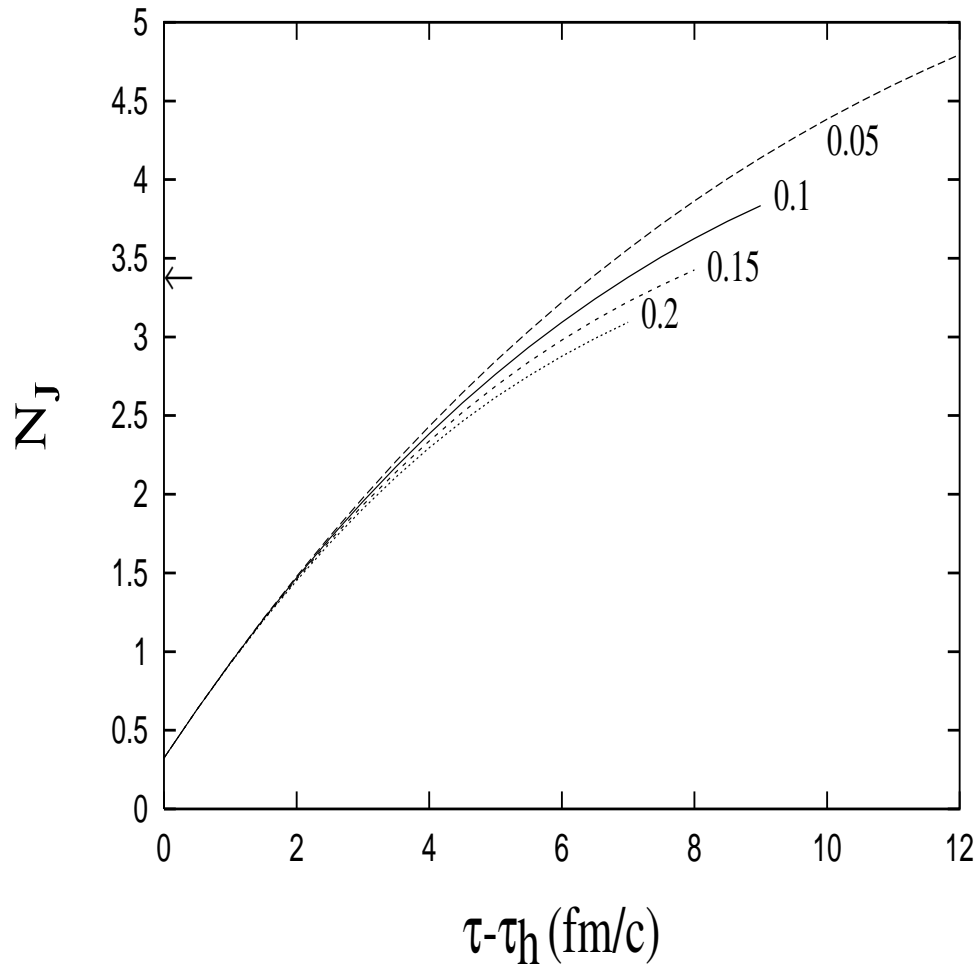
FIG. 3. Time evolution of the abundance of J/\psi and D from Au+Au collisions at LHC for different values of transverse acceleration a ( c^2/\text{fm} ). The initial J/\psi number is denoted by the left arrow.
