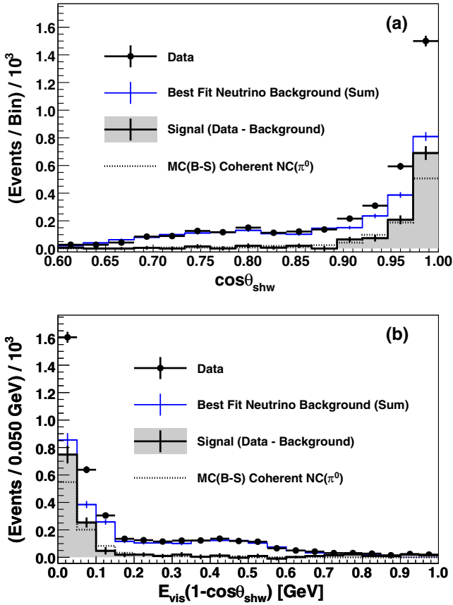
FIG. 10. Distributions of candidate NC( \pi^0 ) coherent-scattering events (solid circles, statistical error bars) in \cos\theta_{\text{shw}} (a) and \eta_\pi (b). The data are compared to the estimate for the neutrino backgrounds (thin blue-line histograms). The coherent-scattering signal (data minus background) is shown by the shaded histogram, together with the signal rate inferred using the Berger-Sehgal model (dotted histogram).
