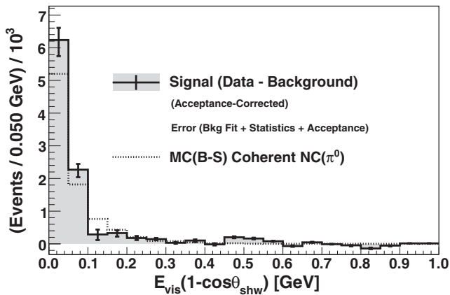
FIG. 11. Distribution in \eta_\pi for the acceptance-corrected data excess above the total neutrino background rate, for events having E_{\text{vis}} > 1.0 GeV (shaded histogram). The dotted-line histogram shows the Berger-Sehgal prediction.
