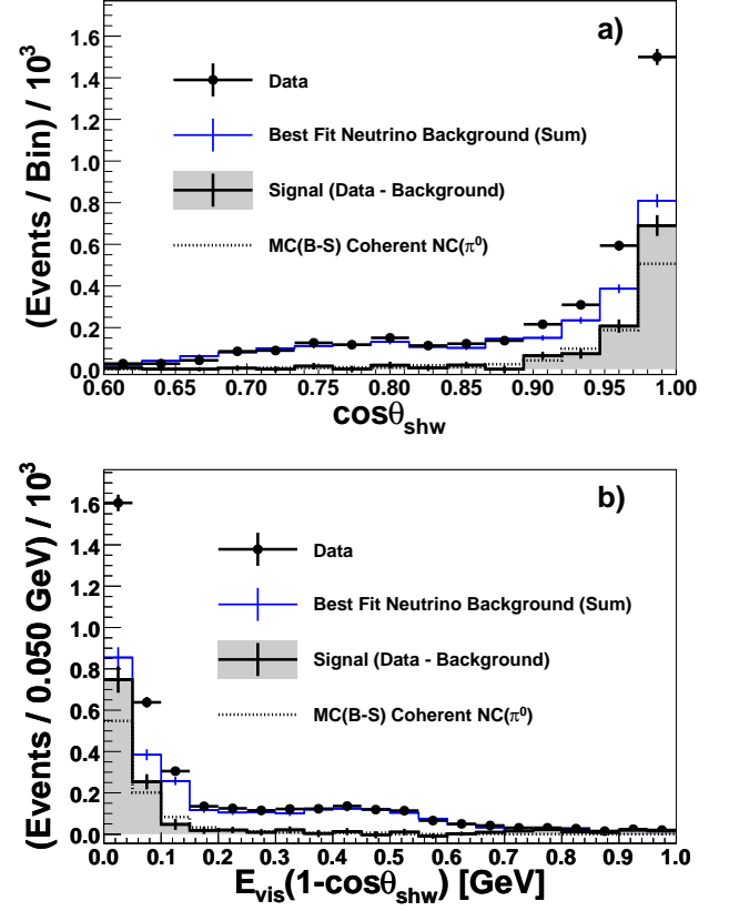
FIG. 10. Distributions of candidate NC( \pi^0 ) coherent scattering events (solid circles, statistical error bars) in \cos\theta_{shw} (a) and \eta_\pi (b). The data are compared to the estimate for the neutrino backgrounds (thin blue-line histograms). The coherent scattering signal (data minus background) is shown by the shaded histogram, together with the signal rate inferred using the Berger-Sehgal model (dotted histogram).
