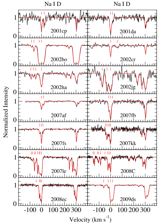
Figure 2. VPFIT models for the Na I D absorption lines for SNe Ia where the K I lines were not observed or detected. The red lines above the D2 line in each spectrum indicate the velocities of the components used to fit the profiles. The most prominent (deepest) component is used to set the zero point of the velocity scale.
