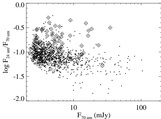
FIG. 3.— The ratio of 24/70 \mu\text{m} flux versus the 70 \mu\text{m} flux. AGNs are indicated by diamonds.
