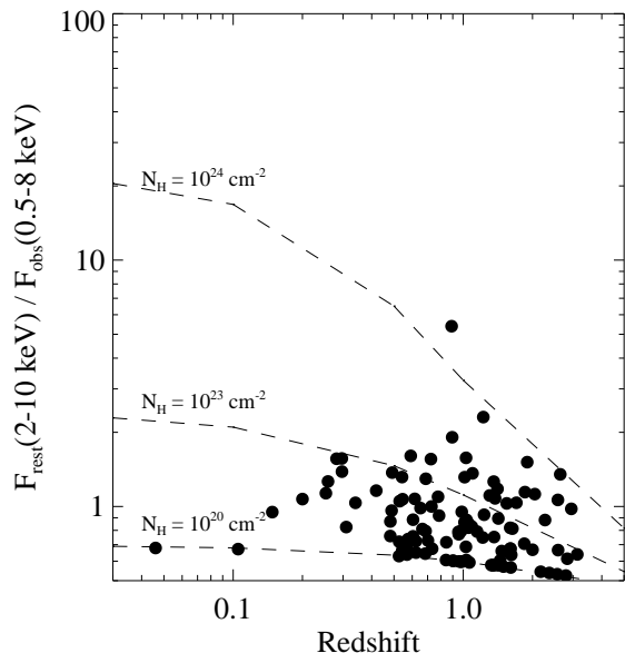
FIG. 5.— The correction from observed 0.5–8 keV flux to rest-frame 2–10 keV flux as a function of redshift for the X-ray-selected AGNs.
