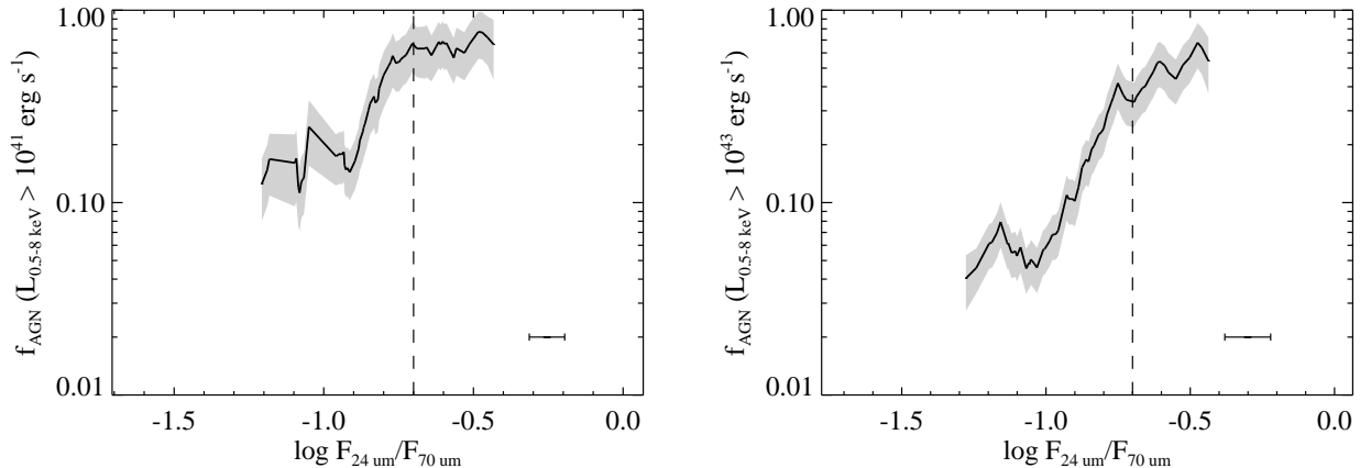
FIG. 10.— The AGN fraction as a function of the mid-infrared color for AGNs with L_{0.5-8.0 \text{ keV}} \geq 10^{41} \text{ erg s}^{-1} (left) and L_{0.5-8.0 \text{ keV}} \geq 10^{43} \text{ erg s}^{-1} (right). The vertical, dashed line denotes \log(F_{24}/F_{70}) \approx -0.7 . A sliding bin containing a minimum of 10 AGNs was used, the mean width of which is indicated in the lower right-hand corner. Variations in the fraction on scales smaller than this bin width are not significant. The shaded region indicates the 1\text{-}\sigma errors.
