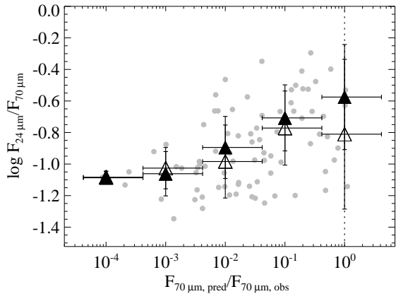
FIG. 8.— The observed mid-infrared color versus the ratio of (observed-frame) predicted-to-observed 70 \mu\text{m} flux for the AGNs in the sample with z < 1.5 . The filled points show the mean values (calculated using the non-logarithmic values of the colors) of subsamples of objects in bins with widths indicated by the horizontal error bars. The open points show the median values for the same bins. Vertical error bars indicate the standard deviation of the colors in each bin.
