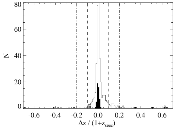
FIG. 1.— Histograms of \Delta z / (1 + z_{\text{spec}}) , where \Delta z = z_{\text{spec}} - z_{\text{phot}} for all 70 \mu\text{m} sources with spectroscopic redshifts ( open region ) and for AGNs only ( filled region ). Vertical lines denote \Delta z / (1 + z_{\text{spec}}) = \pm 0.1 and \Delta z / (1 + z_{\text{spec}}) = \pm 0.2 .
