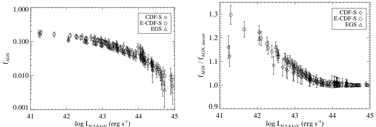
FIG. 9.— Left : The AGN fraction corrected for the Tozzi et al. (2006) distribution of column densities ( f_{\text{AGN}} ) as a function of the intrinsic, rest-frame 0.5–8 keV AGN luminosity. Right : The ratio of the corrected-to-uncorrected AGN fraction as a function of the AGN luminosity. The fraction is plotted separately for each field, as indicated by the different symbols (note, however, that the E-CDF-S sources include those of the CDF-S). Errors are calculated following equation (5), but account only for the sampling error (i.e., \sigma_{\text{phys}} = 0 and \sigma_{N_{\text{H}}} = 0 ).
