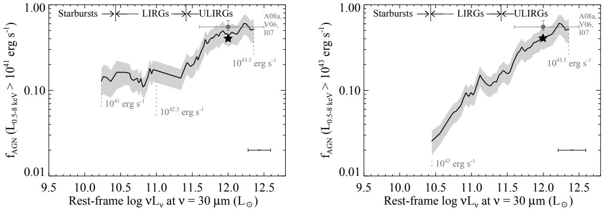
FIG. 11.— The AGN fraction as a function of the rest-frame 30\ \mu\text{m} luminosity for AGNs with L_{0.5-8.0\ \text{keV}} \geq 10^{41}\ \text{erg s}^{-1} (left) and L_{0.5-8.0\ \text{keV}} \geq 10^{43}\ \text{erg s}^{-1} (right). The divisions between starbursts, LIRGs, and ULIRGs were calculated using the starburst models of Chary & Elbaz (2001) by adopting a rest-frame luminosity range for LIRGs of 10^{11}\ L_{\odot} < L_{\text{IR}} < 10^{12}\ L_{\odot} and for ULIRGs of L_{\text{IR}} > 10^{12}\ L_{\odot} . The approximate AGN fraction for local ULIRGs (Imanishi et al. 2007; Veilleux 2006; Alexander et al. 2008a) is indicated by the circle and error bars, with the fraction of such systems found by Alexander et al. (2008a) with L_{2-10\ \text{keV}} \geq 10^{43}\ \text{erg s}^{-1} indicated by the star symbol. The minimum AGN luminosity ( L_{0.5-8.0\ \text{keV}} ) in a number of bins is also indicated. The 1\text{-}\sigma errors and mean bin size are indicated as in Figure 10.
