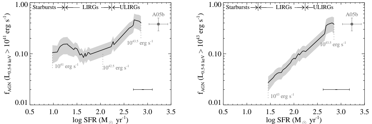
FIG. 12.— The AGN fraction as a function of SFR for AGNs with L_{0.5-8.0\ \text{keV}} \geq 10^{41}\ \text{erg s}^{-1} (left) and L_{0.5-8.0\ \text{keV}} \geq 10^{43}\ \text{erg s}^{-1} (right). The approximate fraction for z \approx 2 submillimeter galaxies (Alexander et al. 2005b) is indicated. The minimum AGN luminosity ( L_{0.5-8.0\ \text{keV}} ) in a number of bins is also indicated. The 1\text{-}\sigma errors and mean bin size are indicated as in Figure 10.
