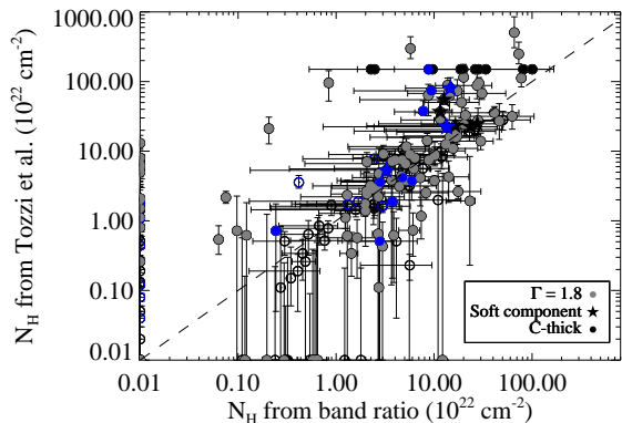
FIG. 4.— Comparison of N_{\text{H}} values from Tozzi et al. (2006) and from our analysis for X-ray-selected AGNs in the CDF-S. The source classification from Tozzi et al. (2006) is indicated by symbol type, and 70\ \mu\text{m} sources are indicated in blue. Sources with N_{\text{H}} < 10^{20}\ \text{cm}^{-2} are set to N_{\text{H}} = 10^{20}\ \text{cm}^{-2} for plotting purposes. A total of 11 sources have this value for both N_{\text{H}} estimates and appear as a single point in the lower left-hand corner.
