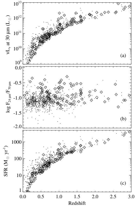
FIG. 2.— The distributions of rest-frame 30 \mu\text{m} luminosity (a), mid-infrared color (b), and star formation rate (c) of the 70 \mu\text{m} sample as a function of redshift. AGNs (selected in §2.6) are indicated by diamonds. AGNs with net 70 \mu\text{m} flux densities that fall below S/N = 3 (after the contribution from the AGN is subtracted) have been removed from the lower panel (a total of 21 sources; see §3.3 for details).
