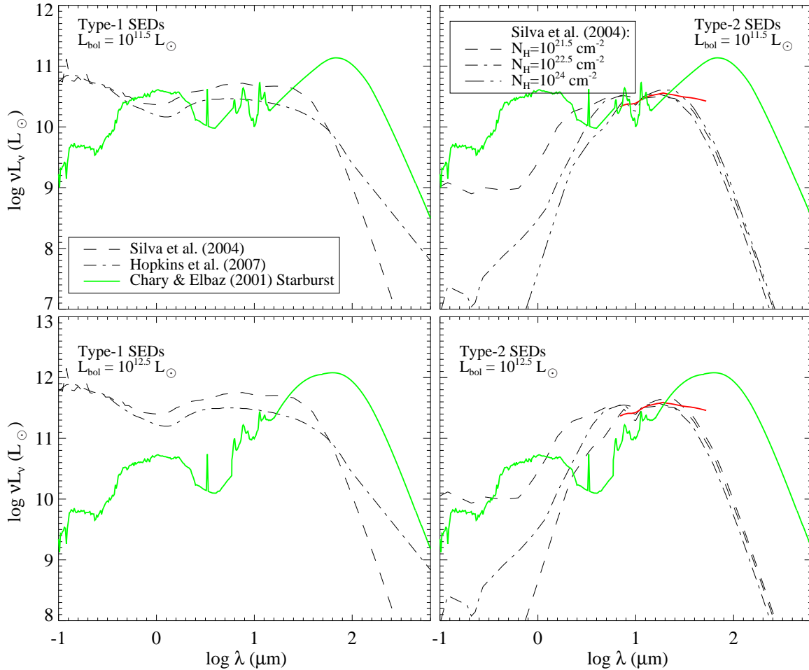
FIG. 6.— Comparison of various AGN SED models (denoted by dashed or dashed-dotted lines). The type-1 AGN models of Silva et al. (2004) and Hopkins et al. (2007) are shown in the left panels, and type-2 AGN models of Silva et al. (2004) with range of intrinsic column densities are shown in the right panels. Also shown (in red) is the average SED from the BAT AGN sample (see §3.2 for details). For comparison, the solid green line shows a starburst SED from Chary & Elbaz (2001) with a SFR chosen such that the 24 \mu\text{m} luminosity approximately matches that of the AGN SEDs.
