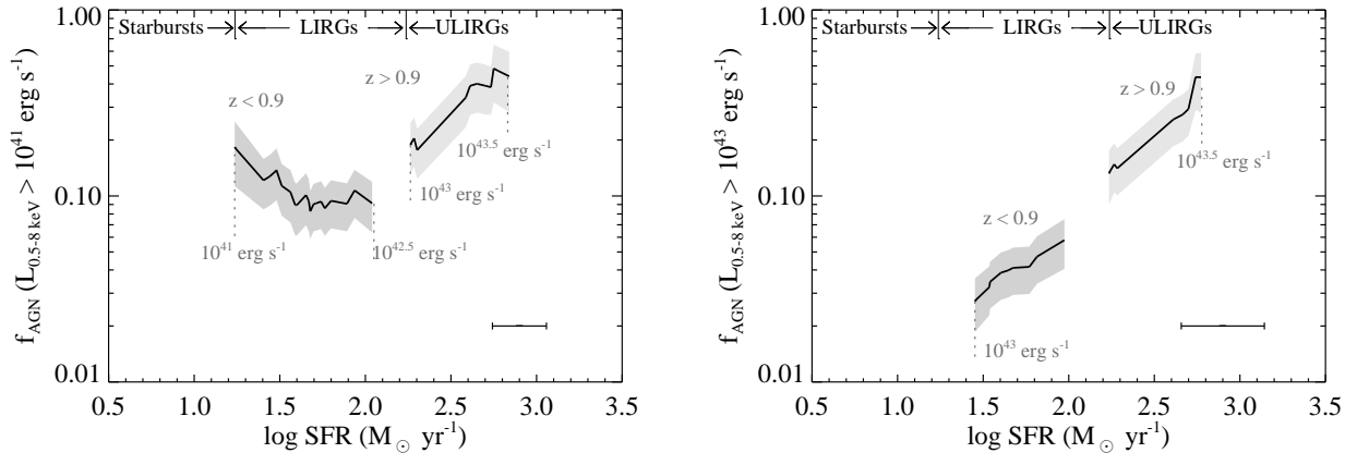
FIG. 13.— The same as Figure 12 but for two subsamples: sources with z < 0.9 (dark gray) and those with z > 0.9 (light gray).
