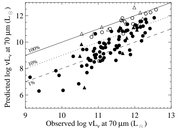
FIG. 7.— Comparison of the AGN’s predicted observed-frame 70 \mu\text{m} luminosity to the observed 70 \mu\text{m} luminosity using the models of Silva et al. (2004) for non-type-1 AGNs (circles) and the models of Hopkins et al. (2007) for type-1 AGNs (triangles). Open symbols denote systems that have a net S/N < 3 after subtracting the estimated contribution from the AGN (see text for details). The solid line denotes equality, and the dashed and dotted lines indicate an AGN contribution to the observed 70 \mu\text{m} luminosity of 1% and 10%, respectively.
