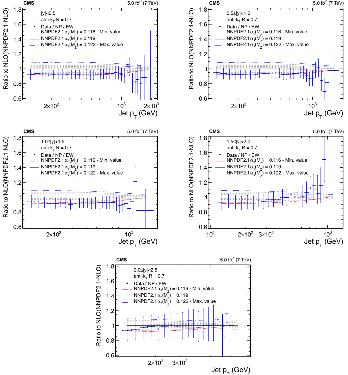
Figure 8: Ratio of the inclusive jet cross section to theoretical predictions using the NNPDF2.1-NLO PDF set for the five rapidity bins, where the \alpha_s(M_Z) value is varied in the range 0.116–0.122 in steps of 0.001. The error bars correspond to the total uncertainty.
