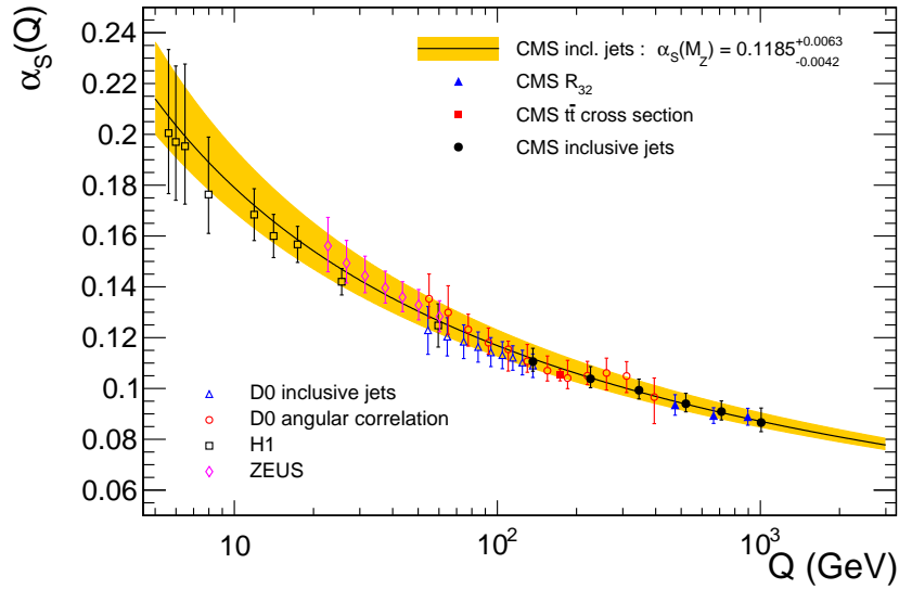
Figure 10: The strong coupling \alpha_s(Q) (full line) and its total uncertainty (band) as determined in this analysis using a two-loop solution to the RGE as a function of the momentum transfer Q = p_T . The extractions of \alpha_s(Q) in six separate ranges of Q as presented in Table 5 are shown together with results from the H1 [58, 59], ZEUS [60], and D0 [52, 53] experiments at the HERA and Tevatron colliders. Other recent CMS measurements [55, 56] are displayed as well. The uncertainties represented by error bars are subject to correlations.
