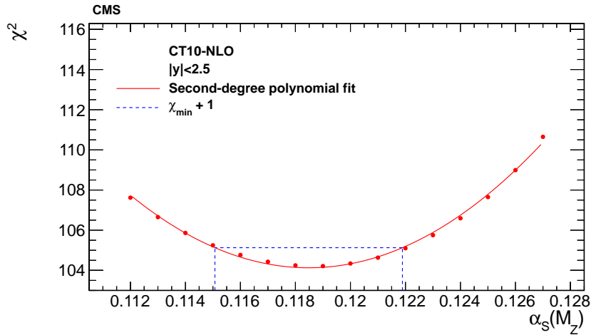
Figure 9: The \chi^2 minimisation with respect to \alpha_S(M_Z) using the CT10-NLO PDF set and data from all rapidity bins. The experimental uncertainty is obtained from the \alpha_S(M_Z) values for which \chi^2 is increased by one with respect to the minimum value, indicated by the dashed line. The curve corresponds to a second-degree polynomial fit through the available \chi^2 points.
