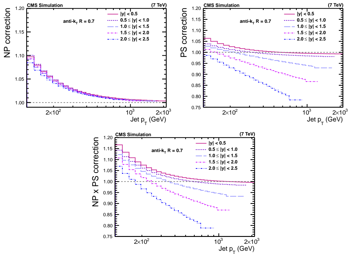
Figure 4: NP correction (top left) obtained from the envelope of the predictions of PYTHIA6 tune Z2, HERWIG++ tune 2.3, and POWHEG + PYTHIA6 with the tunes P11 and Z2*, PS correction (top right) obtained from the average of the predictions of POWHEG + PYTHIA6 tune Z2* with scale factor variation, and combined correction (bottom), defined as the product of the NP and PS correction, for the five regions in |y| .
