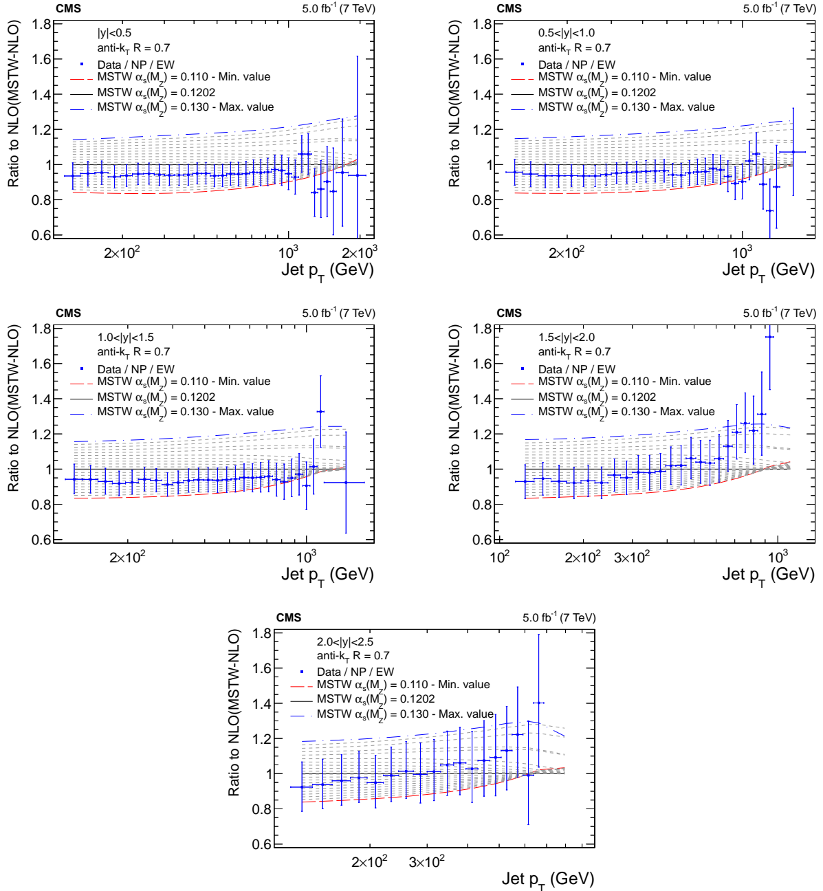
Figure 7: Ratio of the inclusive jet cross section to theoretical predictions using the MSTW2008-NLO PDF set for the five rapidity bins, where the \alpha_s(M_Z) value is varied in the range 0.110–0.130 in steps of 0.001. The error bars correspond to the total uncertainty.
