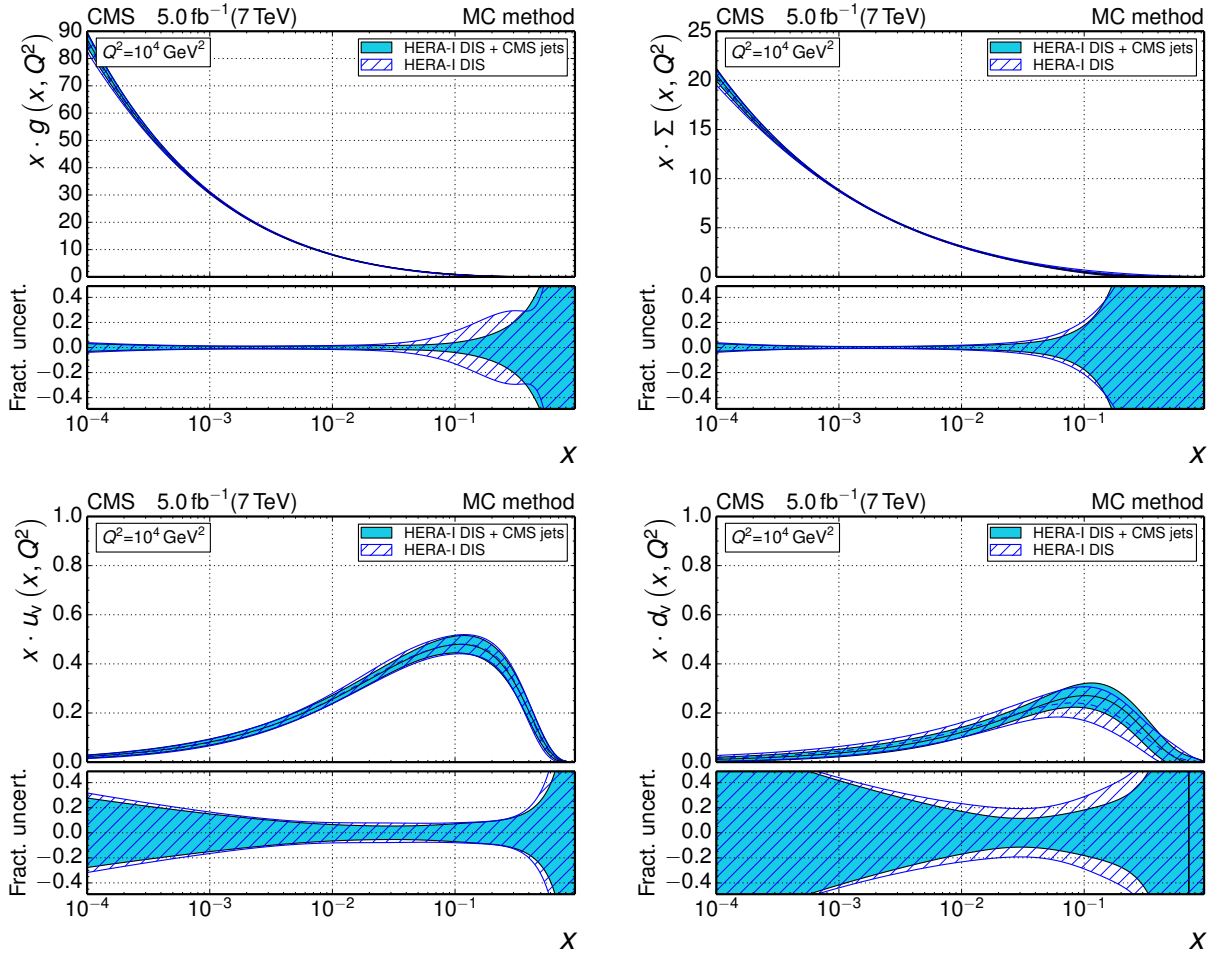
Figure 16: The gluon (top left), sea quark (top right), u valence quark (bottom left), and d valence quark (bottom right) PDFs as a function of x as derived from HERA-I inclusive DIS data alone (dashed line) and in combination with CMS inclusive jet data (full line). The PDFs are determined employing the MC method with data-derived regularisation. The PDFs are evolved to Q^2 = 10^4 GeV ^2 . Only the total uncertainty in the PDFs is shown (hatched and solid bands).
