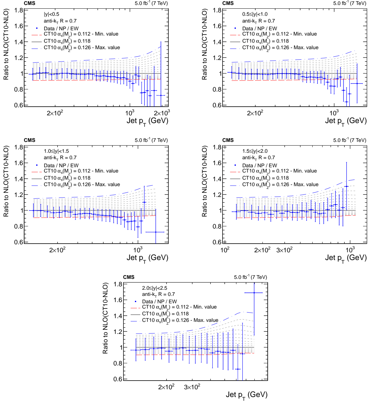
Figure 6: Ratio of the inclusive jet cross section to theoretical predictions using the CT10-NLO PDF set for the five rapidity bins, where the \alpha_s(M_Z) value is varied in the range 0.112–0.126 in steps of 0.001. The error bars correspond to the total uncertainty.
