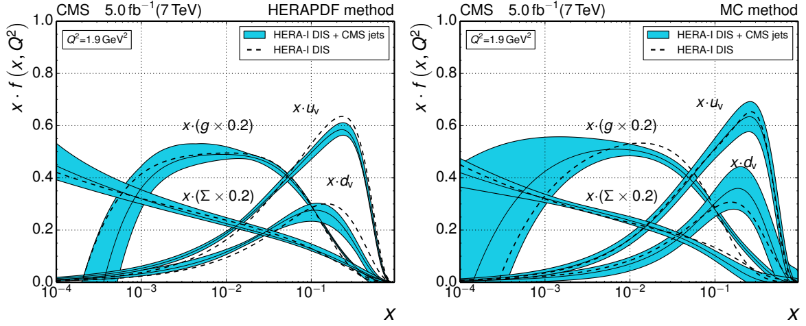
Figure 17: Overview of the gluon, sea, u valence, and d valence PDFs before (dashed line) and after (full line) including the CMS inclusive jet data into the fit. The plots show the PDF fit outcome from the HERAPDF method (left) and from the MC method with data-derived regularisation (right). The PDFs are shown at the starting scale Q^2 = 1.9 \text{ GeV}^2 . The total uncertainty including the CMS inclusive jet data is shown as a band around the central fit result.
