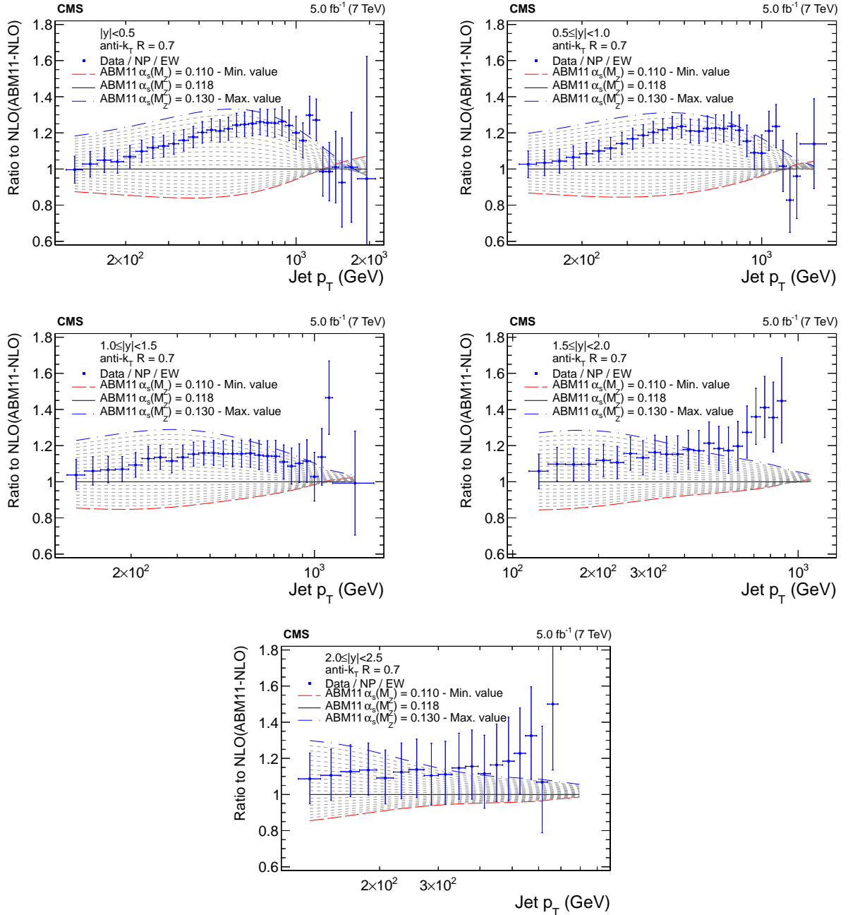
Figure 5: Ratio of the inclusive jet cross section to theoretical predictions using the ABM11-NLO PDF set for the five rapidity bins, where the \alpha_s(M_Z) value is varied in the range 0.110–0.130 in steps of 0.001. The error bars correspond to the total uncertainty.
