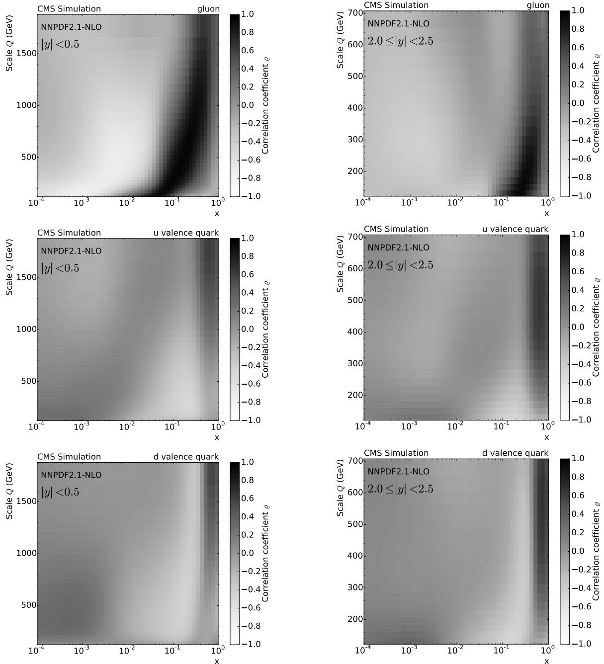
Figure 11: The correlation coefficient between the inclusive jet cross section and the gluon (top row), the u valence quark (middle row), and the d valence quark PDFs (bottom row), as a function of the momentum fraction x of the proton and the energy scale Q of the hard process. The correlation is shown for the central rapidity region |y| < 0.5 (left) and for 2.0 < |y| < 2.5 (right).
