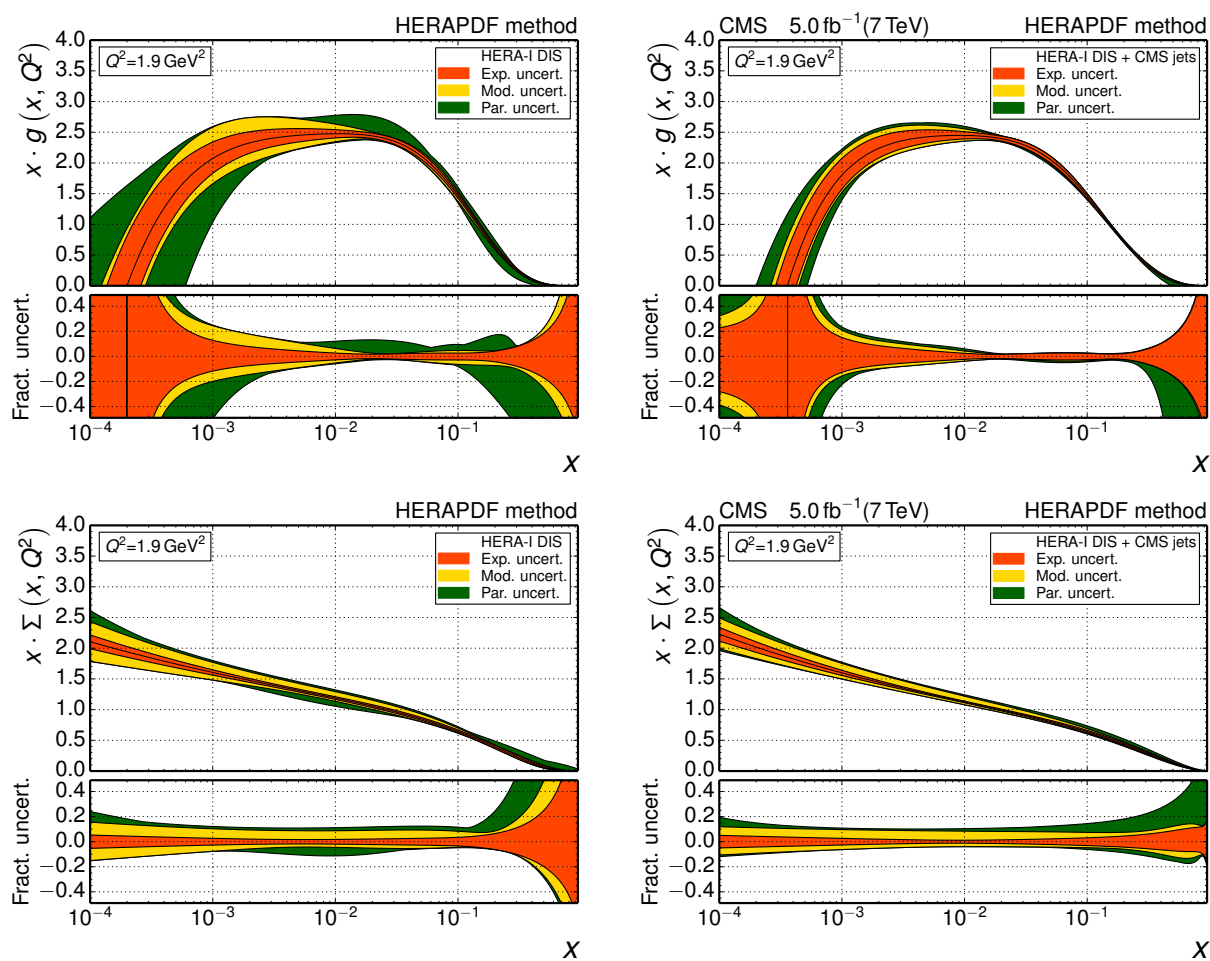
Figure 12: The gluon (top) and sea quark (bottom) PDFs as a function of x as derived from HERA-I inclusive DIS data alone (left) and in combination with CMS inclusive jet data (right). The PDFs are shown at the starting scale Q^2 = 1.9 \text{ GeV}^2 . The experimental (inner band), model (middle band), and parameterization uncertainties (outer band) are successively added quadratically to give the total uncertainty.
