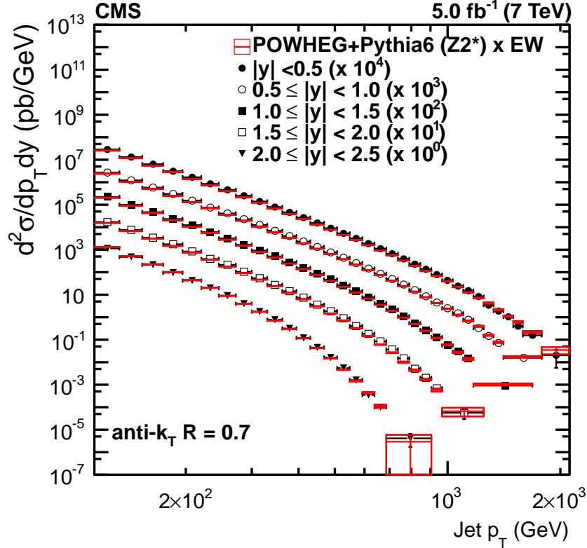
Figure 1: Measured inclusive jet cross section from Ref. [1] compared to the prediction by POWHEG + PYTHIA6 tune Z2* at particle level complemented with electroweak corrections. The boxes indicate the statistical uncertainty of the calculation.
