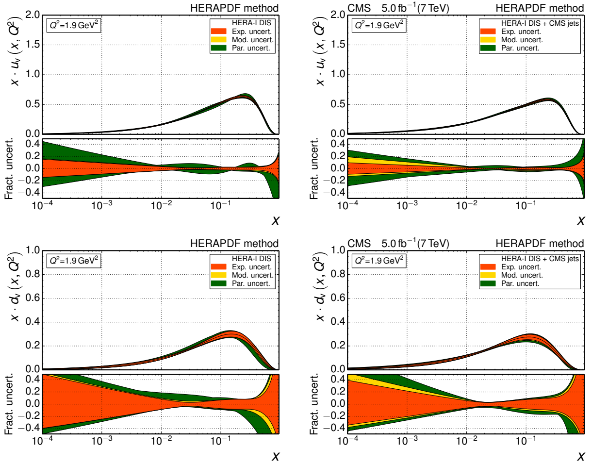
Figure 13: The u valence quark (top) and d valence quark (bottom) PDFs as a function of x as derived from HERA-I inclusive DIS data alone (left) and in combination with CMS inclusive jet data (right). The PDFs are shown at the starting scale Q^2 = 1.9 \text{ GeV}^2 . The experimental (inner band), model (middle band), and parameterization uncertainties (outer band) are successively added quadratically to give the total uncertainty.
