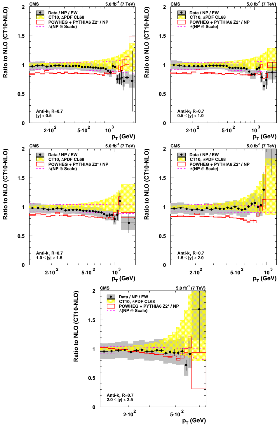
Figure 18: Ratio of data to pQCD at NLO with the CT10-NLO PDF set multiplied by electroweak and NP corrections for the five bins in rapidity together with bands representing the CT10 PDF uncertainty (hatched), and the quadratically added scale and NP uncertainty (dashed lines). In addition, the ratio of the prediction by POWHEG + PYTHIA6 tune Z2* at particle level is shown with boxes indicating the statistical uncertainty. The error bars and the grey boxes correspond to the statistical and systematic uncertainty in the data.
