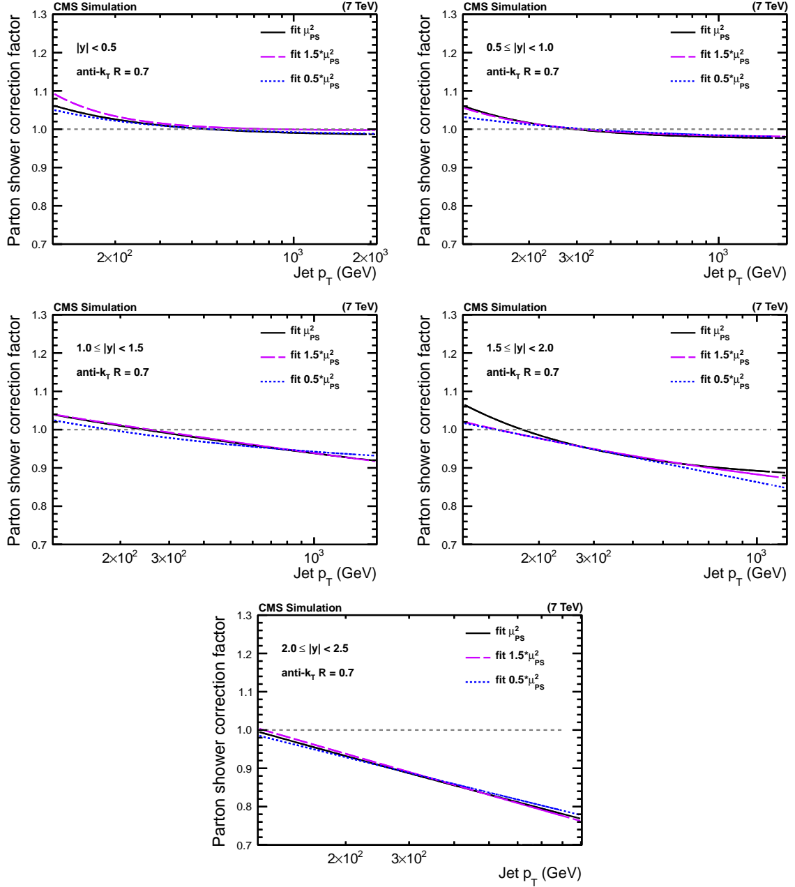
Figure 3: PS corrections for the five regions in |y| obtained from POWHEG using PYTHIA6 for showering for different upper scale limits of the parton shower evolution in PYTHIA6 tune Z2*. The curves parameterize the correction factors as a function of the jet p_T .
