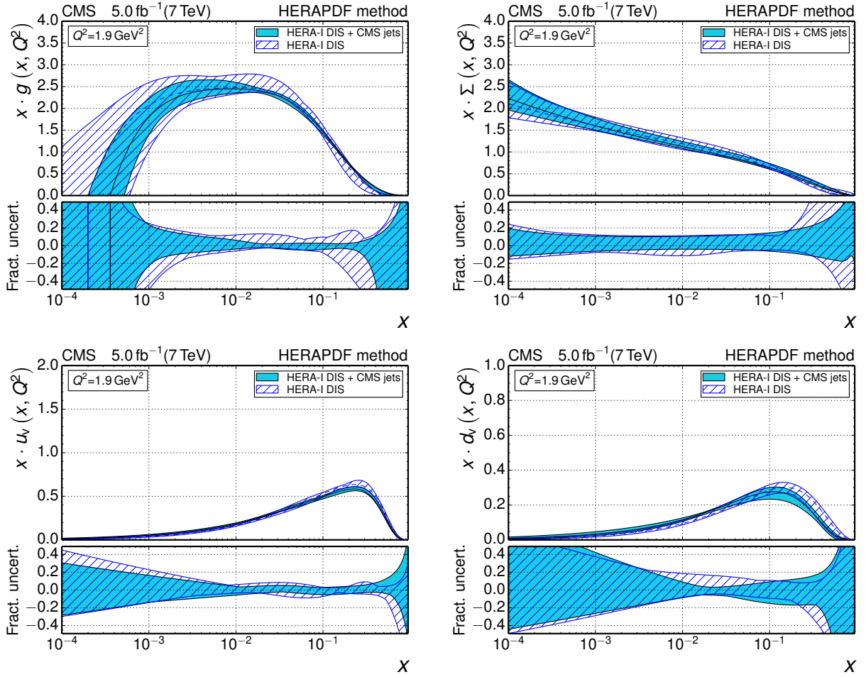
Figure 14: The gluon (top left), sea quark (top right), u valence quark (bottom left), and d valence quark (bottom right) PDFs as a function of x as derived from HERA-I inclusive DIS data alone (dashed line) and in combination with CMS inclusive jet data (full line). The PDFs are determined employing the HERAPDF method with a Q_{\min}^2 = 7.5 \text{ GeV}^2 selection criterion. The PDFs are shown at the starting scale Q^2 = 1.9 \text{ GeV}^2 . Only the total uncertainty in the PDFs is shown (hatched and solid bands).
