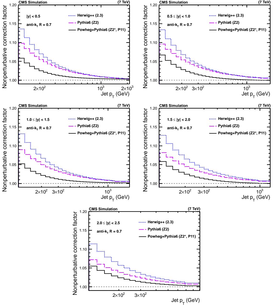
Figure 2: NP corrections for the five regions in |y| as derived in Ref. [1], using PYTHIA6 tune Z2 and HERWIG++ with the default tune of version 2.3, in comparison to corrections obtained from POWHEG using PYTHIA6 for showering with the two underlying event tunes P11 and Z2*.
