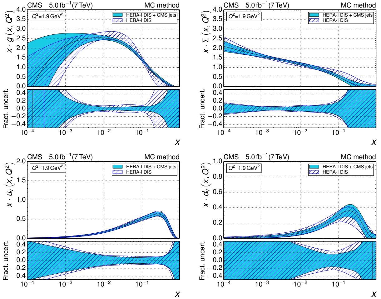
Figure 15: The gluon (top left), sea quark (top right), u valence quark (bottom left), and d valence quark (bottom right) PDFs as a function of x as derived from HERA-I inclusive DIS data alone (dashed line) and in combination with CMS inclusive jet data (full line). The PDFs are determined employing the MC method with data-derived regularisation. The PDFs are shown at the starting scale Q^2 = 1.9 \text{ GeV}^2 . Only the total uncertainty in the PDFs is shown (hatched and solid bands).
