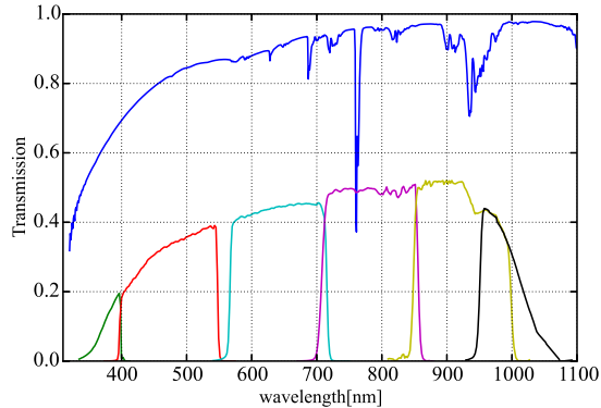
Figure 1. The fiducial atmospheric transmission \phi_{ref}^{atm}(\lambda) at CTIO (upper curve) and the fiducial instrumental throughput \phi_{b,ref}^{inst}(\lambda) of the DES- ugrizY filter bandpasses (lower curves). As DECam only provides a relative throughput measurement, the scale of the lower curves is arbitrary to provide a better visualization.
