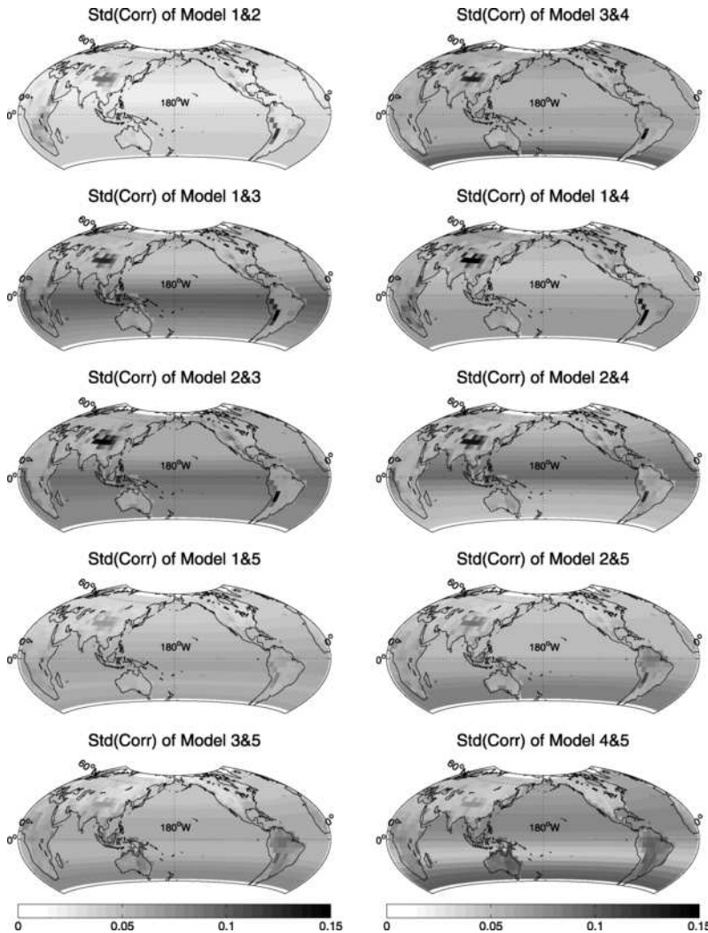
FIG. 5. Standard deviation of the estimated cross-correlation for each pair of climate model errors in Figure 4.
