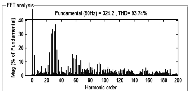
Figure 8. The harmonic spectrum of the output voltage obtained with PWM three intervals strategy.
