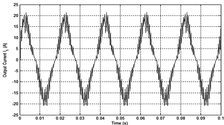
Figure 9. The output current obtained with PWM three intervals strategy – simulation.
