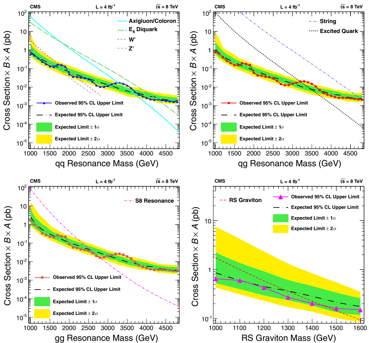
FIG. 2 (color online). Observed upper limits at 95% C.L. on \sigma \times \mathcal{B} \times A for resonances decaying to qq , qg , and gg final state (points and solid lines) compared with the expected limits (dot-dashed dark lines) and their variation at the 1\sigma and 2\sigma levels (shaded bands). Predicted cross sections for various resonance assumptions are shown. The signal shape for the RS model is obtained by weighting the shapes for qq and gg final states according to LO calculations of the relative branching fractions.
