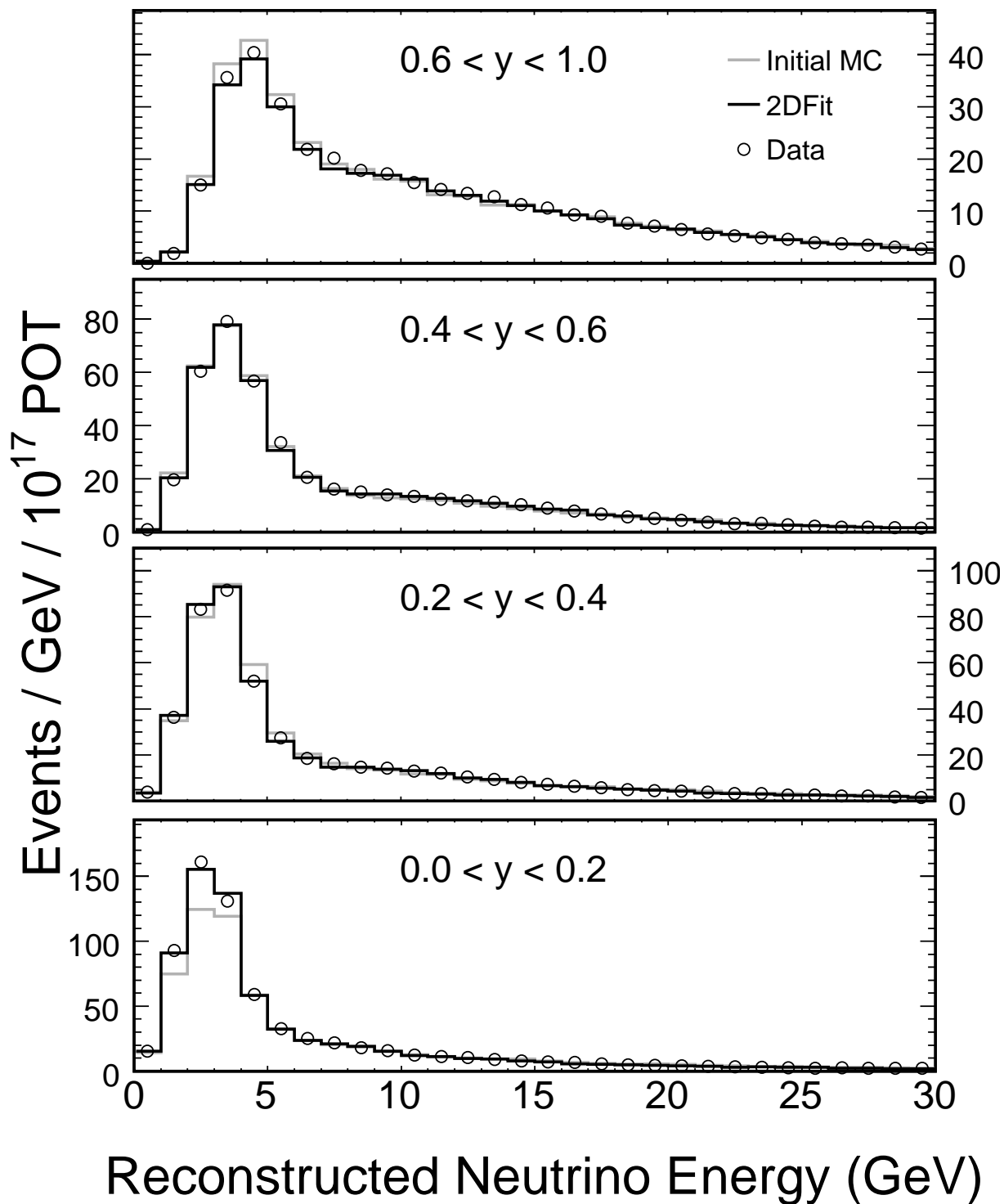
FIG. 33: Near Detector reconstructed neutrino energy spectra collected in the LE10/185kA beam configuration and for different reconstructed y regions. Open circles show the data. The Monte Carlo simulation is shown before and after the tuning procedure performed by the 2DFit technique (Eq. 11). To simplify the presentation we have grouped the eight reconstructed y bins used in the fit into four bins here.
