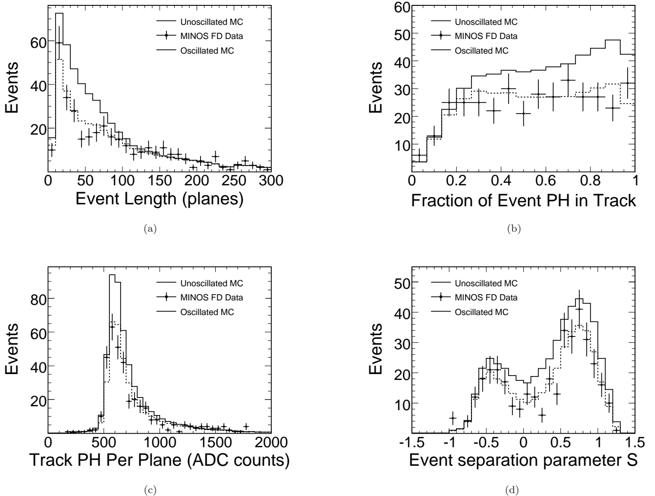
FIG. 24: Distributions of the variables that are used in \nu_\mu charged-current and neutral-current event classification, for Far Detector data and Monte Carlo simulation. The bottom-right plot shows the distribution of the event separation parameter S that is derived from these three PDFs. Oscillations are accounted for according to the mixing parameters extracted from our data (see Sec. VII). These distributions are shown here to illustrate the level of agreement between data and simulation for S and its input variables. They were not examined until the analysis procedure had been fully defined.
