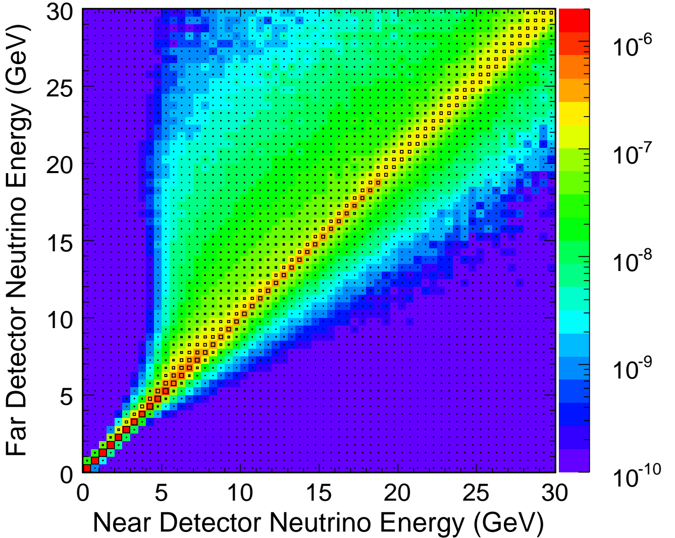
FIG. 31: The joint distribution of neutrino energies observed in the Near and Far Detectors. The contents of each cell represent the mean number of \nu_\mu events expected in the Far Detector for one event in the Near Detector. This distribution may be treated as a matrix, as in Eq. 9, to relate the energy spectra measured in the Near Detector to those in the Far Detector.
