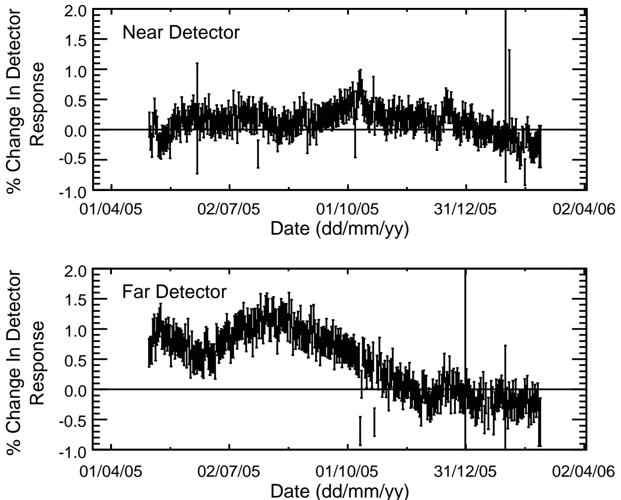
FIG. 19: Variations in the median signal per plane deposited by through-going cosmic-ray muons observed during the data-taking period covered by this paper. The time dependence is largely due to variations in the environmental conditions in the Near and Far Detector halls and aging of the scintillator. The zero point on the ordinate is arbitrary.
