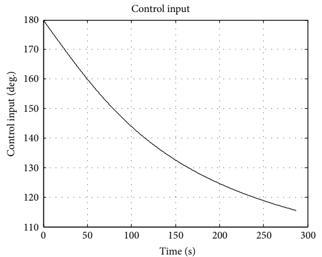
FIGURE 7: The control command for the optimal lunar landing.
