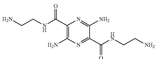
Scheme 1 of Example 4: Chemical structures of pyrazine-based diamino crosslinkers. Structure 2 is also referred to as MP-3142. Structure 3 is also referred to as MP-3192.
