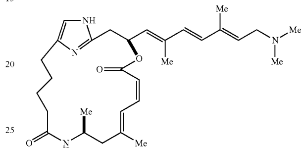
AminoDMDAPatA (imidazole derivative)
