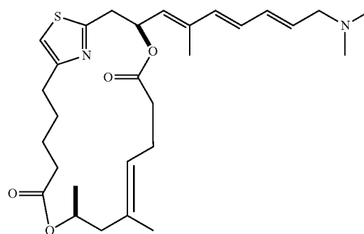
Dihydro desmethyl DMDAPatA
