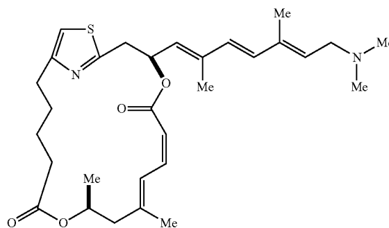
3: Des-methyl, des-amino PatA (DMDAPatA)
