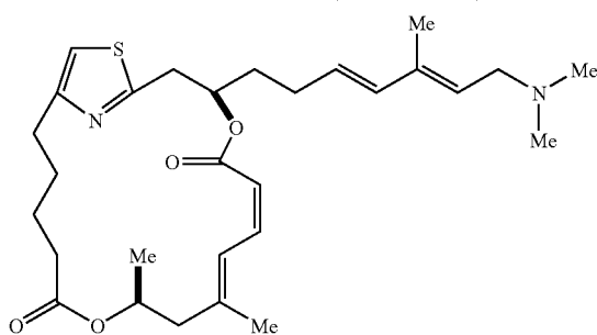
DMDAPatA with unconjugated side chain
