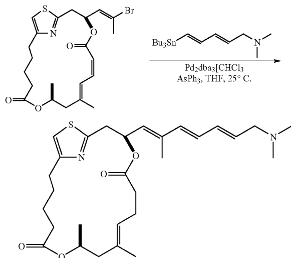
Dihydro desmethyl DMDAPatA
