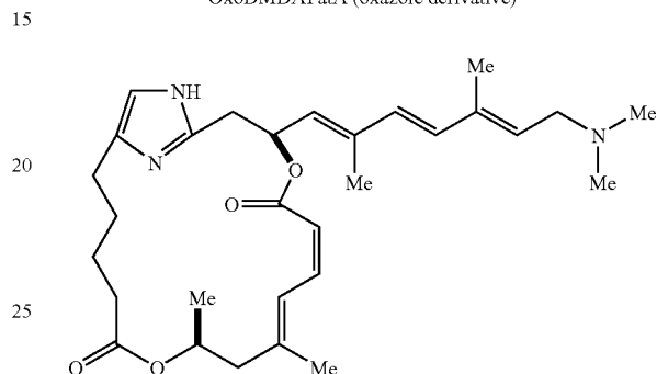
AminoDMDAPatA (imidazole derivative)
