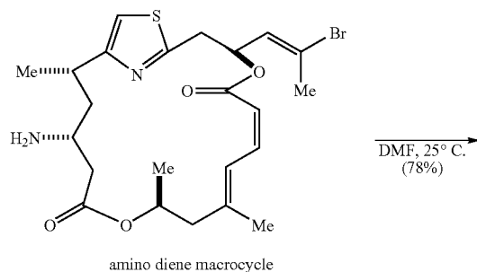
amino diene macrocycle
