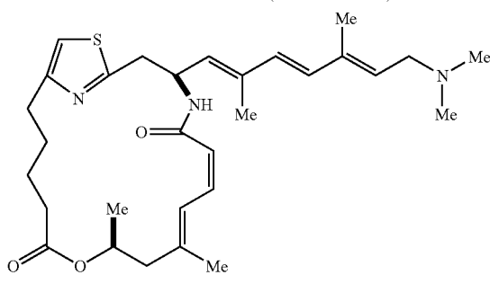
C18-AmidoDMDAPatA (amide derivative)
