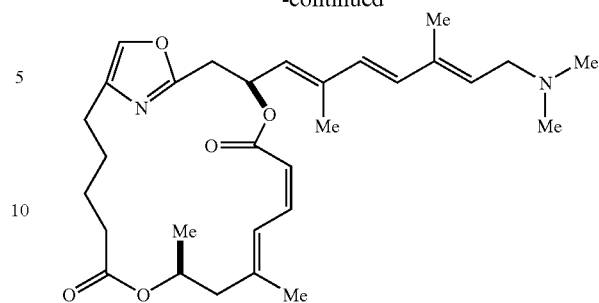
OxoDMDAPatA (oxazole derivative)
