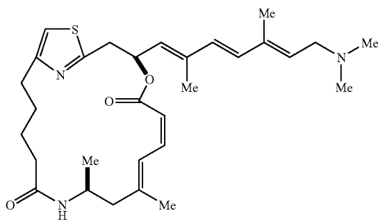
C1-AmidoDMDAPatA (amide derivative)
