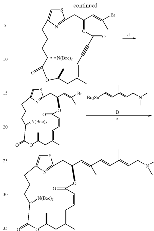
Des-methyl \alpha -amino Pateamine A derivative, 21
