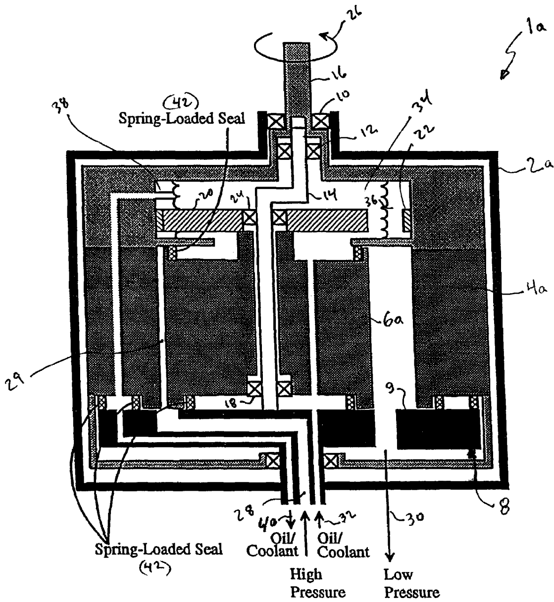
Figure 3 Small-diameter gerotor.
