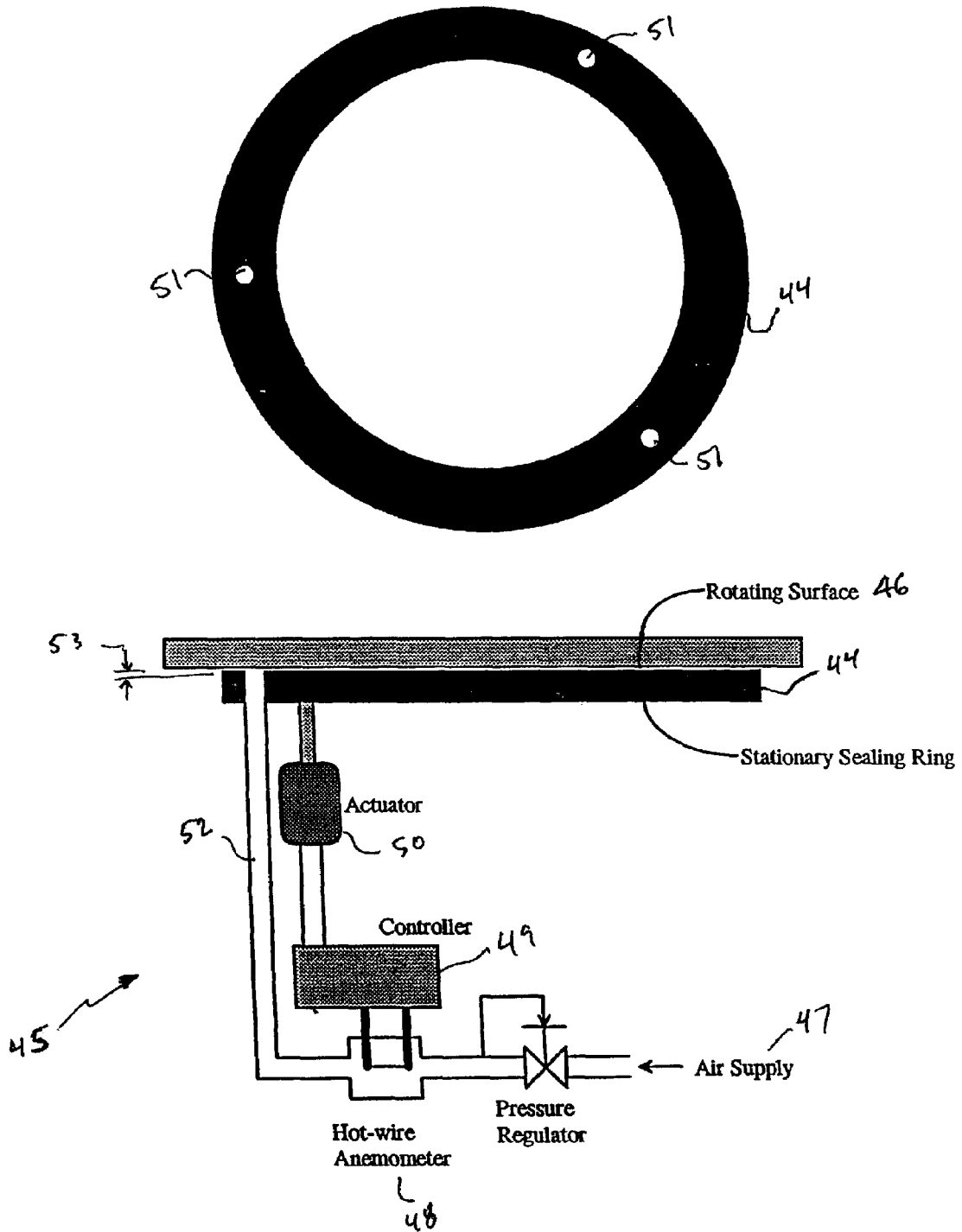
Figure 7 Actuated seal.
