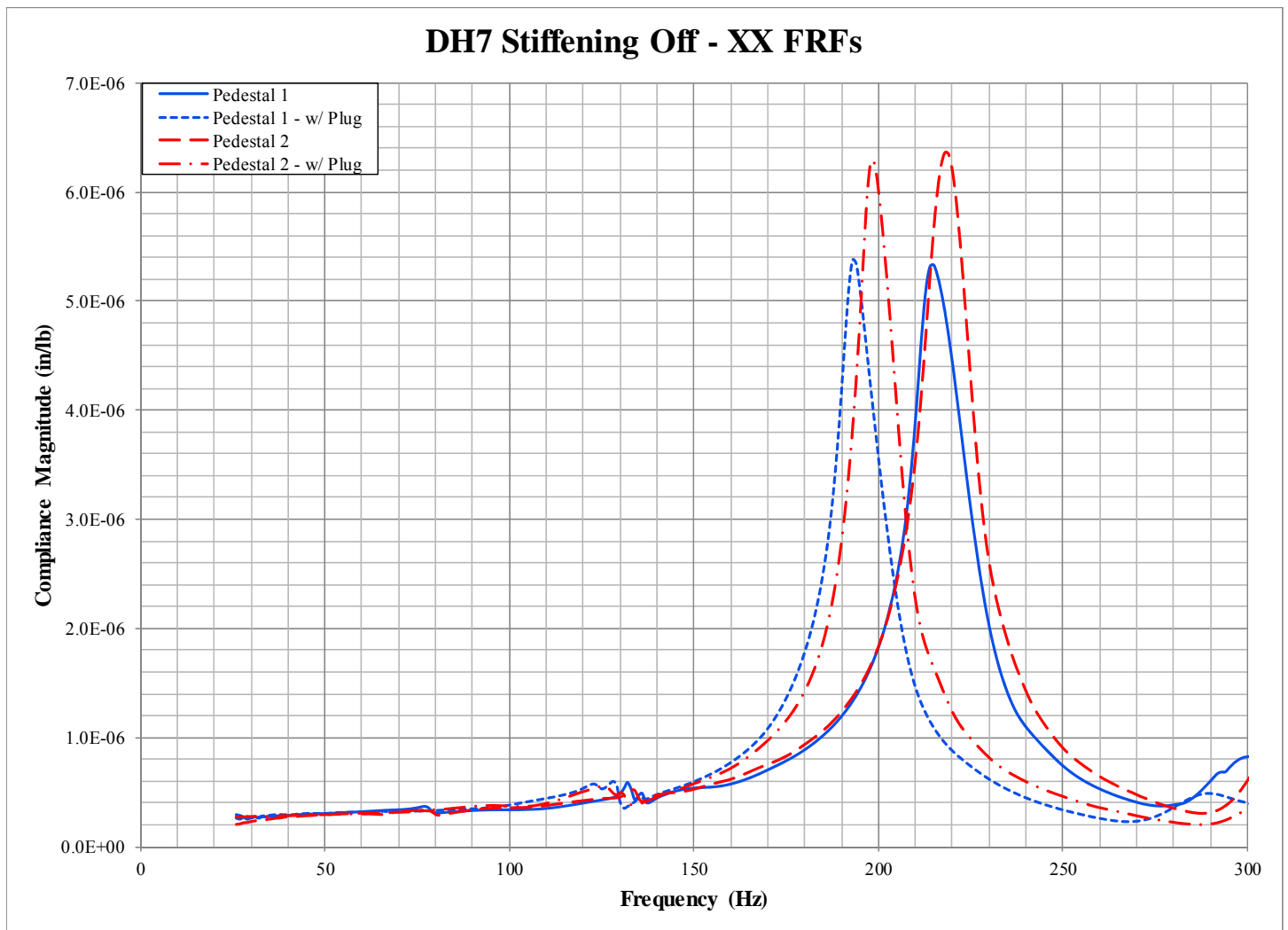
Figure 15: DH7 pedestal response with and without plug (XX, stiffening off)
