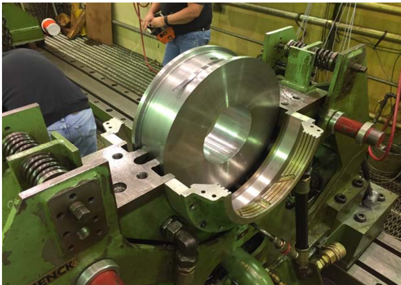
Figure 14: DH7 Pedestal Plug
