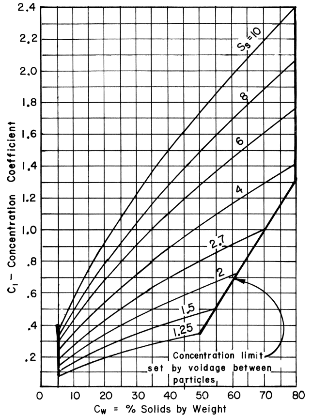
Figure 8. Settling Slurries—Head and Efficiency Correction. Concentration effect.
