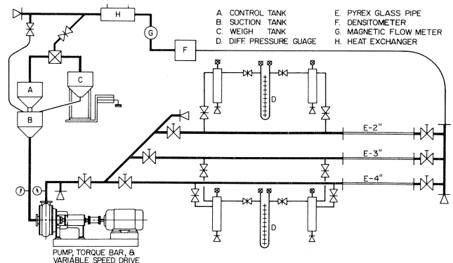
Figure 11. Outline of Slurry Test Facility.
