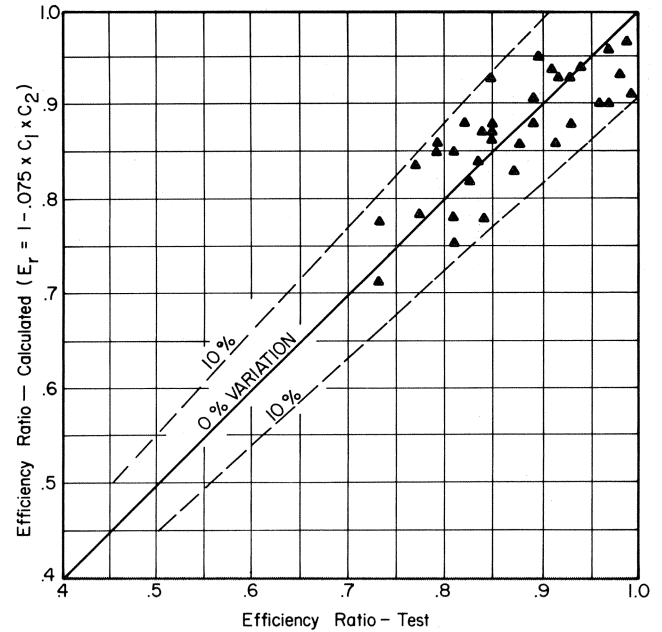
Figure 13. Performance Reduction Error Analysis—Efficiency.
