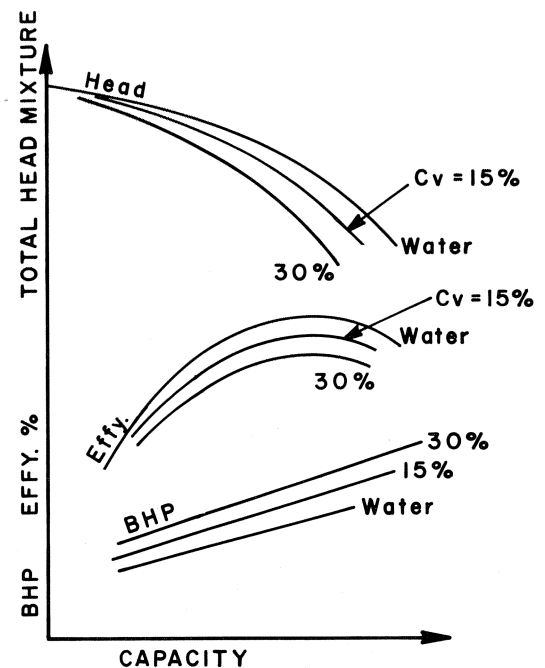
Figure 4. Typical Performance Characteristic Non-Settling Slurries.
