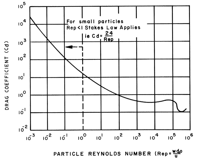
Figure 3. Drag Coefficient Curve for Spherical Particles.
