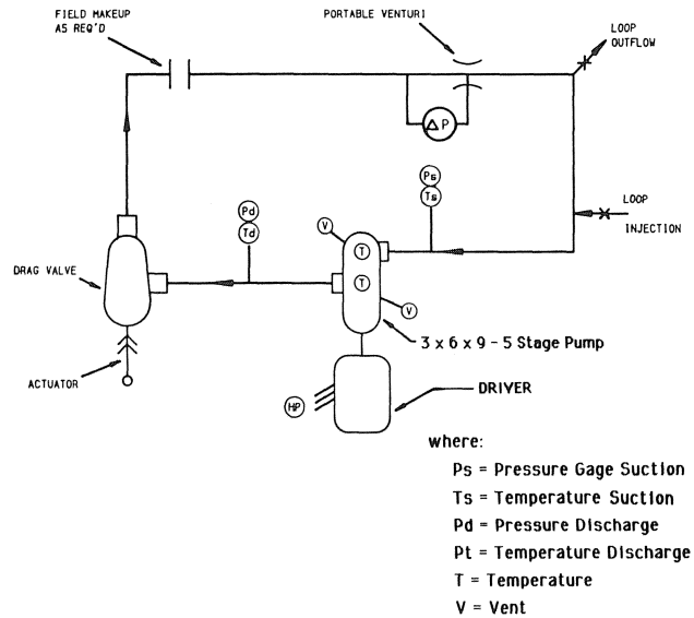
Figure 6. Test Loop Schematic.
