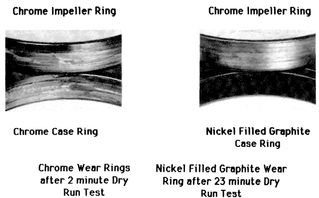
Figure 7. Comparison of Case Wear Rings After Dry Run Test.
