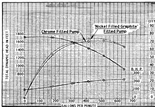
Figure 5. Hydraulic Performance Comparison.
