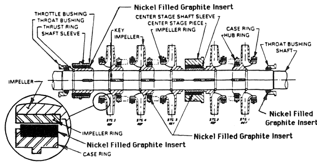
Figure 4. Nickel Filled Graphite Fitted Rotating Element.
