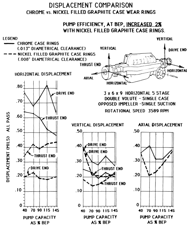
Figure 8. Displacement Comparison.
