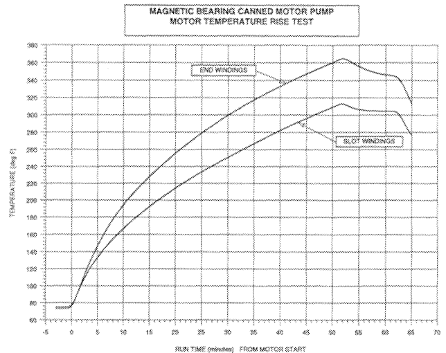
Figure 9. Motor Temperature Rise.
