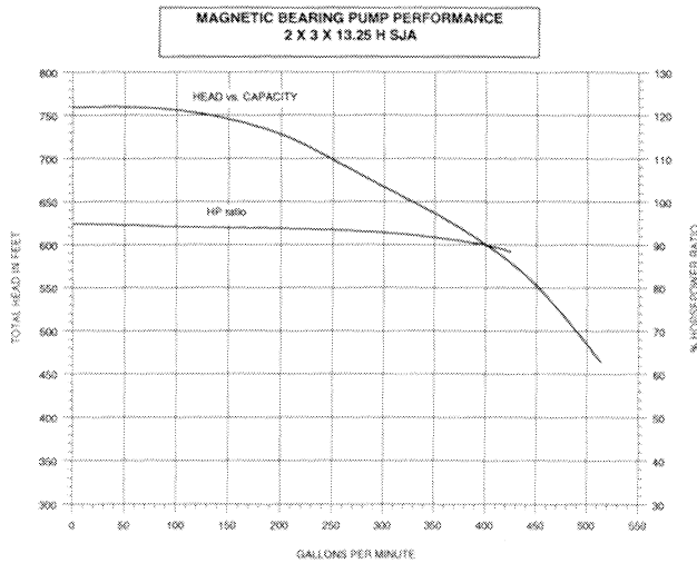
Figure 4. Pump Performance Curve.
