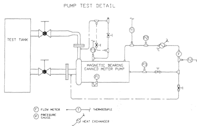
Figure 3. Test Stand Schematic.
