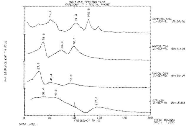
Figure 5. Resonance Plots Using Sweep Generator.
