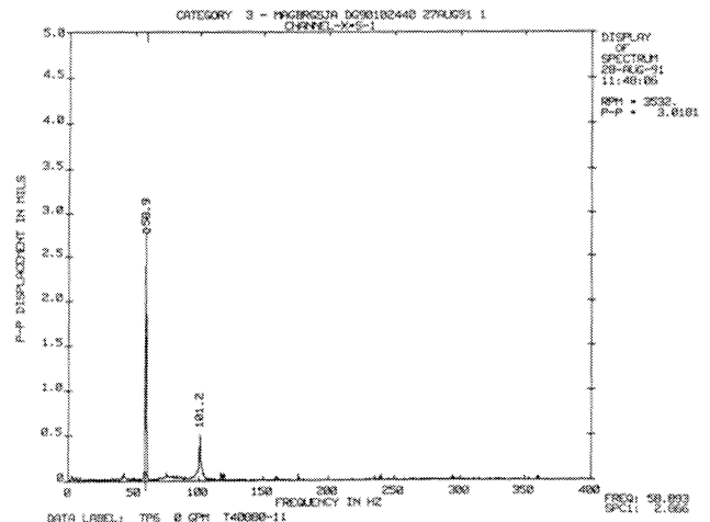
Figure 6. Pump Vibration at Shutoff Flow.
