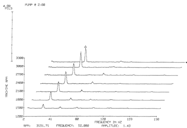
Figure 8. Cascade Plot with Pump Run Using VFD.
