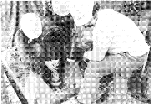
Figure 25. The Cylinder of a Homemade Grout Pump Was Used as a Funnel to Fill the Baseplate.
