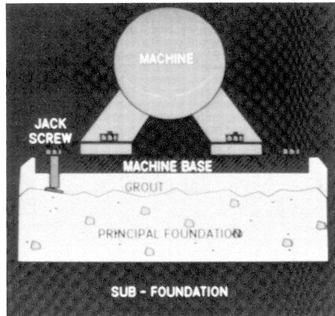
Figure 3. Jack Screws Resting on Circular Disks is the Preferred Method of Pump Baseplate Support Prior to Grouting.
