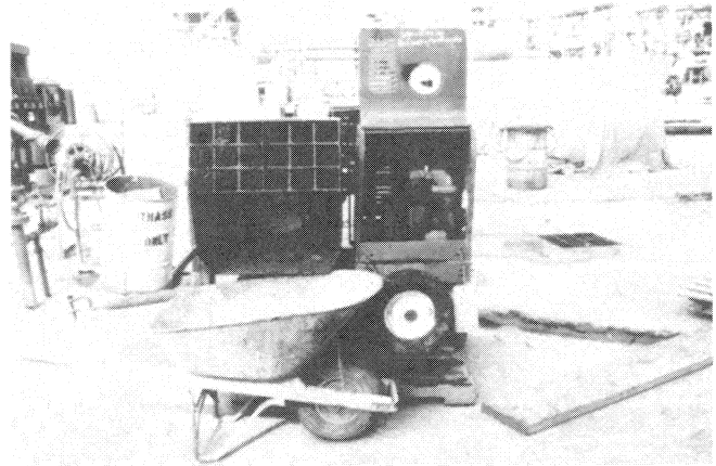
Figure 19. A Second Method of Epoxy Grout Mixing is with a Motorized Mortar Mixer with a Mixer Blade Speed of 15 to 30 RPMs.
