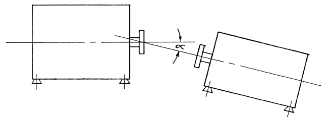
Figure 36. Angular Misalignment.
