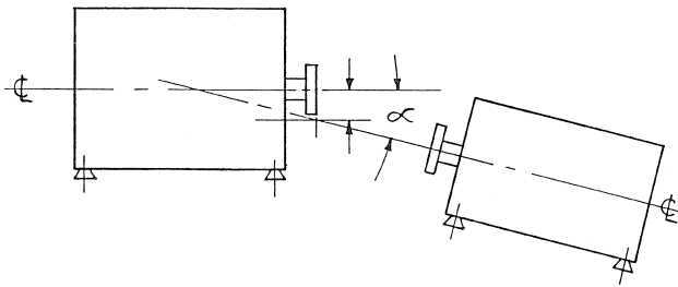
Figure 37. Parallel and Angular Misalignment.
