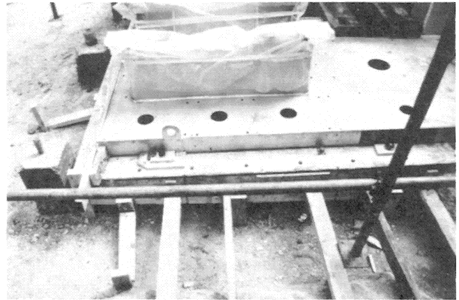
Figure 16. An API Pump Baseplate Formed up for a Single Pour Grout Job. Notice the vented top form attached to the side forms and baseplate flanges.
