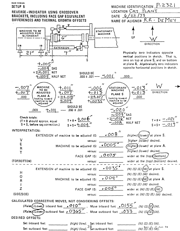
Figure 44. Reverse Indicator Using Crossover Brackets, Including Face Gap Equivalent Differences and Thermal Growth Offsets.
