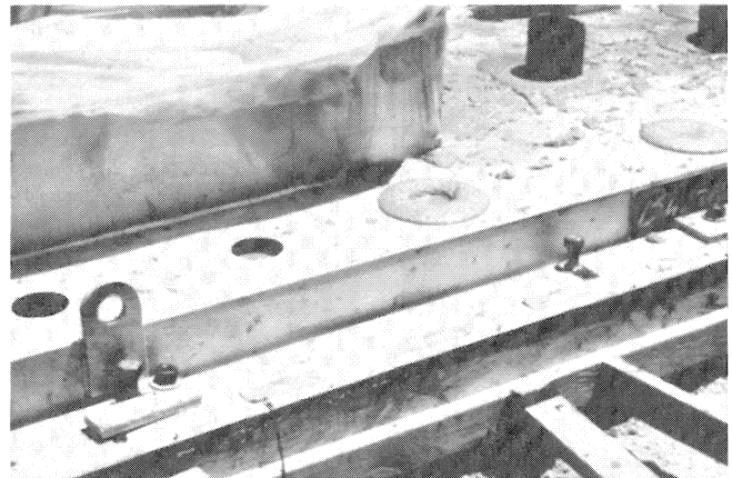
Figure 17. Duct Tape was Used to Stop the Flow of Grout Out Vent Holes as the Baseplate Grouting Continued.
