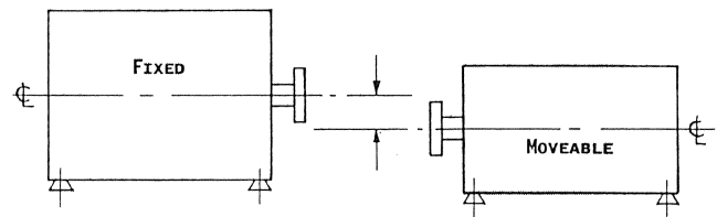
Figure 35. Parallel Misalignment.
