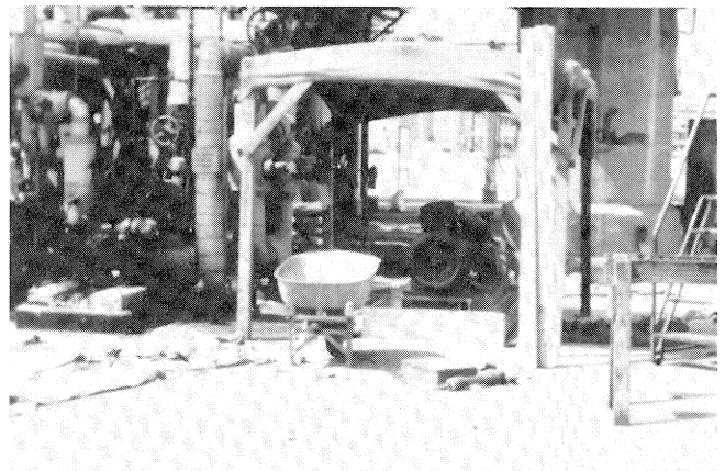
Figure 7. In Hot Weather, Shade the Baseplate/Foundation for 24 Hr Before and 48 Hr after Pouring the Grout. Also protects against rain.
