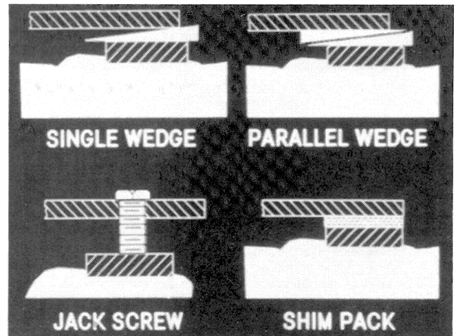
Figure 1. The Four Most Common Methods Used to Level Pump Baseplates Are a Single, Double, or Parallel Wedges, Jack Screws and Shim Pack with Chock.
