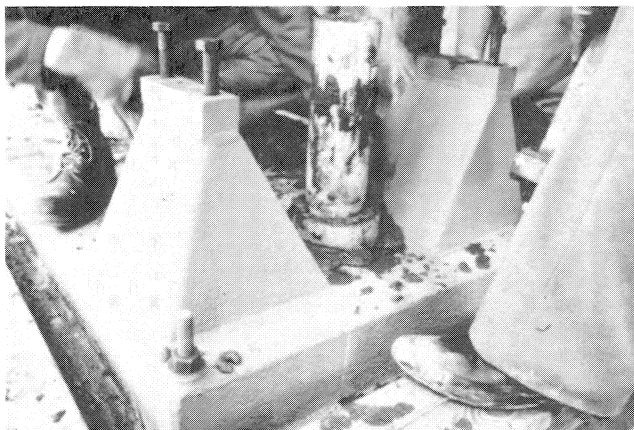
Figure 27. Notice the "Grout Worms" Pressured Out of the Vent Holes Around the Anchor Bolts by the Grout Pump.
