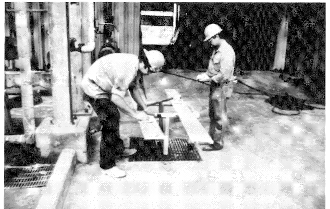
Figure 13. Three Coats of Paste Wax Must be Applied to all Grout Form Surfaces Coming in Contact with the Grout.
