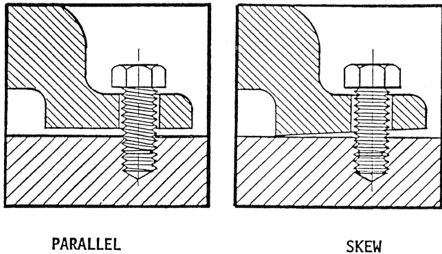
Figure 33. Types of Soft Foot.
