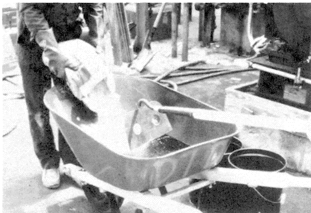
Figure 18. One Method of Epoxy Grout Mixing is by Hand Using a Wheelbarrow and Mortar Hoe. Aggregate is slowly added to the liquid epoxy.
