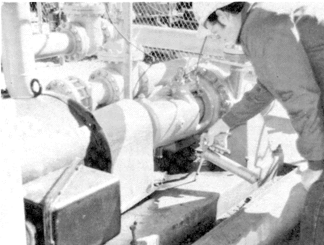
Figure 32. This Machinist Used a Clean Grease Gun to Fill a Void Under the Baseplate with Unfilled Epoxy Grout.
