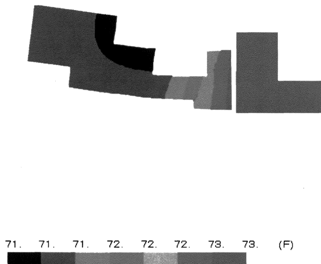
Figure 9. Predicted Face Distortions on Saddleback Shaped Primary Rings.
