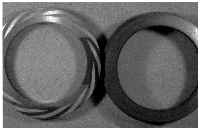
Figure 14. Seal Faces After Start/Stop Testing.
