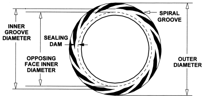
Figure 1. Typical Spiral Groove Sealing Surface.
