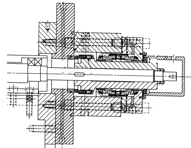
Figure 13. High Pressure Gas Seal Test Rig Arrangement.
