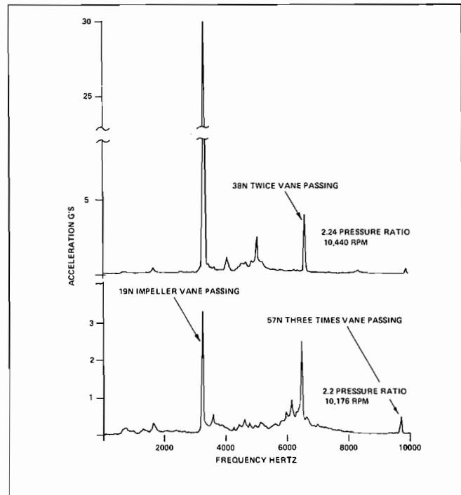
Figure 11. Amplitude Variation of a Centrifugal Compressor Vane Passing Frequency in Response to a Change in Speed and Pressure Ratio.
