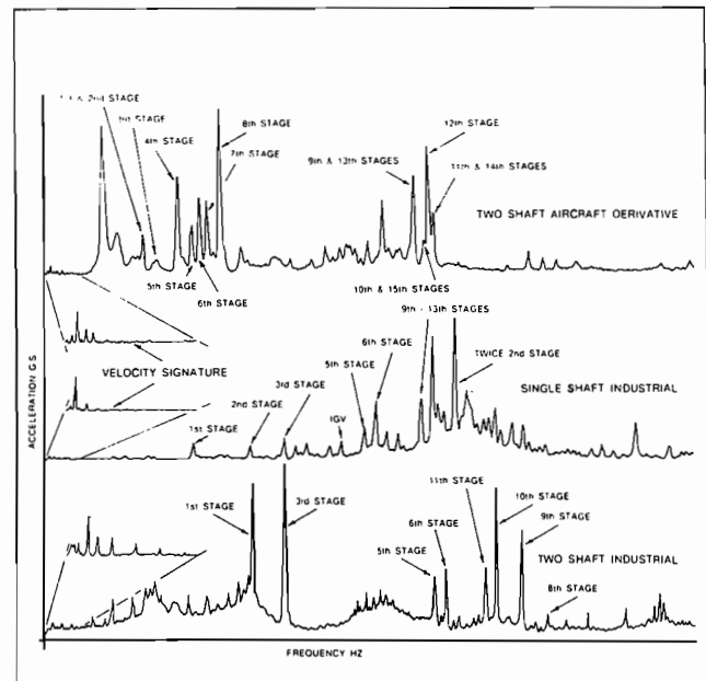
Figure 8. Gas Turbine Casing Acceleration Signatures — Axial Compressor Section.
