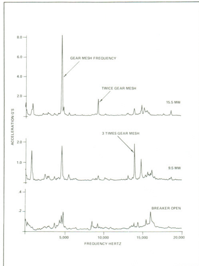
Figure 2. High Frequency Amplitude Variations Corresponding to Changes in Gear Load.
