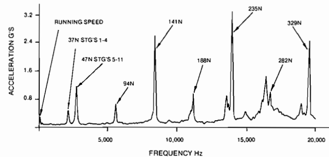
Figure 7. Axial Flow Compressor Casing Acceleration Signature.
