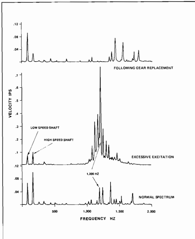
Figure 5. Speed Increasing Gear Casing Acceleration Signatures.
