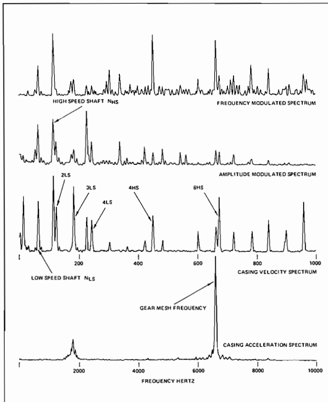
Figure 3. Speed Increasing Gear Casing and Demodulated Signatures.
