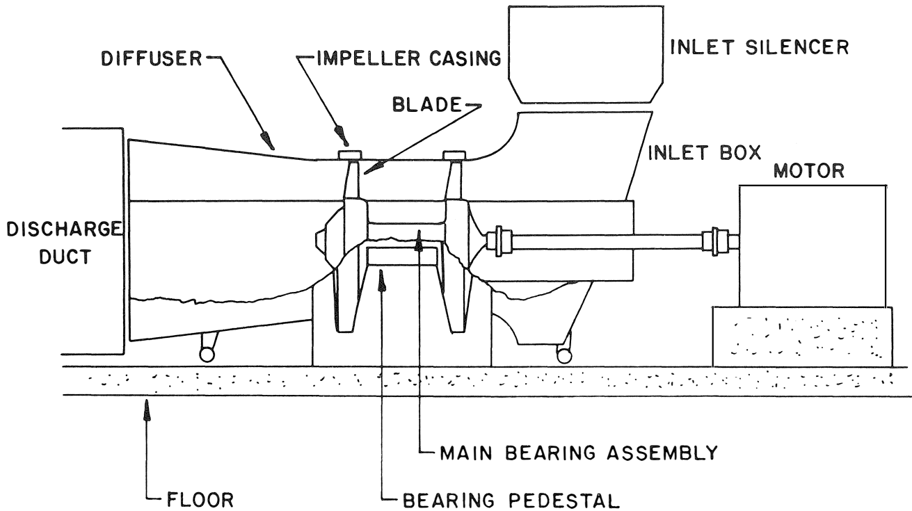
Figure 11. Cutaway View of Two-Stage Axial Fan.
