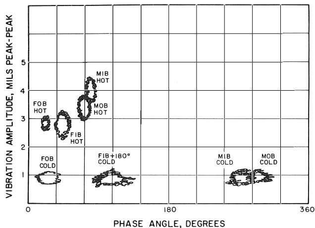
Figure 9. Variation of Motor and Fan Bearing Vibration During Hot and Cold Conditions.
