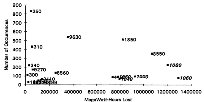
Figure 7. Typical Risk Plot Showing Frequency and Consequence by Cause Code [3].
