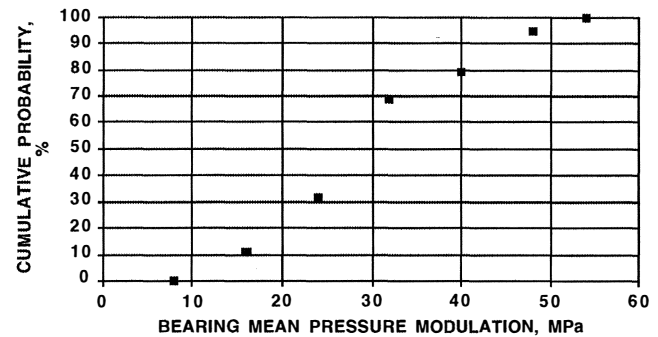
Figure 11. Cumulative Probability of Failure vs Mean Pressure Modulation, Average Fatigue Strength = 29.25 Mpa ± 37 Percent (Extracted from [8]).
