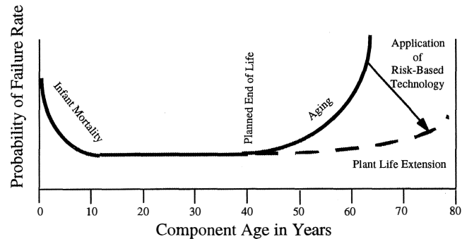
Figure 1. Plant Component Life Cycle.
