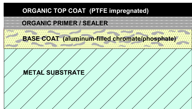
Figure 1. Illustration of Three-Part Construction of Multilayer Composite Coating.
