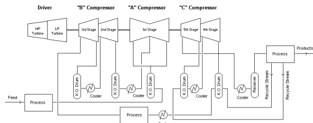
Figure 4. Schematic Diagram of CGC at Corunna Plant. ("C" compressor (fourth/fifth stage) is centrifugal compressor discussed in case study.)
