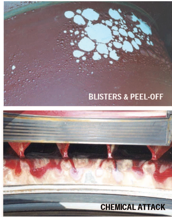
Figure 6. Deterioration of Organic Topcoat of Coating 3P with Benzene Blisters and Chemical Attack from Amine.
