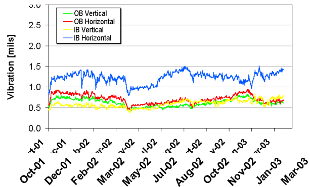
Figure 7. Vibration Trend of "C" Compressor Rotor Coated with Electroless Nickel and Operated from October 2001 to Date.
