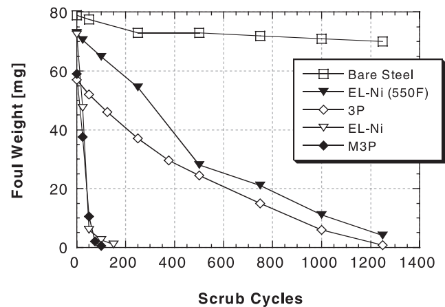
Figure 3. Comparison of Fouling-Release Performance of Bare Steel and Coated Panels.
