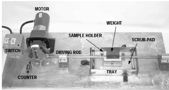
Figure 2. Foulant-Release Test Rig.
