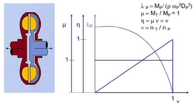
FIGURE 24: HYDRODYNAMIC COUPLING PERFORMANCE MAP
