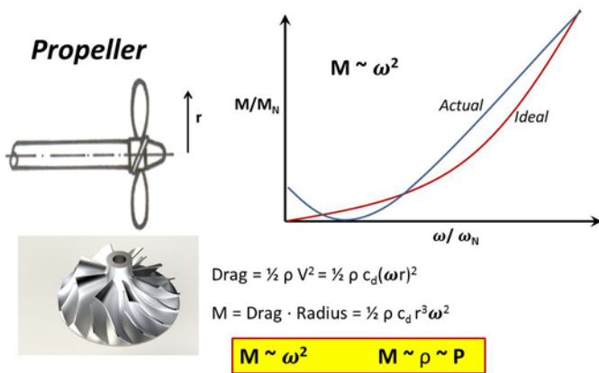
FIGURE 3: FLUID MACHINERY TORQUE TRANSMISSION
