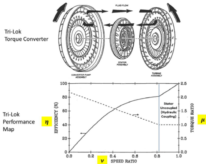
FIGURE 17: AUTOMOTIVE TORQUE CONVERTER EXAMPLE
