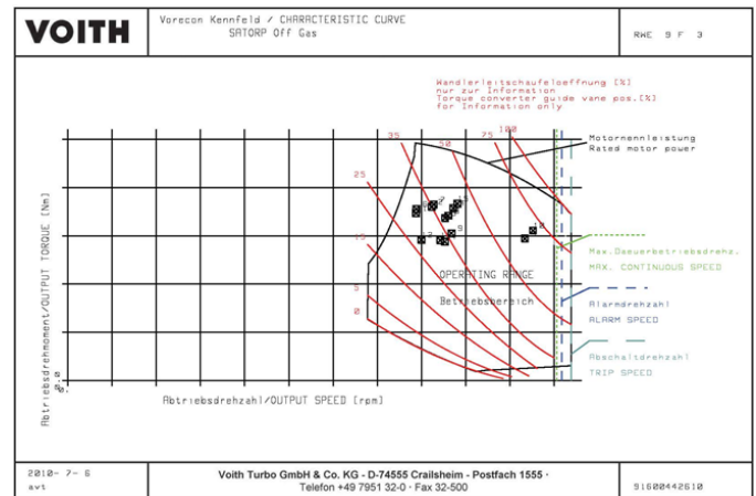
FIGURE 30: VORECON PERFORMANCE MAP TORQUE VERSUS SPEED
