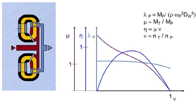
FIGURE 22: FOETTINGER TORQUE CONVERTER PERFORMANCE MAPS
