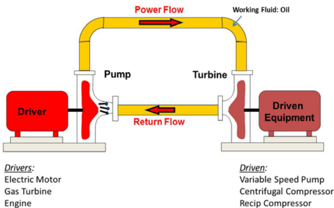
FIGURE 7: BASIC FUNCTION OF HYDRODYNAMIC TRANSMISSION
