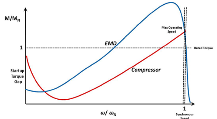
FIGURE 6: ELECTRIC MOTOR WITH CENTRIFUGAL COMPRESSOR TORQUE CURVES (STARTING LIMITED)
