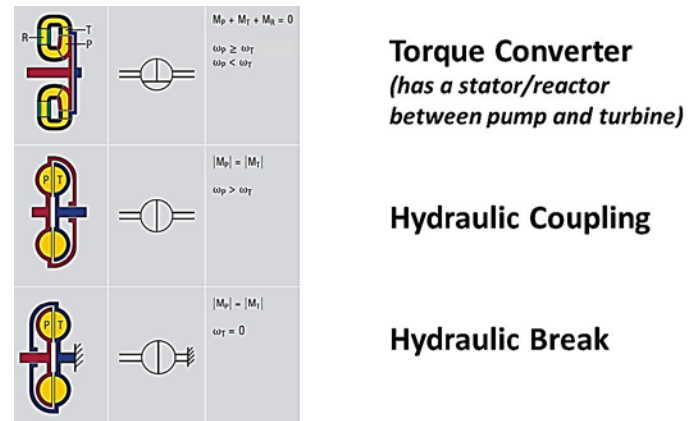
FIGURE 11: TYPES OF HYDRODYNAMIC TRANSMISSIONS
